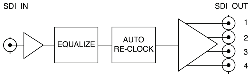
Figure 1. Simplified Block Diagram of SRA-9001 Functions
