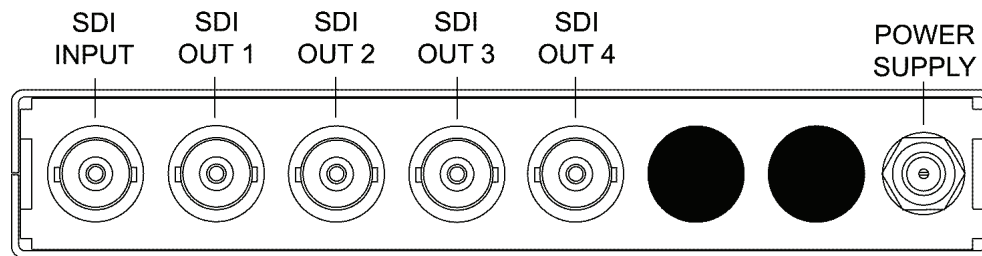
Figure 8. SRA-9001 Rear Connections Configuration
