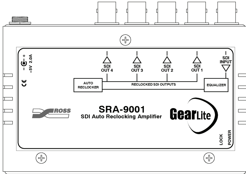
Figure 7. SRA-9001 Cable Connections Indicator Label
