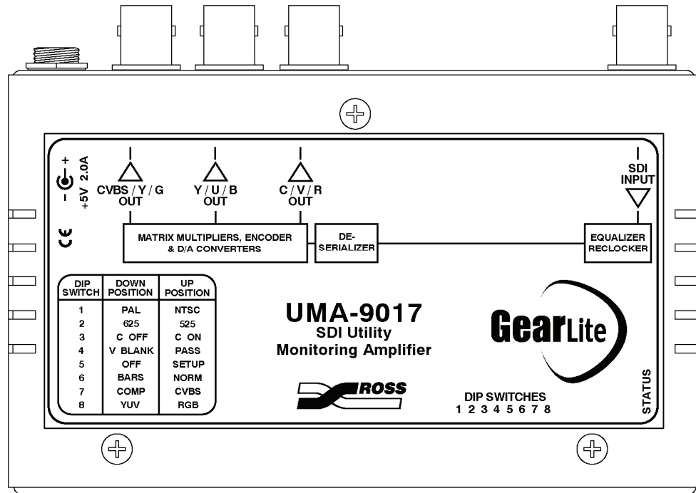
Figure 7. UMA-9017 Cable Connections Indicator Label
