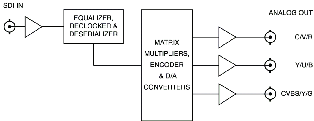
Figure 1. Simplified Block Diagram of UMA-9017 Functions
