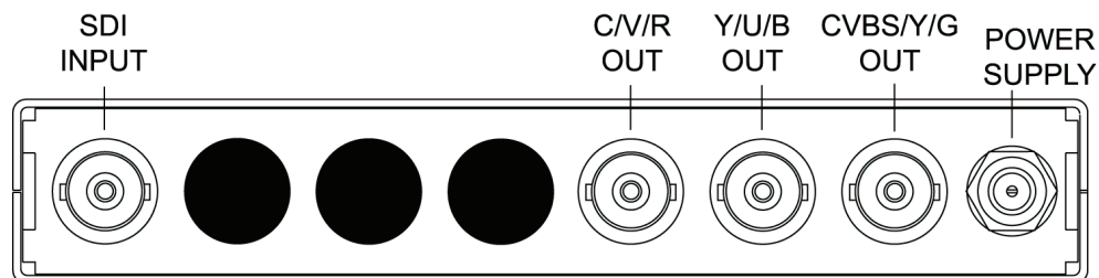
Figure 8. UMA-9017 Rear Connections Configuration
