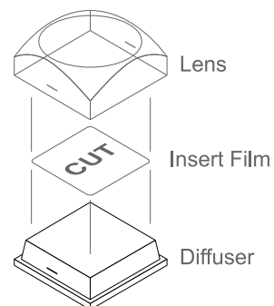
Figure 11: Inserting Film
