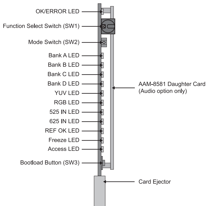
Figure 3.2 ADC-8733A Card-edge Controls
