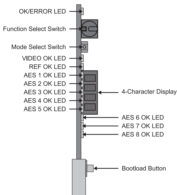
Figure 3.2 DMX-6259-A Card-edge Controls
