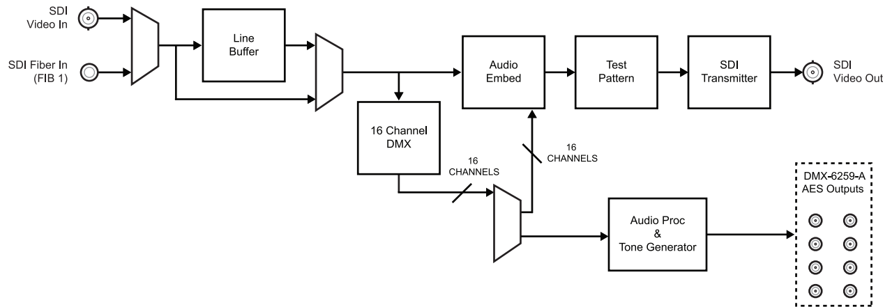
Figure 1.1 DMX-6259-A — Simplified Block Diagram
