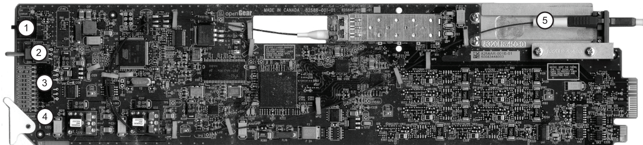
Figure 3.1 DMX-6259-A — Card-edge Components
