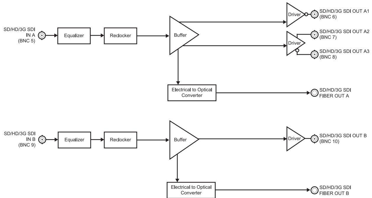
Figure 1.1 FDT-6604 Full Rear Module — Simplified Block Diagram
