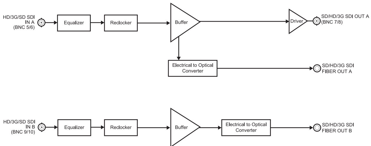
Figure 1.2 FDT-6604 Split Rear Module — Simplified Block Diagram (Single Card only)
