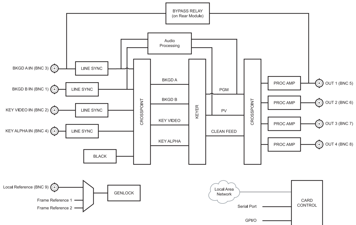
Figure 1.1 Simplified Block Diagram — MDK-111A-Lite
