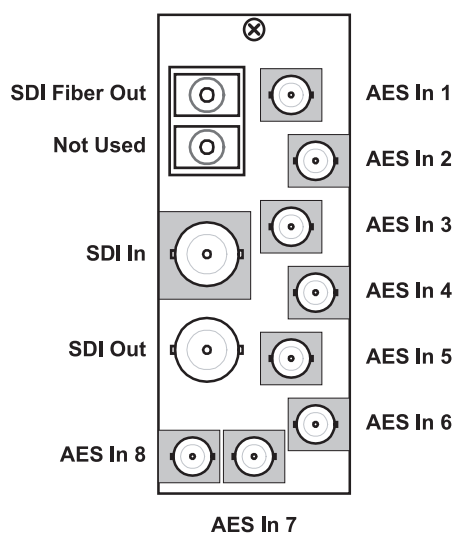
Figure 2.4 Cable Connections for the 8320AR-048A Rear Module
