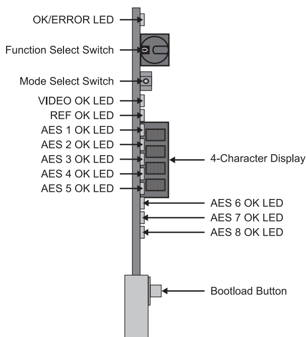
Figure 3.2 MUX-6258-A Card-edge Controls
