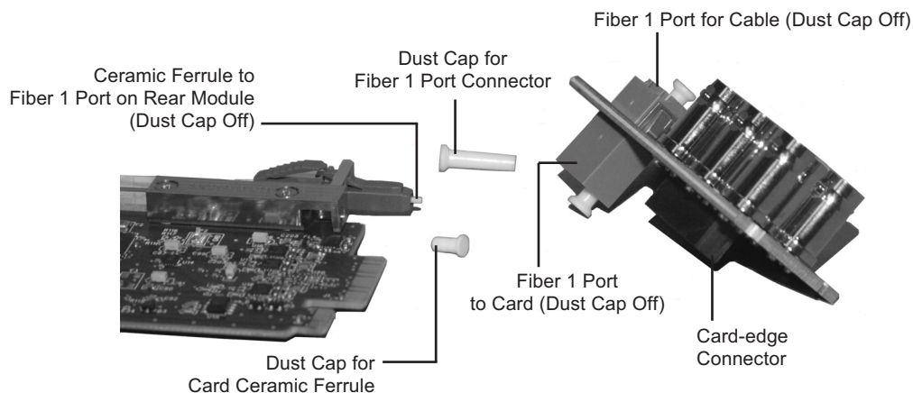
Figure 2.2 Card Connectors with Dust Caps Removed
