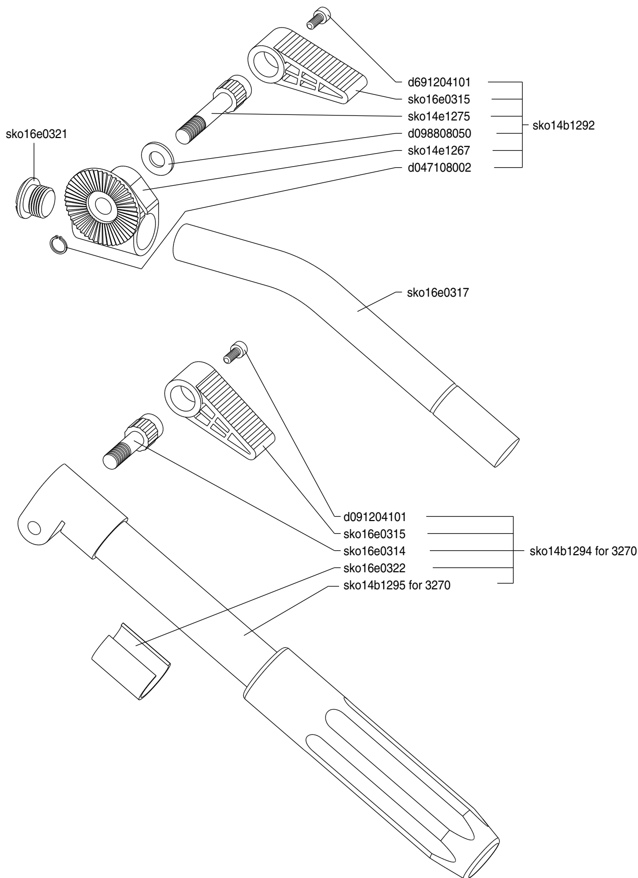
Schwenkarm Plus rechts/right 3270 from January '99 Pan arm Plus
