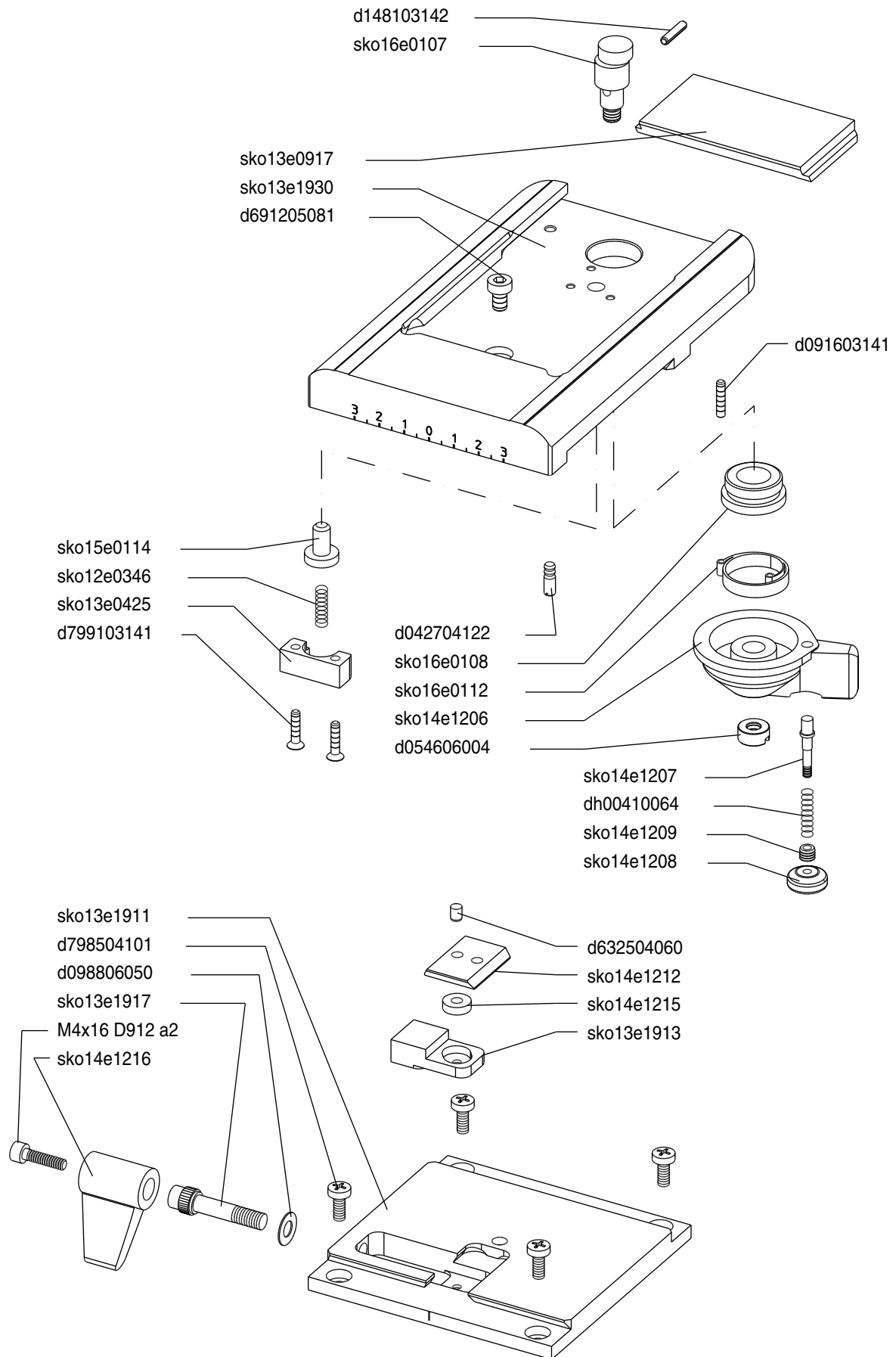
Schnellspannplatte / Grundplatte Quick-release sliding platform / Base plate
