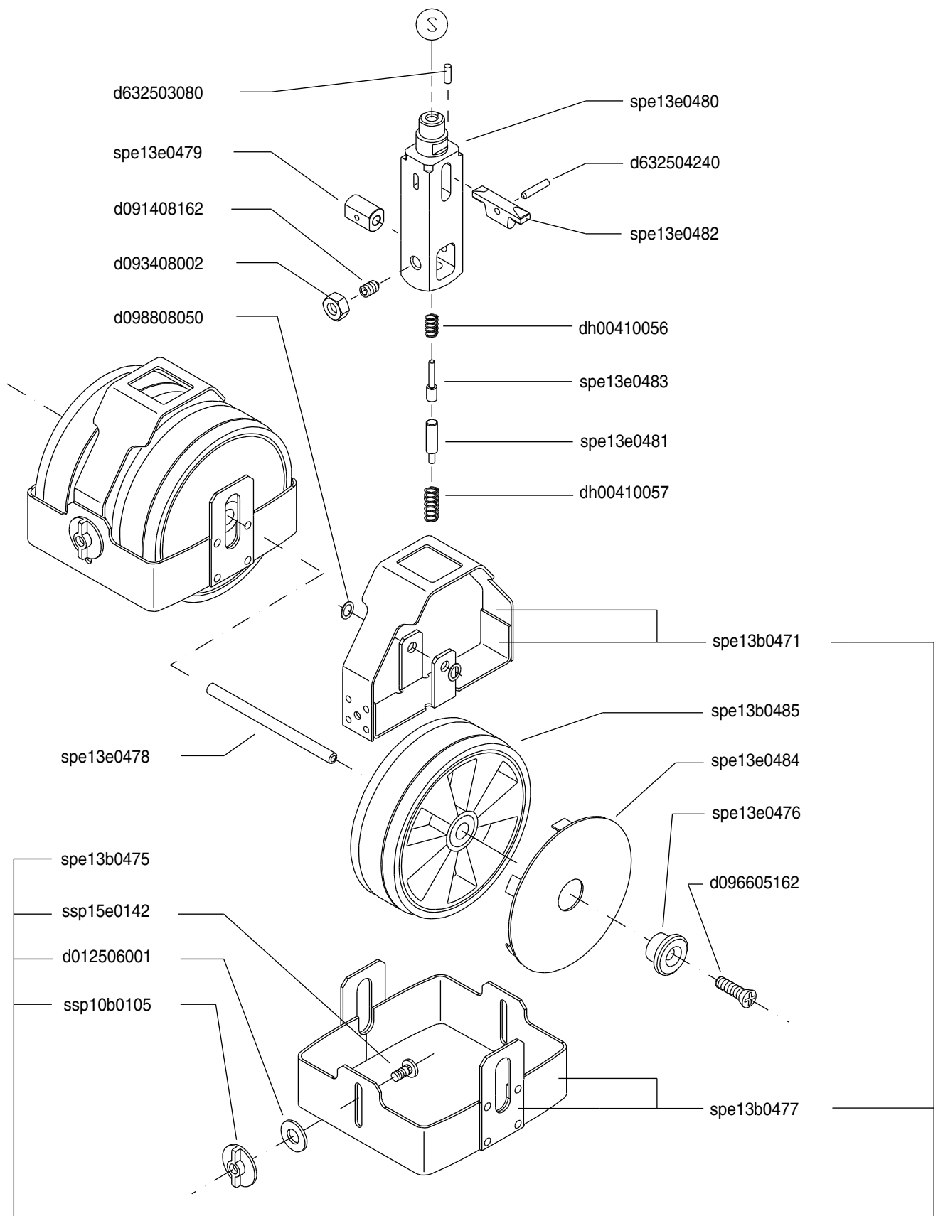
Studio Rad Laufrolle Ö125 (1 Stück) spe13b0470 studio wheel assembly Ö125 (1 piece) spe13b0470
