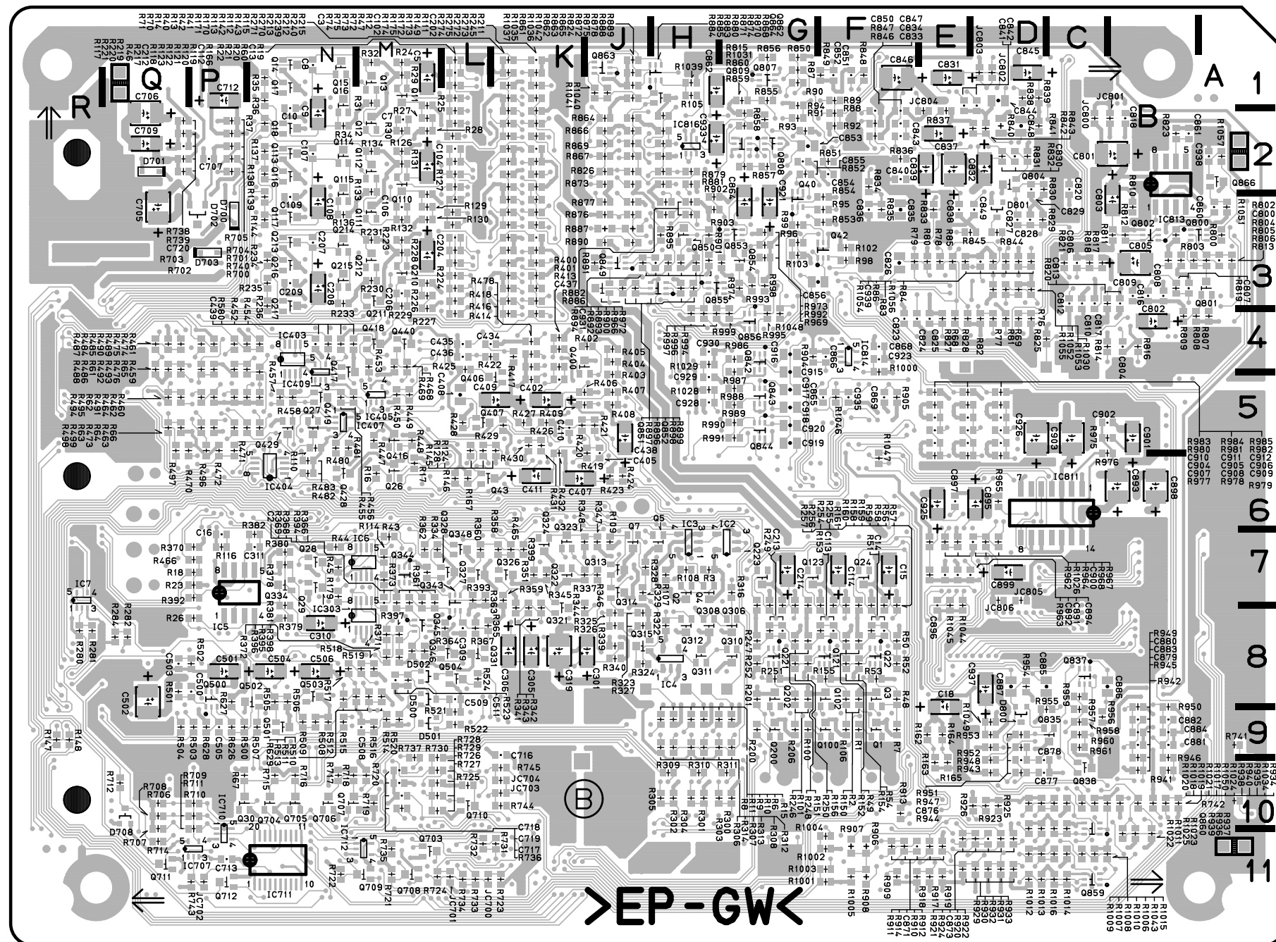
MS-57 -B SIDE- SUFFIX : -12
