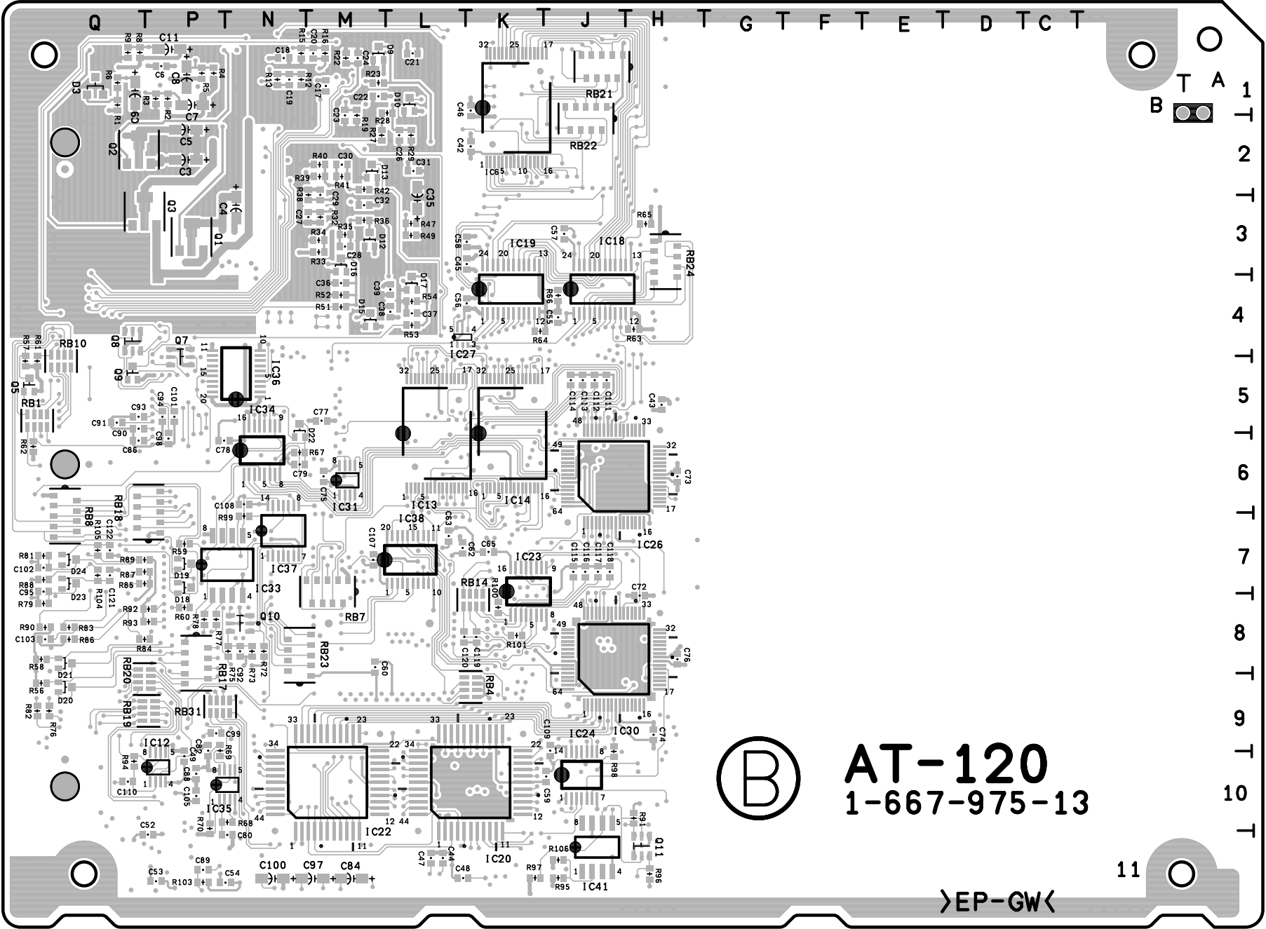
AT-120 -B SIDE- SUFFIX : -13
