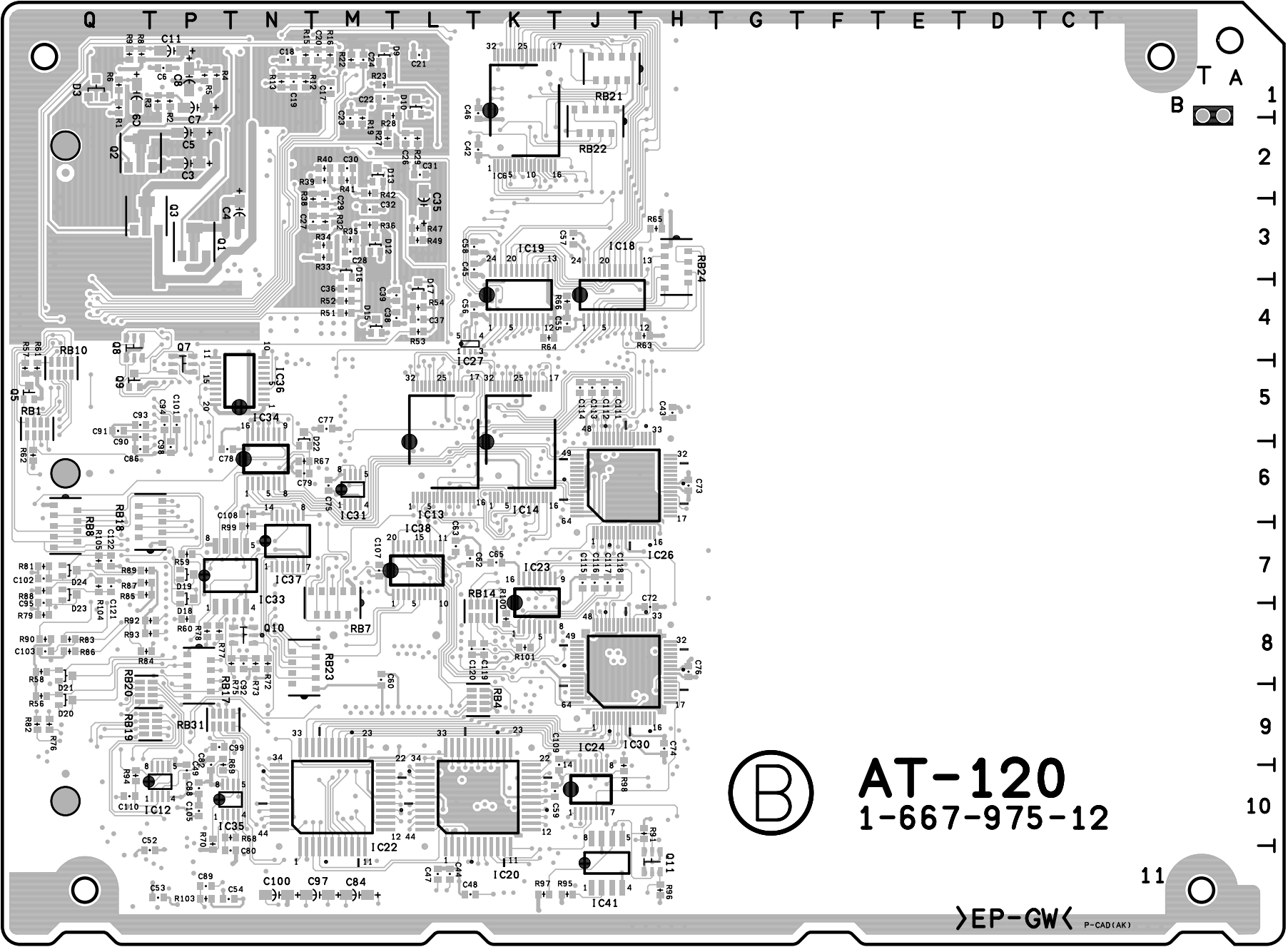
AT-120 -B SIDE- SUFFIX : -12
