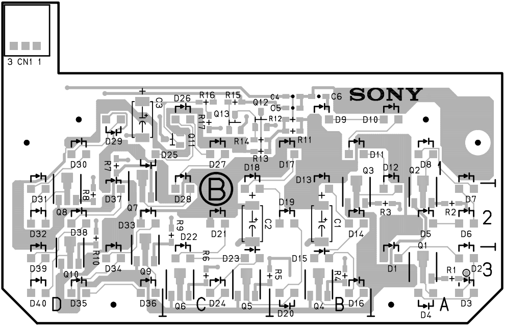
LE-172 -B SIDE- SUFFIX : -13 LE-216 -B SIDE- SUFFIX : -11
