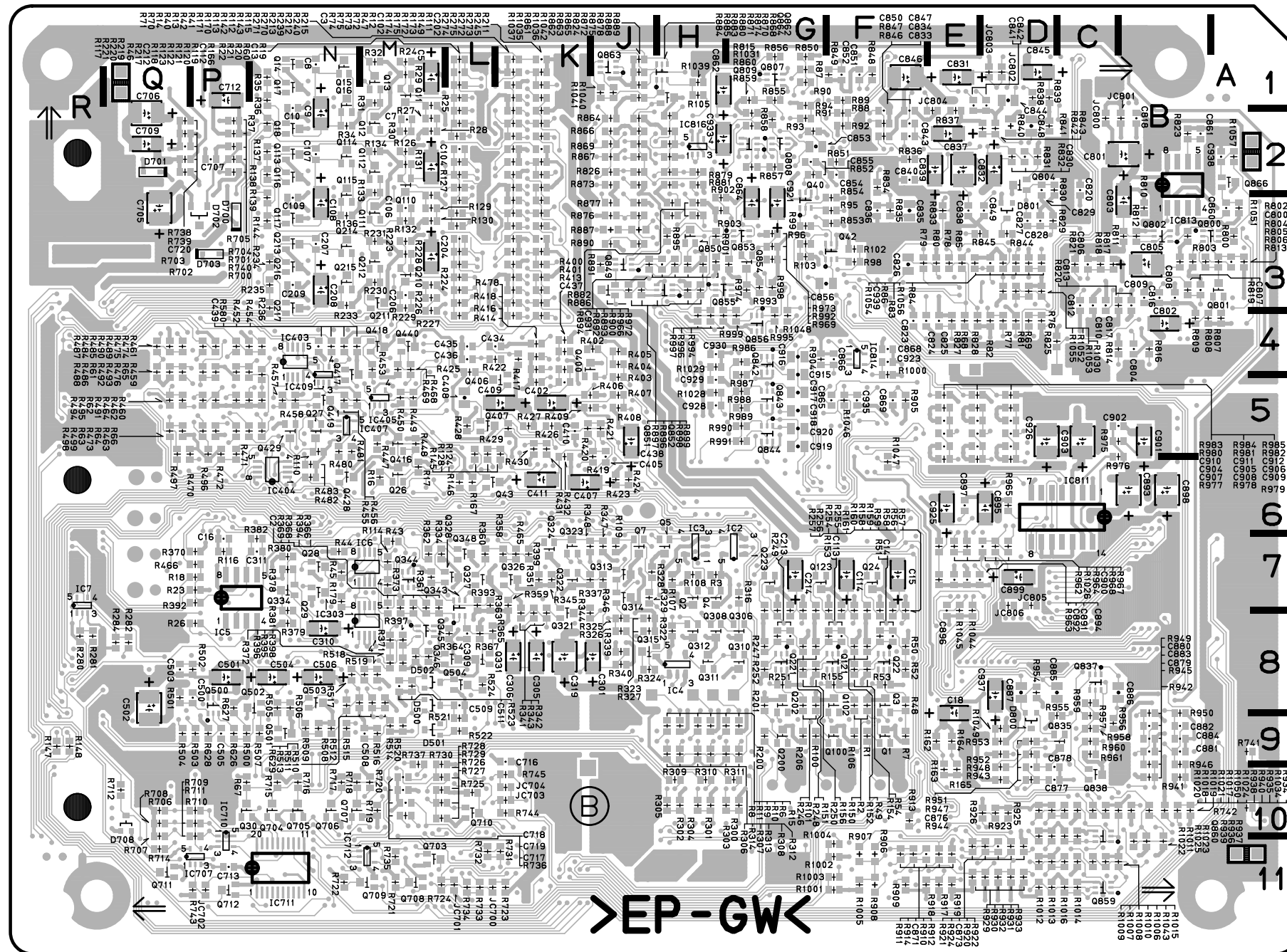
MS-57 -B SIDE- SUFFIX : -13
