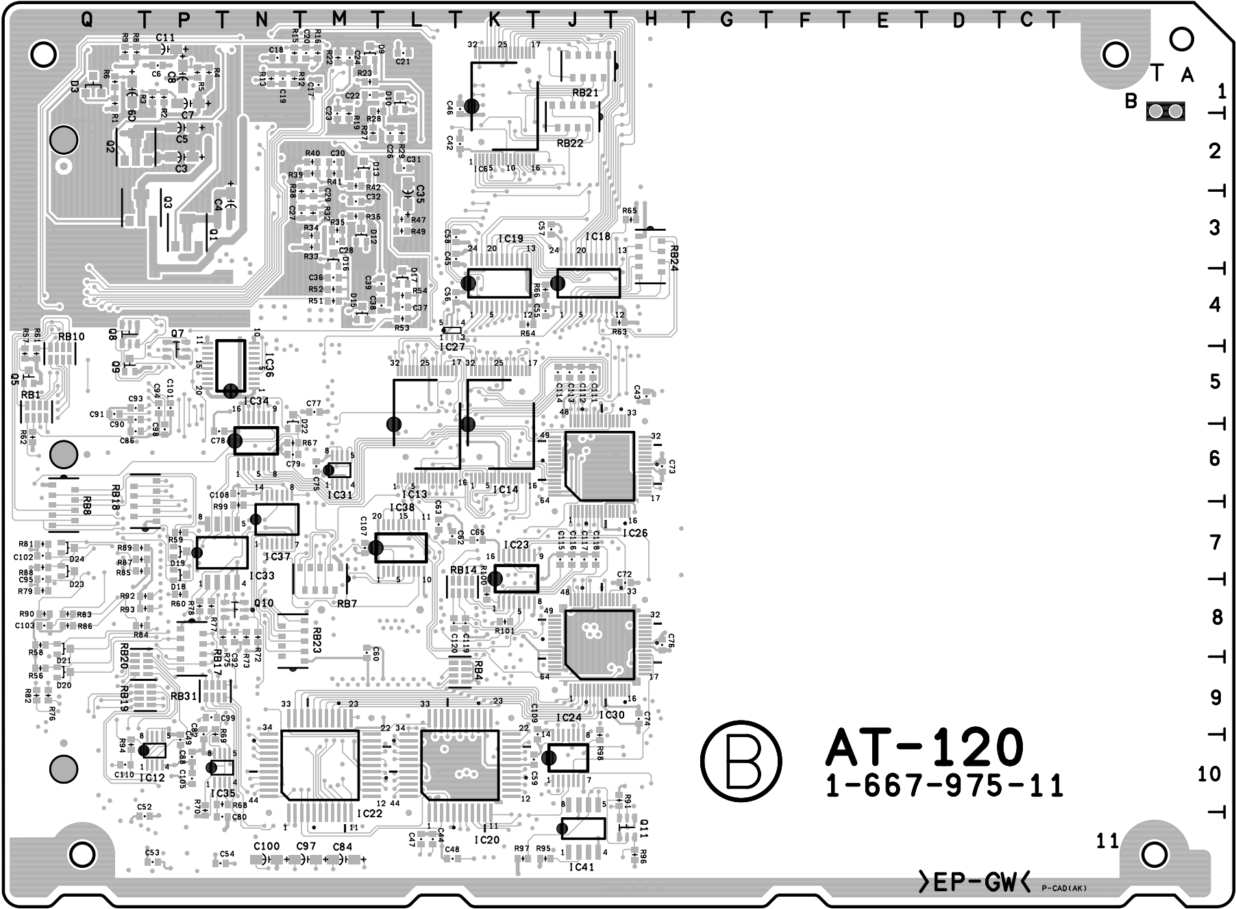
AT-120 -B SIDE- SUFFIX : -11
