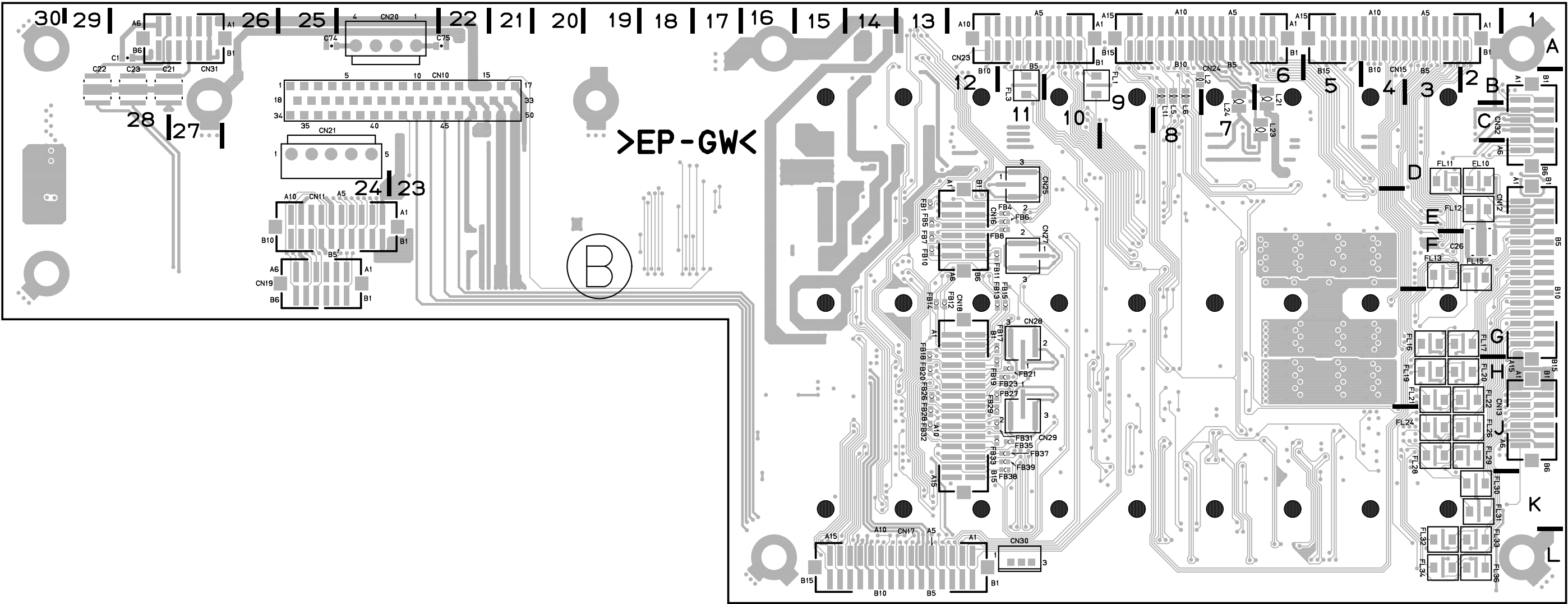
MB-764 -B SIDE- SUFFIX : -12
