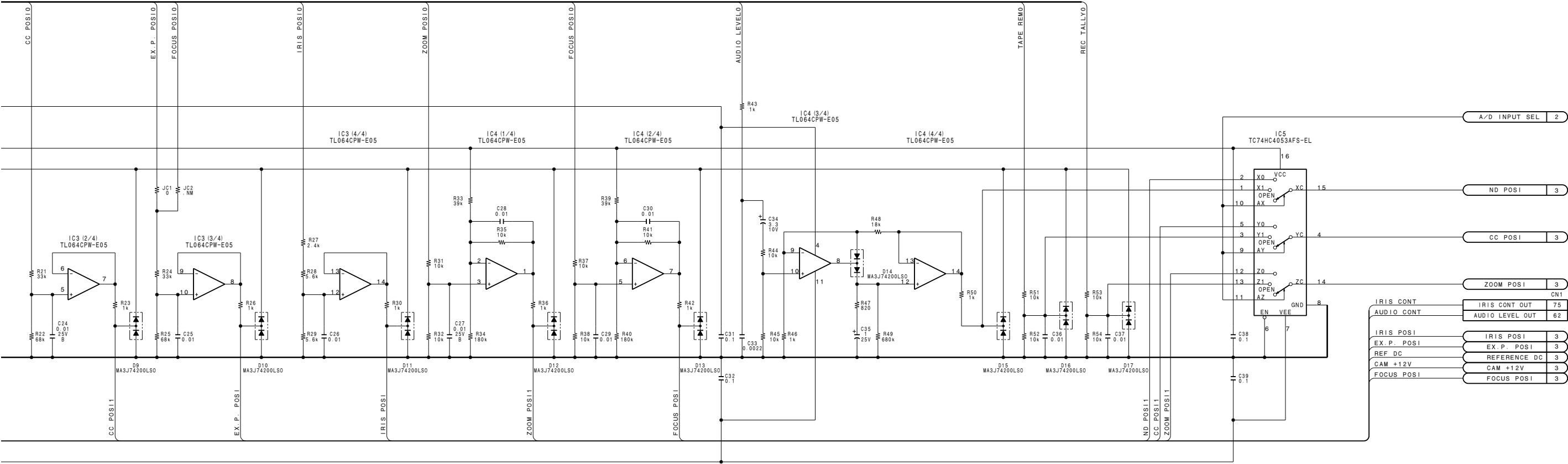
AT-120 (1/3) BOARD NO. 1-667-975-11, 12 LOT NO. 709- B-VBVP900-AT120-Z
