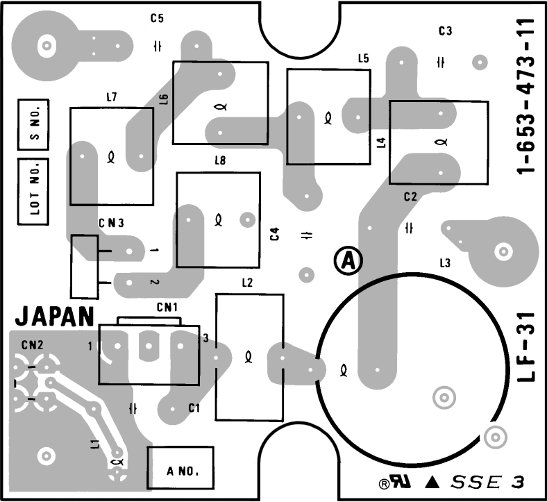
LF-31 -A SIDE- SUFFIX : -11
