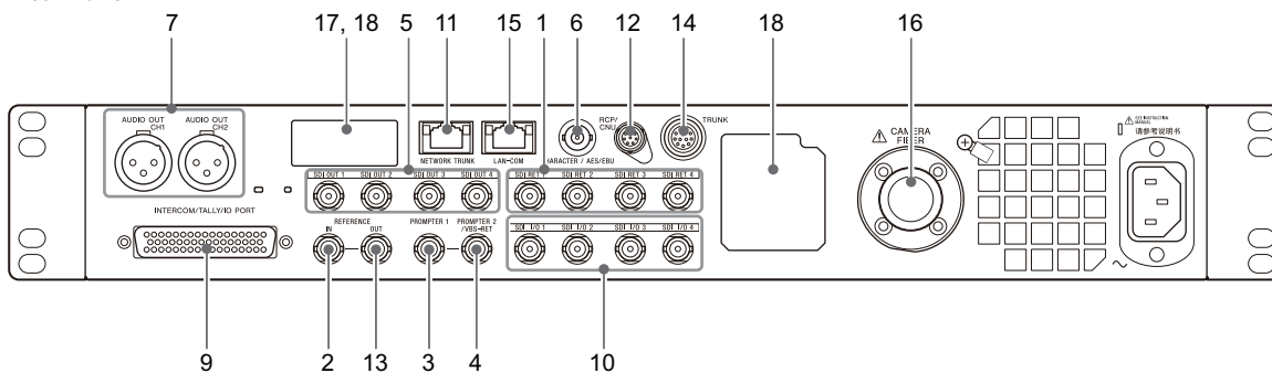
Rear Panel
