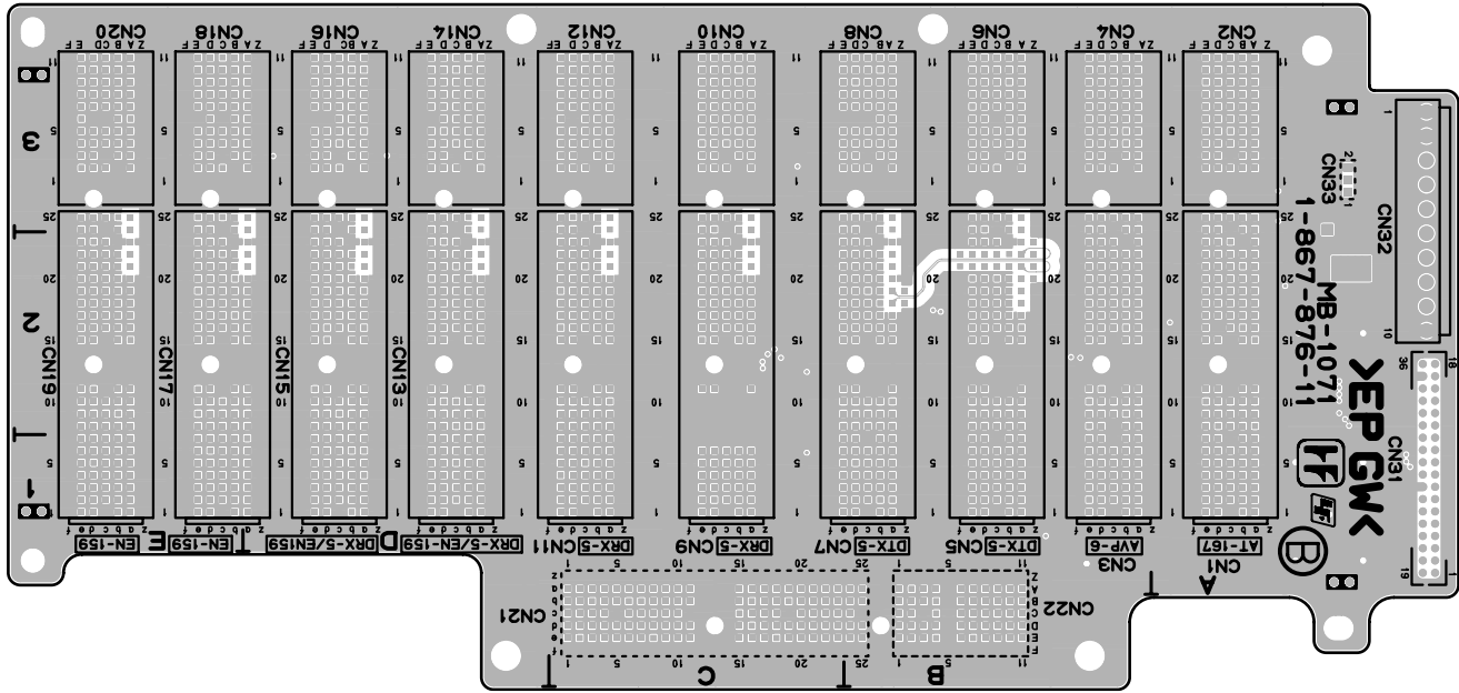
MB-1071 -B SIDE- SUFFIX: -11, 31
