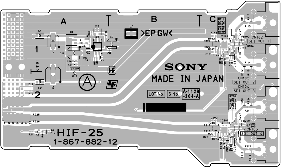
HIF-25 -A SIDE- SUFFIX: -12, 32
