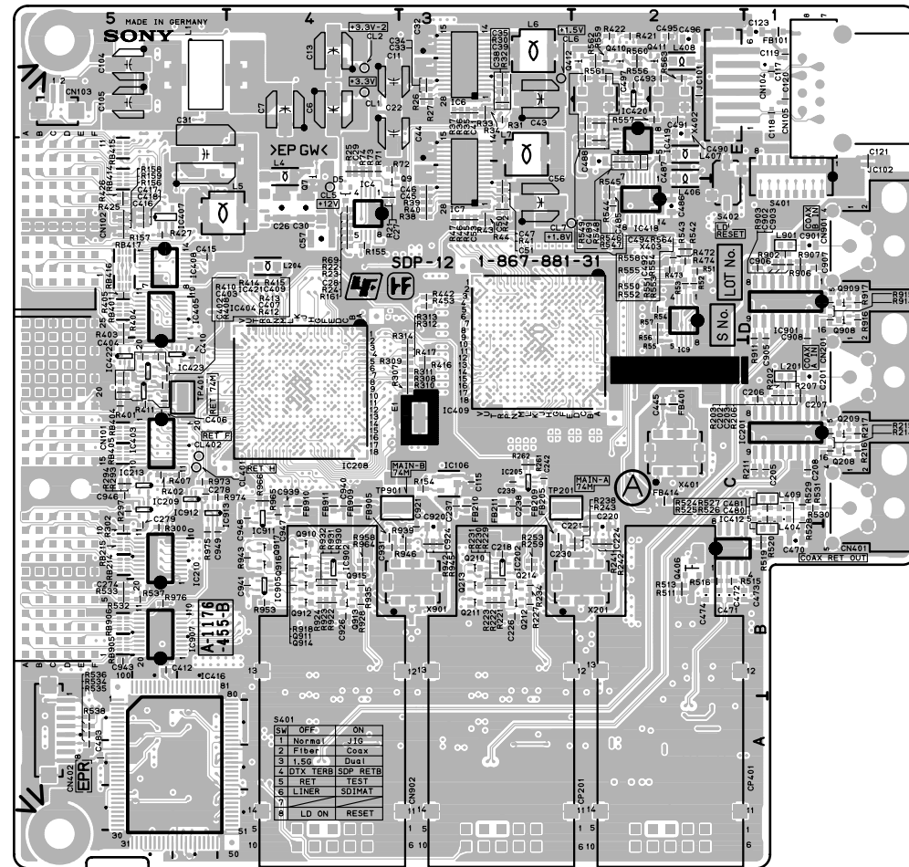
SDP-12 -A SIDE-SUFFIX: -13, 31
