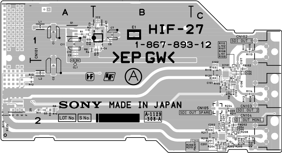
HIF-27 -A SIDE- SUFFIX: -12, 32
