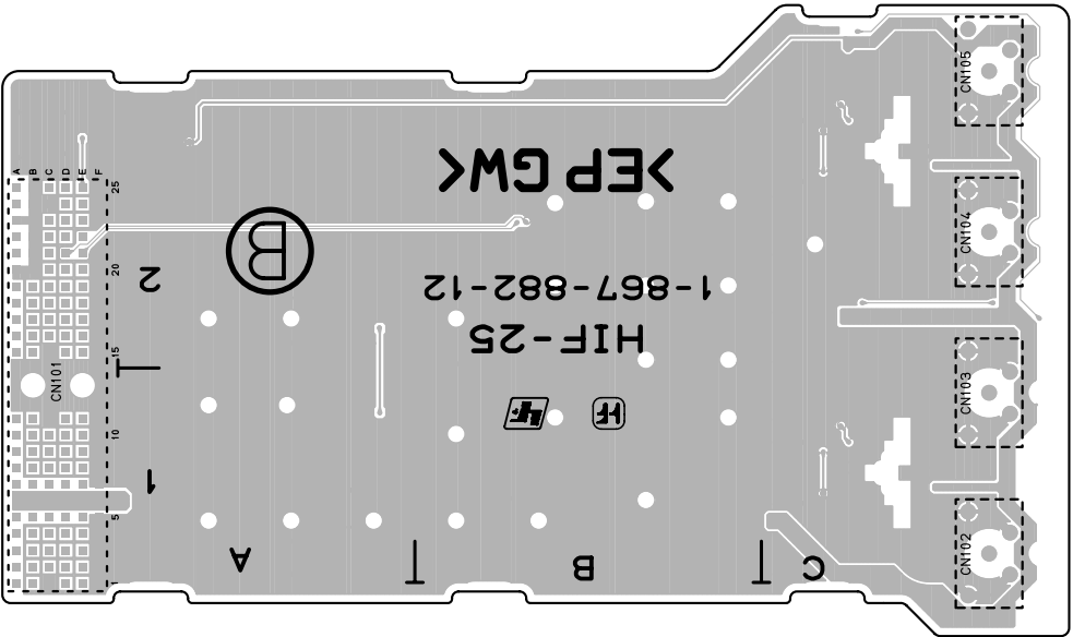
HIF-25 -B SIDE- SUFFIX: -12, 32
