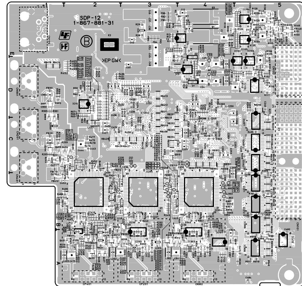
SDP-12 -B SIDE- SUFFIX: -13, 31
