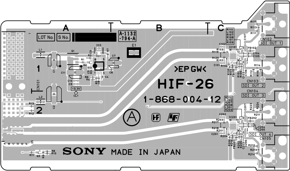
HIF-26 -A SIDE- SUFFIX: -12
