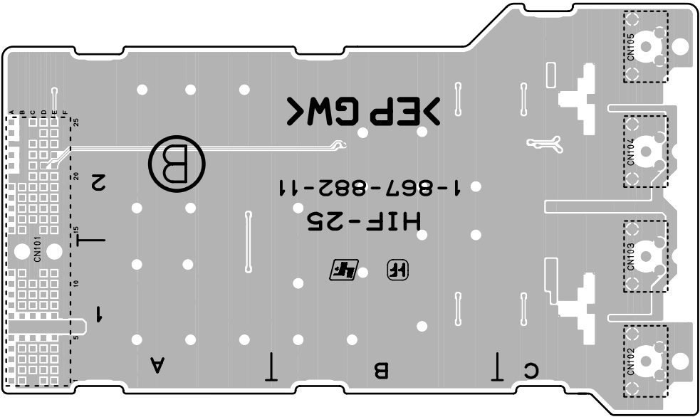
HIF-25 -B SIDE- SUFFIX: -11, 31
