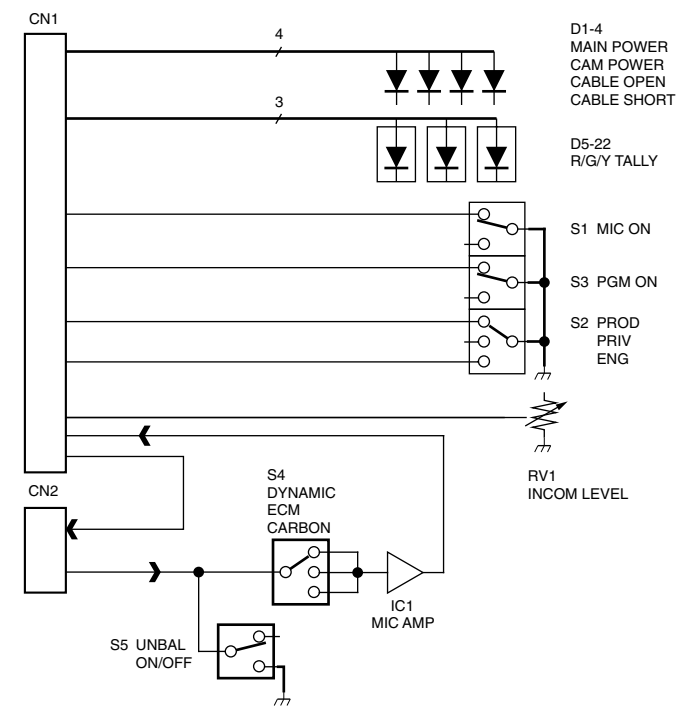
FRONT INTERCOM INTERFACE AU-302
