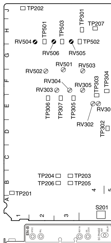
EN-159B board (A side and panel side )
