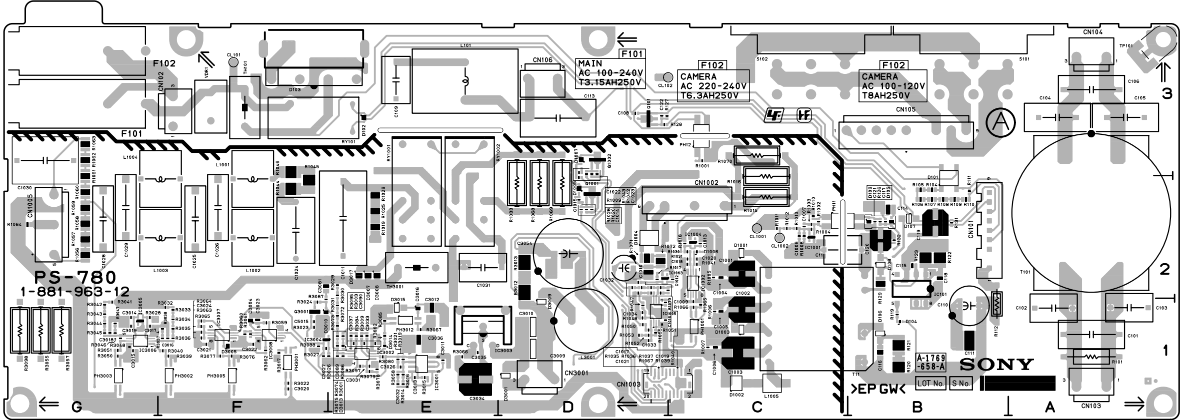
PS-780 -A SIDE- SUFFIX: -12
