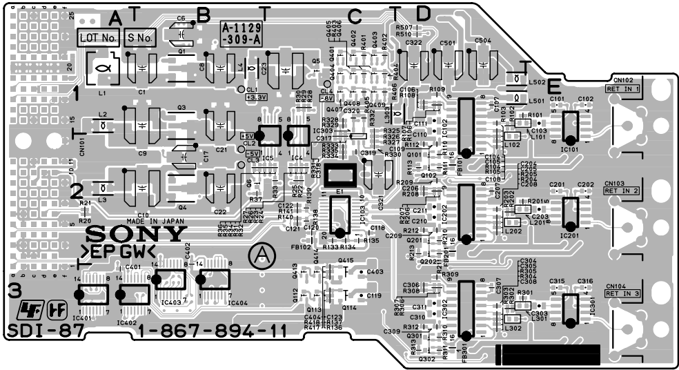
SDI-87 -A SIDE- SUFFIX: -11, 31
