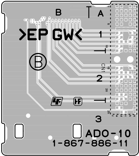
ADO-10 -B SIDE- SUFFIX: -11, 31
