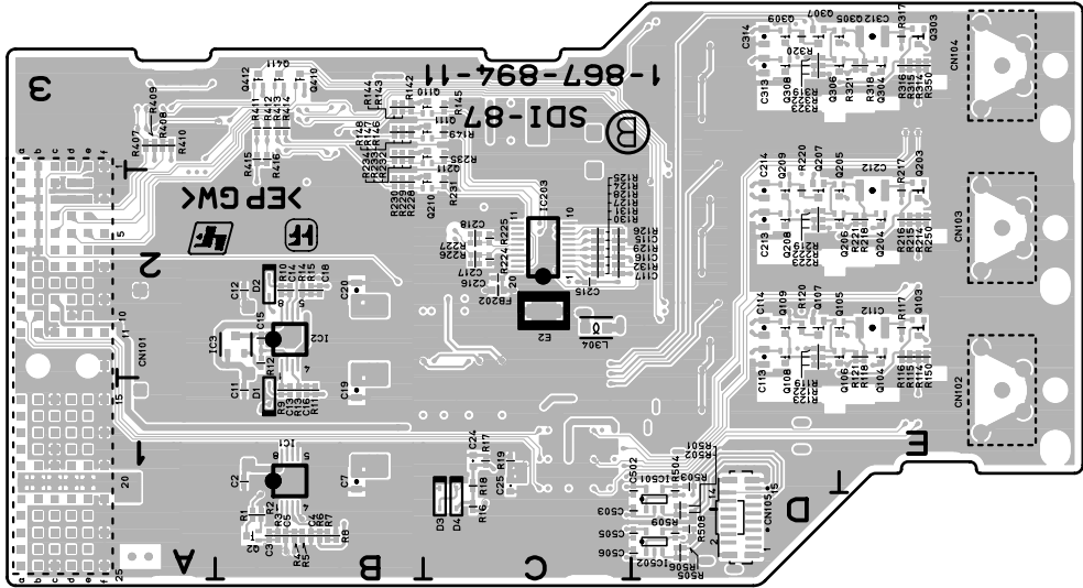
SDI-87 -B SIDE- SUFFIX: -11, 31
