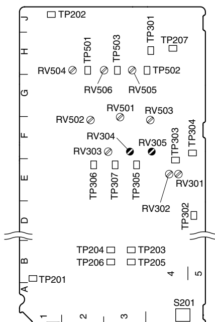
EN-159A/159B board (A side)
