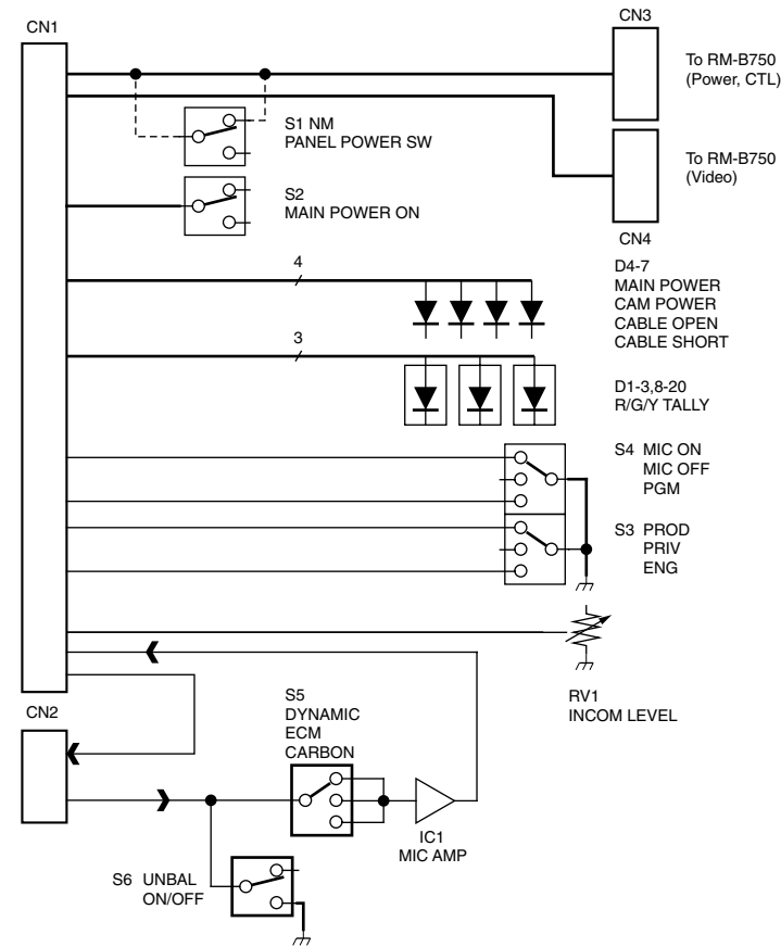
FRONT INTERCOM INTERFACE AU-303
