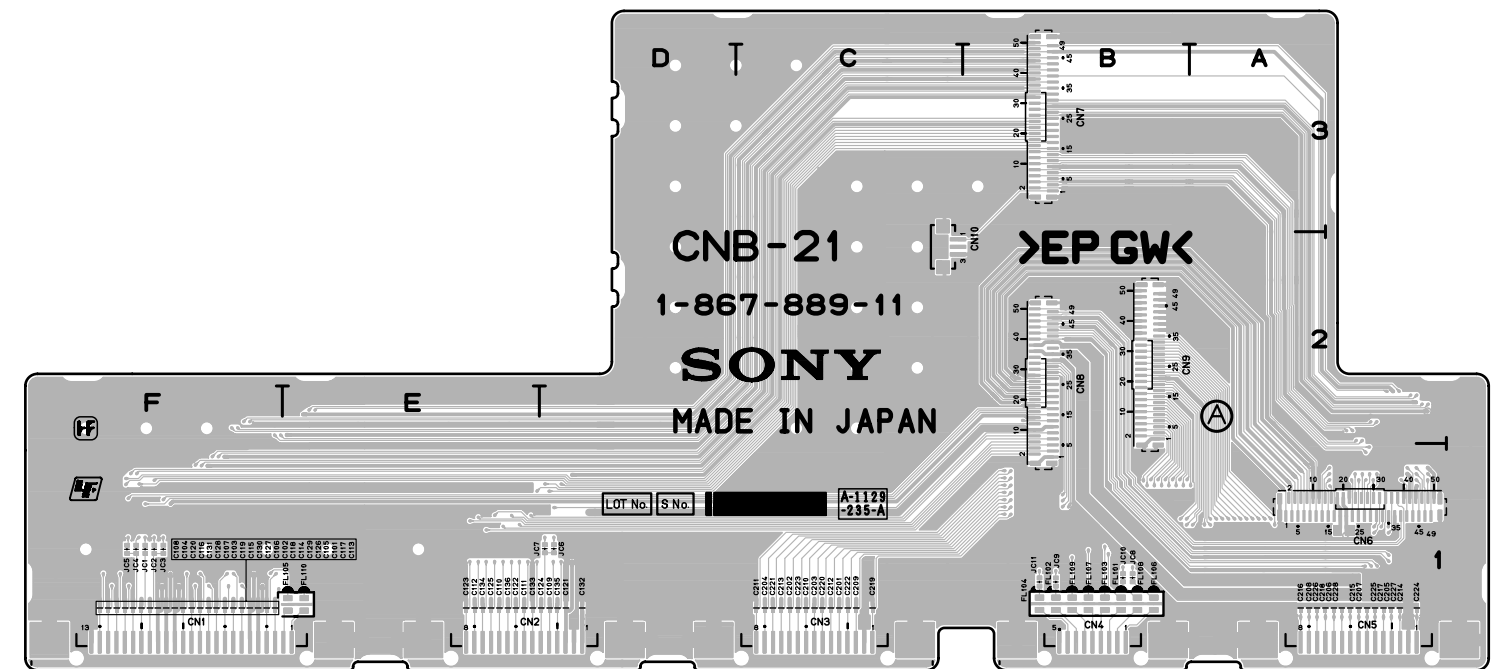
CNB-21 -A SIDE- SUFFIX: -11, 31
