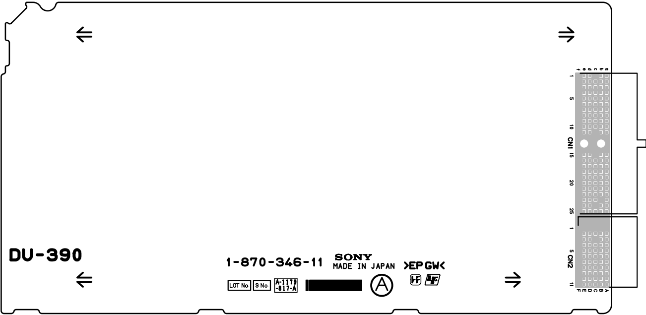
DU-390 -A SIDE- SUFFIX: -11
