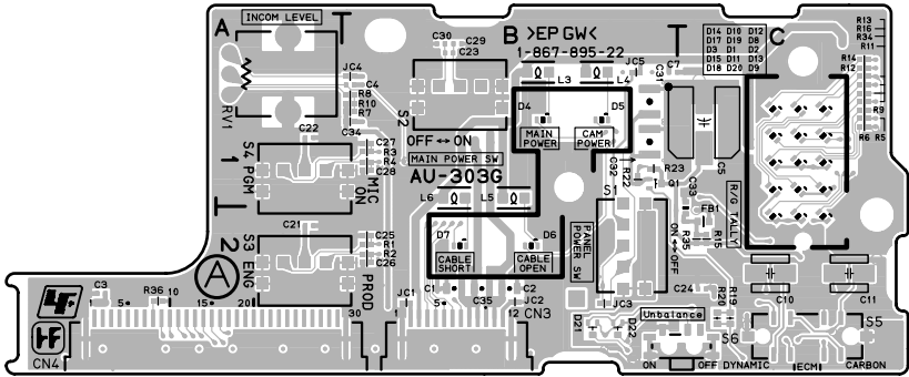
AU-303G -A SIDE- SUFFIX: -22, 31
