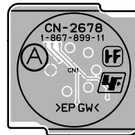
CN-2678 -A SIDE- SUFFIX: -11
