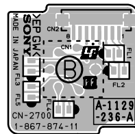
CN-2700 -B SIDE- SUFFIX: -11
