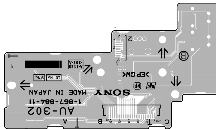
AU-302 -B SIDE- SUFFIX: -11, 12
