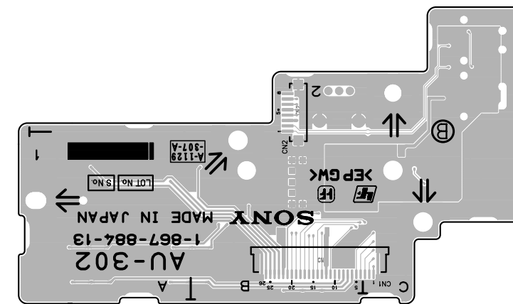
AU-302 -B SIDE- SUFFIX: -13
