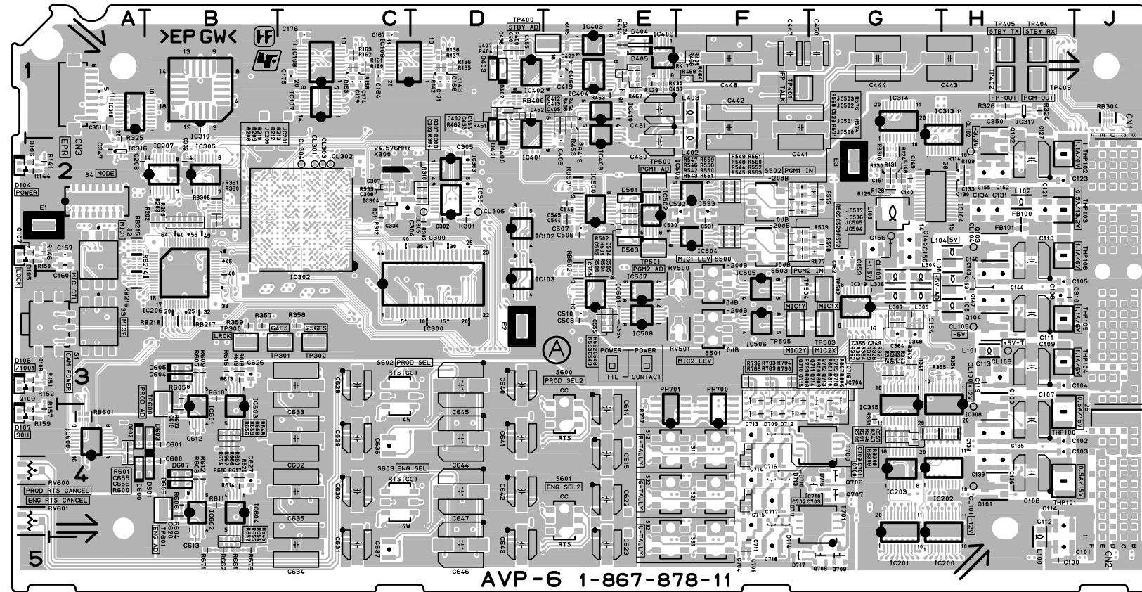
AVP-6 -A SIDE- SUFFIX: -11, 12, 31
