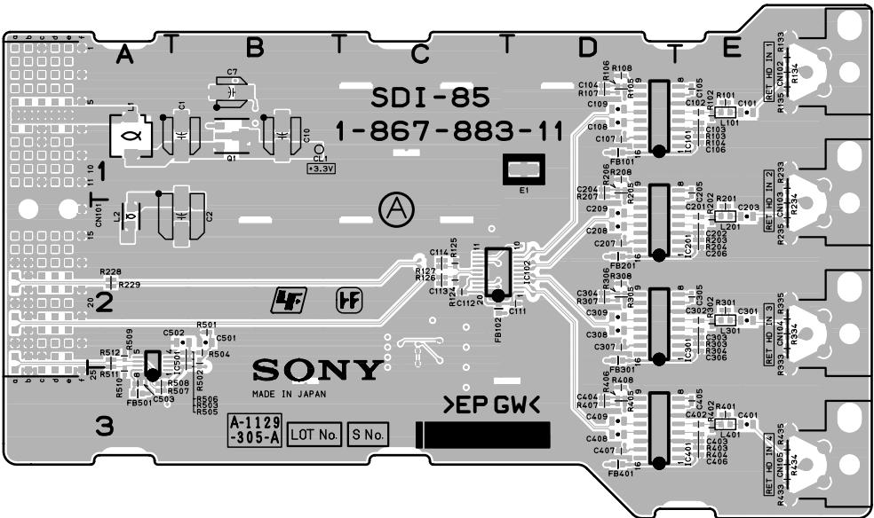
SDI-85 -A SIDE- SUFFIX: -11, 31
