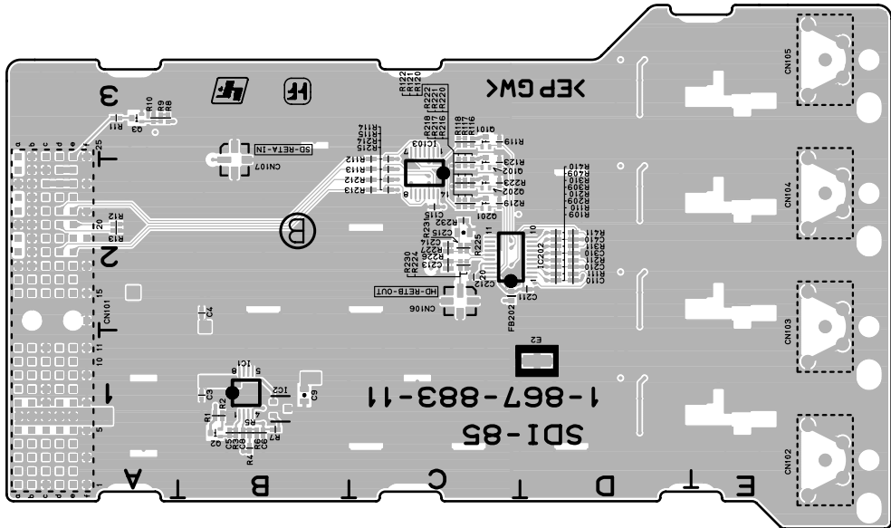
SDI-85 -B SIDE- SUFFIX: -11, 31
