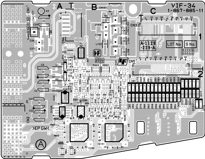
VIF-34 VIF-34B -A SIDE- SUFFIX: -11, 31
