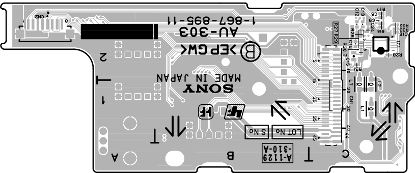
AU-303 -B SIDE- SUFFIX: -11
