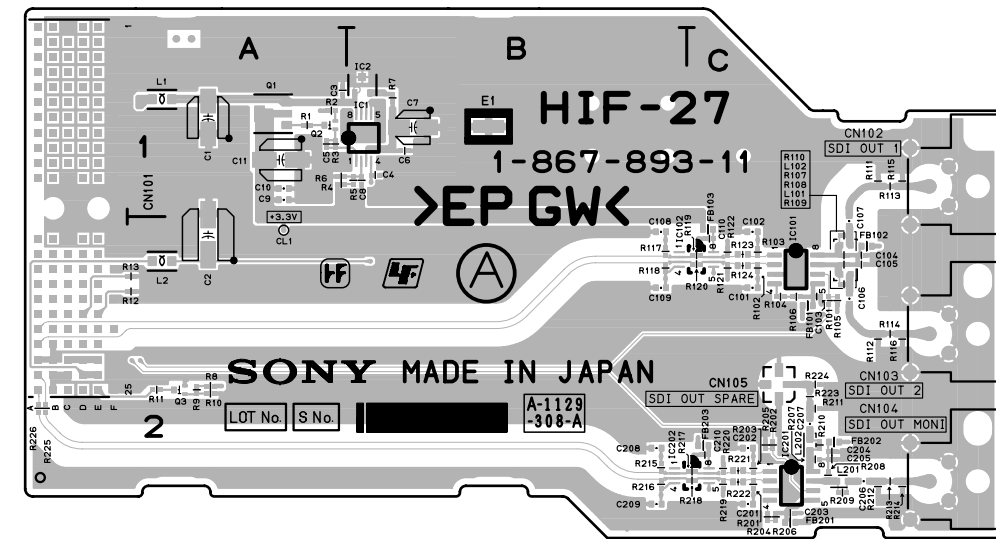
HIF-27 -A SIDE-SUFFIX: -11, 31
