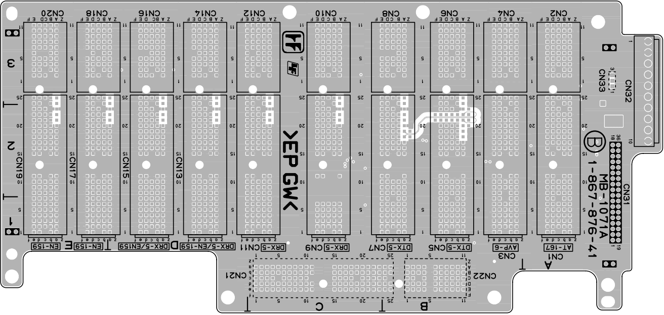
MB-1071A -B SIDE- SUFFIX: -41
