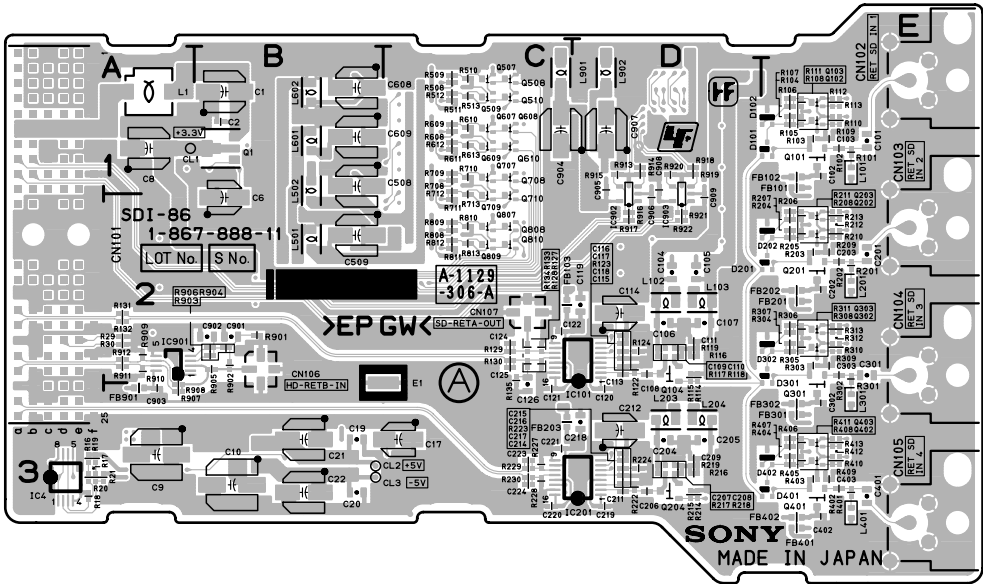
SDI-86 -A SIDE- SUFFIX: -11, 31
