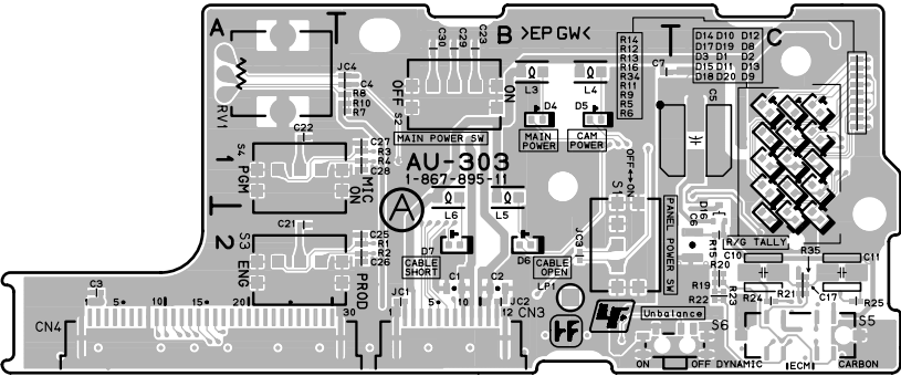
AU-303 -A SIDE- SUFFIX: -11
