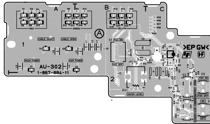
AU-302 -A SIDE-SUFFIX: -11, 12
