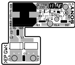
DU-565 -A SIDE- SUFFIX: -11
