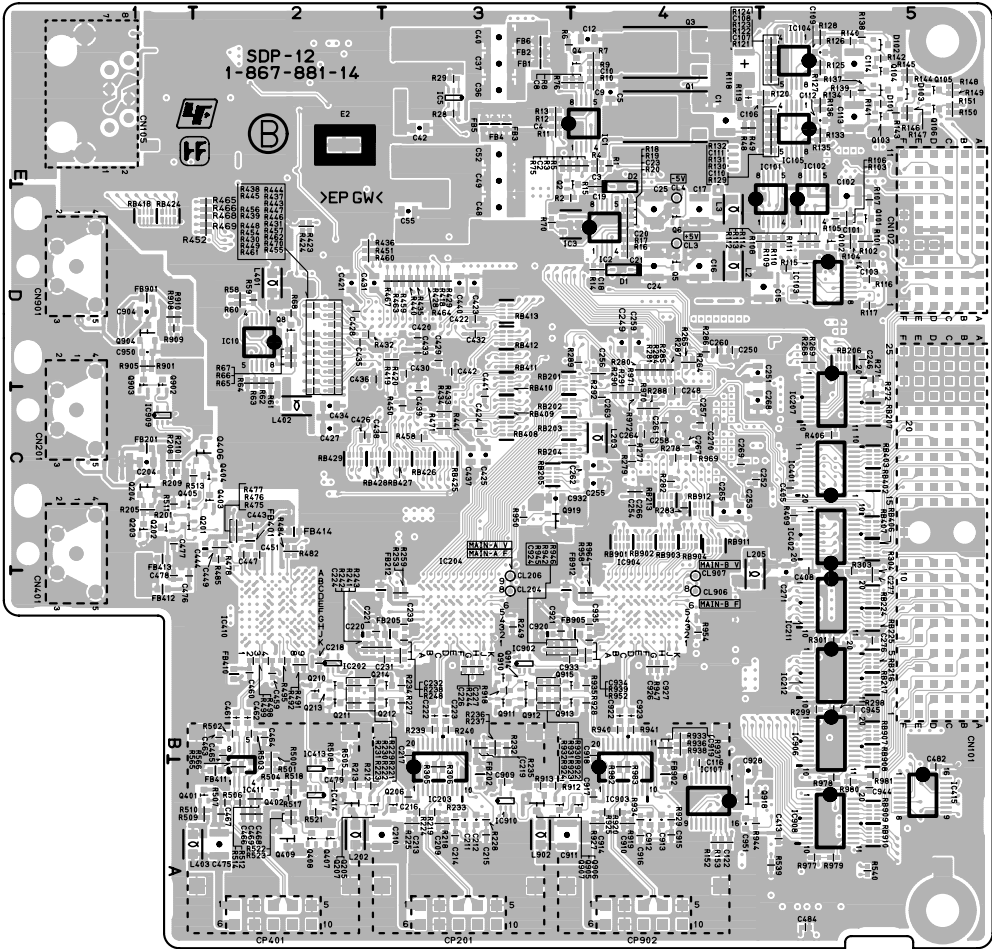
SDP-12 -B SIDE- SUFFIX: -14
