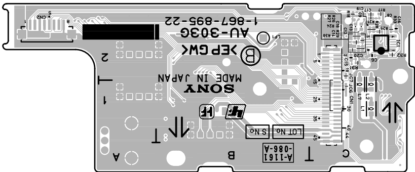
AU-303G -B SIDE- SUFFIX: -22, 31
