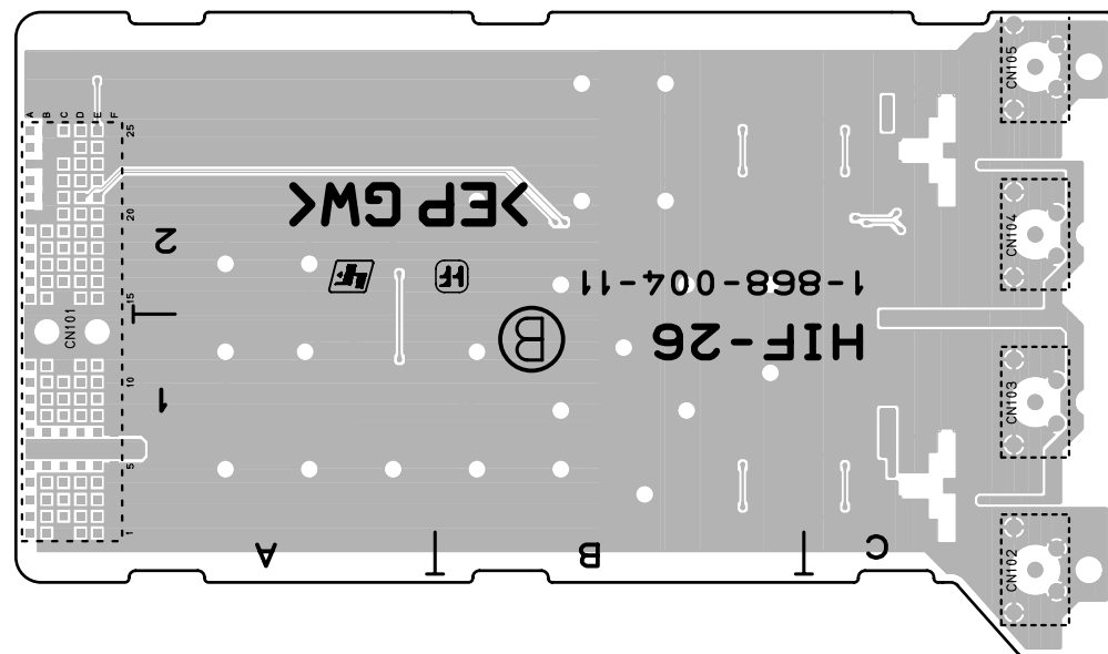
HIF-26 -B SIDE- SUFFIX: -11
