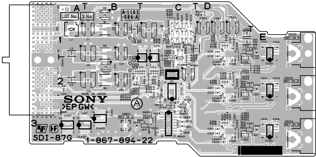
SDI-87G -A SIDE- SUFFIX: -22, 32
