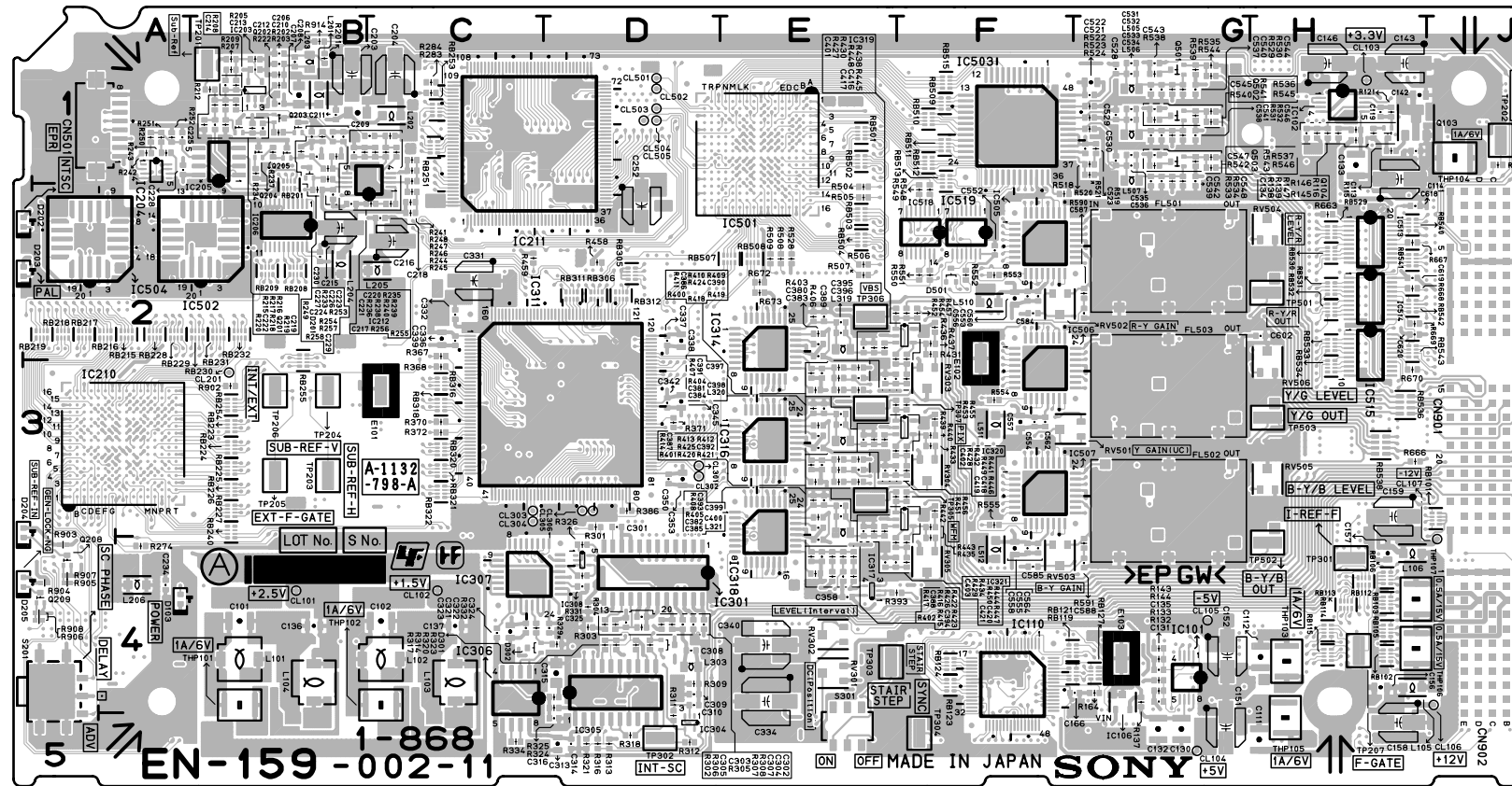
EN-159A EN-159B -A SIDE- SUFFIX: -11
