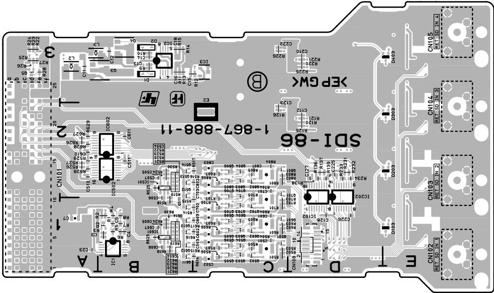
SDI-86 -B SIDE- SUFFIX: -11, 31
