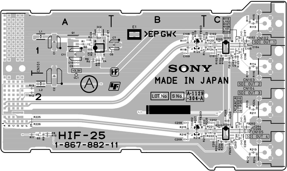
HIF-25 -A SIDE- SUFFIX: -11, 31
