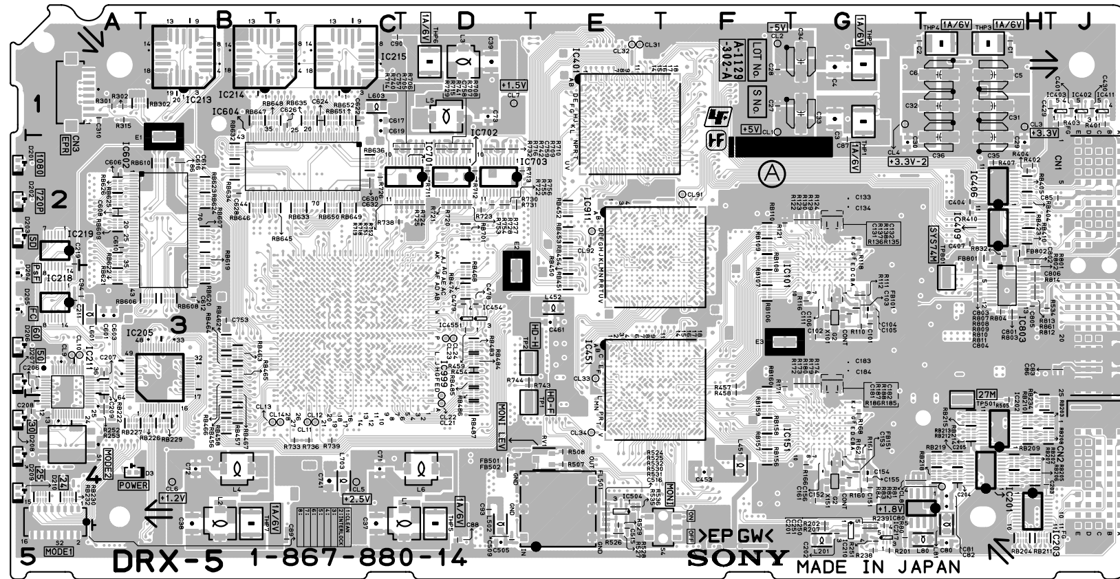
DRX-5 -A SIDE- SUFFIX: -14
