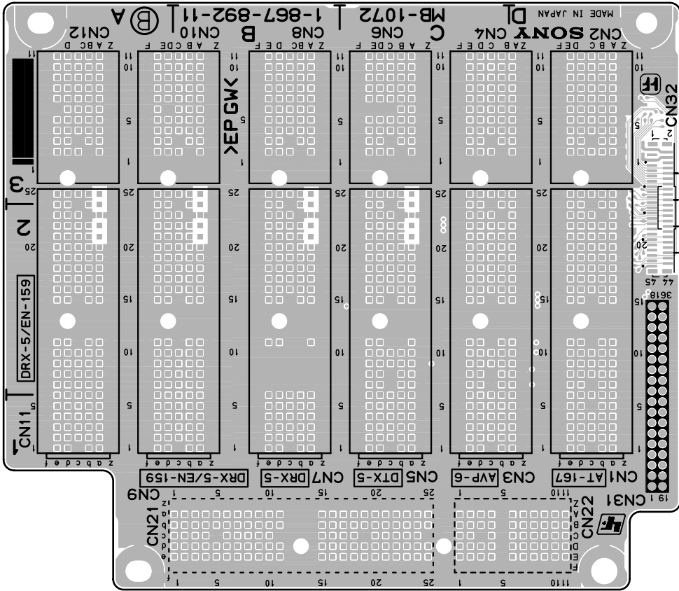
MB-1072 -B SIDE- SUFFIX: -11, 31
