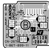
CN-2678 -B SIDE- SUFFIX: -11
