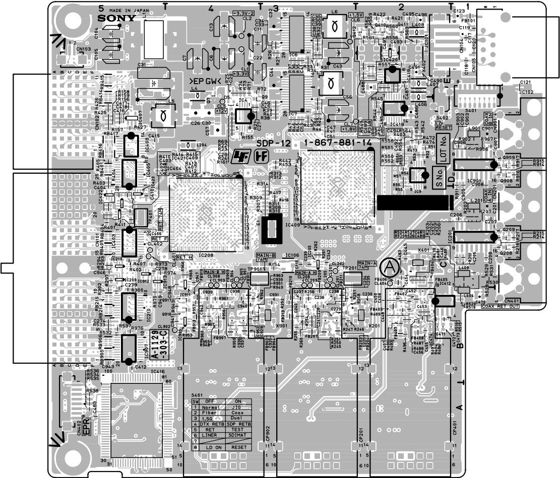
SDP-12 -A SIDE- SUFFIX: -14
