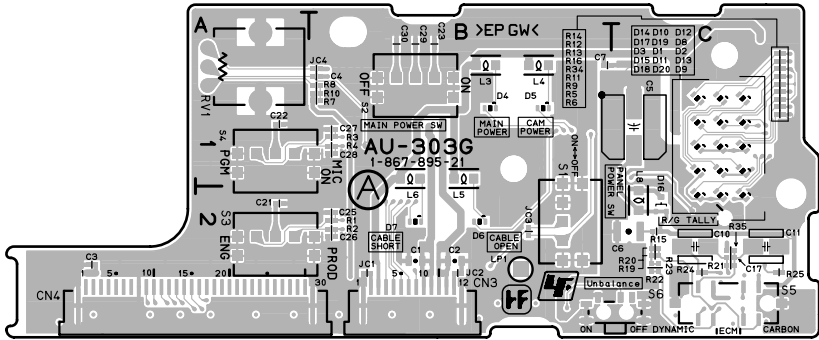
AU-303G -A SIDE- SUFFIX: -21
