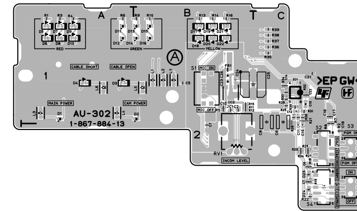
AU-302 -A SIDE-SUFFIX: -13
