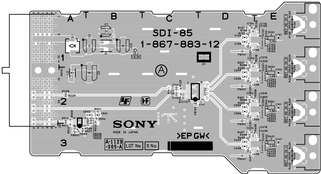
SDI-85 -A SIDE- SUFFIX: -12, 32
