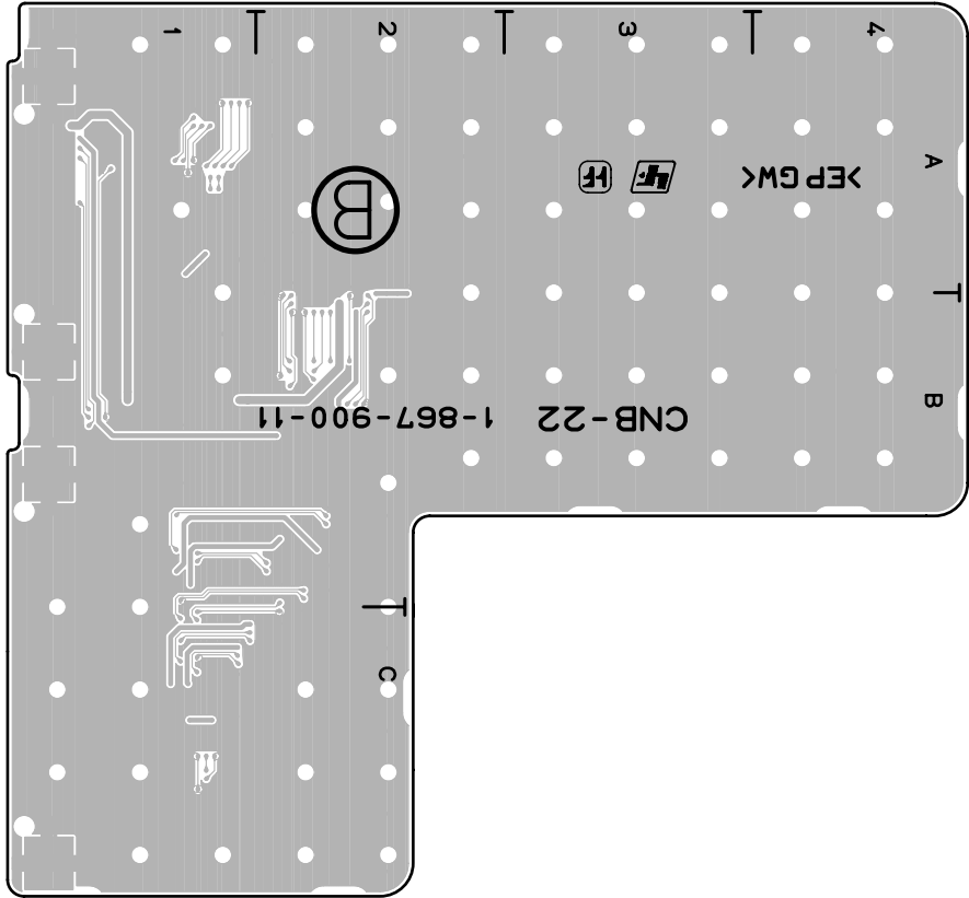
CNB-22 -B SIDE- SUFFIX: -11, 31
