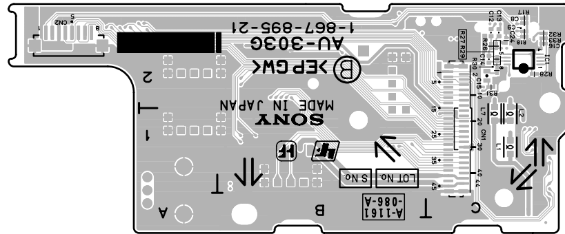
AU-303G -B SIDE- SUFFIX: -21
