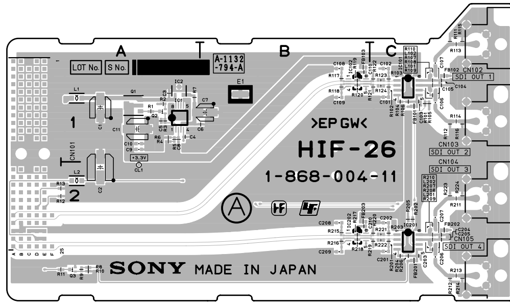
HIF-26 -A SIDE-SUFFIX: -11
