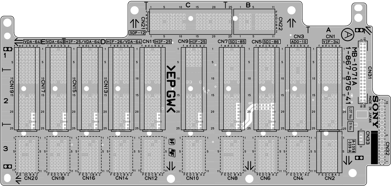
MB-1071A -A SIDE- SUFFIX: -41
