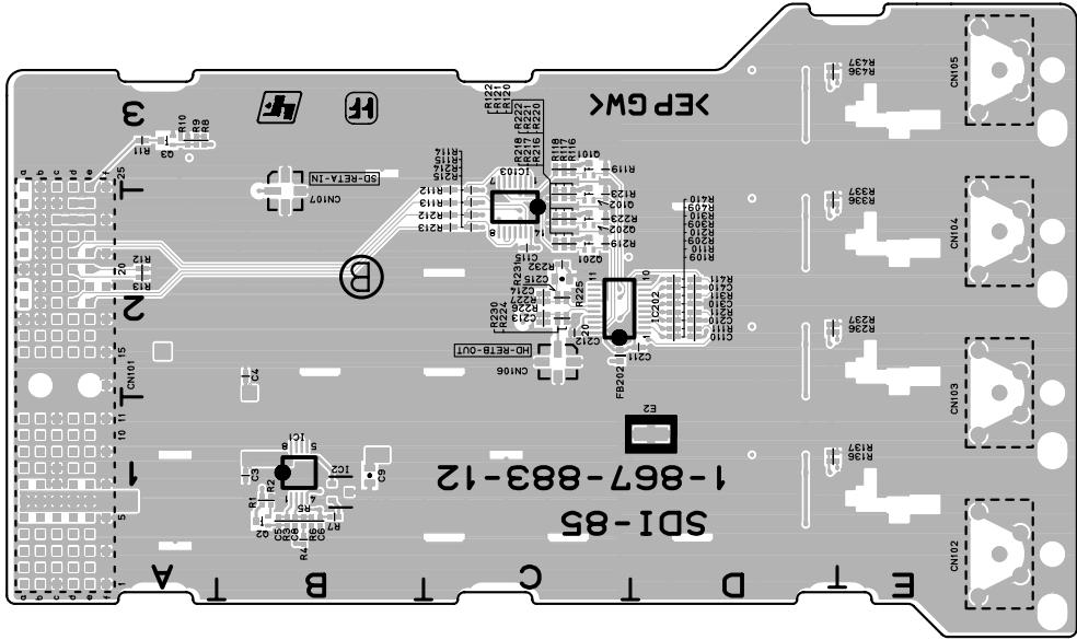
SDI-85 -B SIDE- SUFFIX: -12, 32
