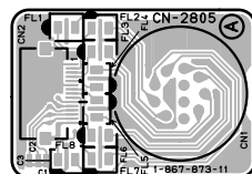
CN-2805 -A SIDE- SUFFIX: -11, 31
