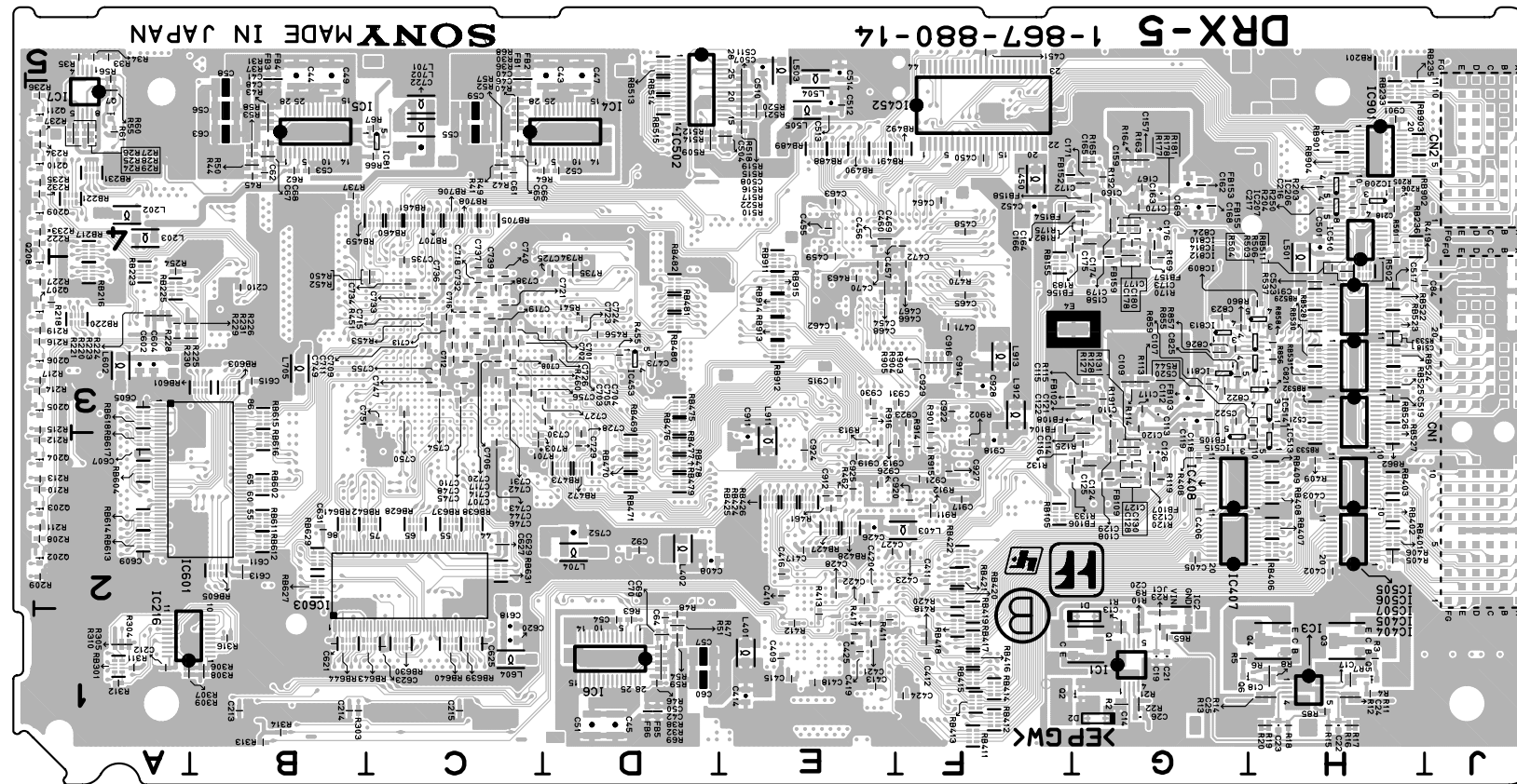
DRX-5 -B SIDE- SUFFIX: -14
