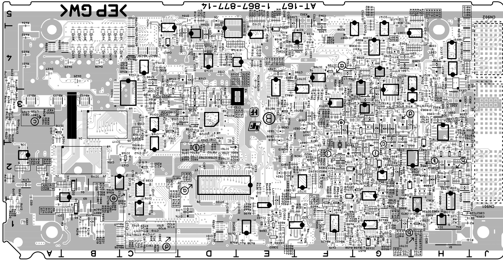
AT-167 -B SIDE- SUFFIX: -14
