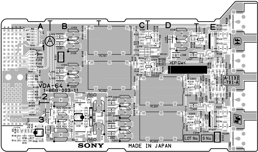
VDA-64A VDA-64B VDA-64C -A SIDE- SUFFIX: -11, 12
