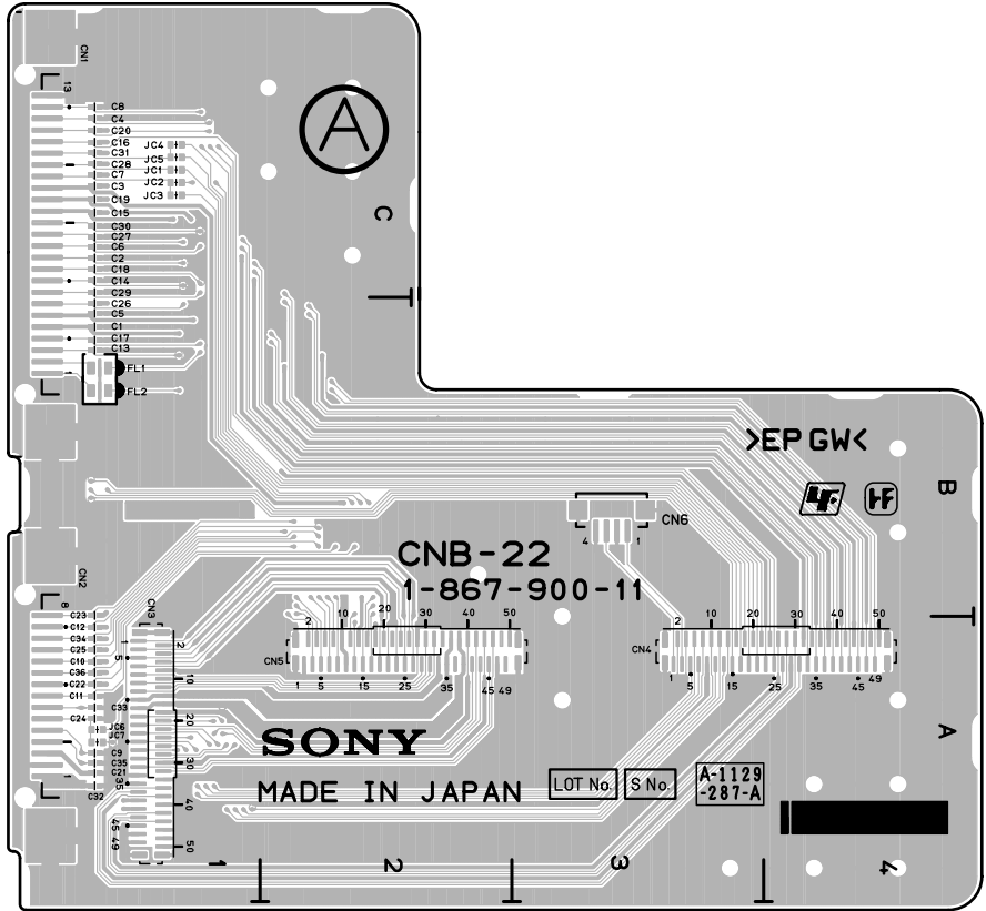
CNB-22 -A SIDE- SUFFIX: -11, 31
