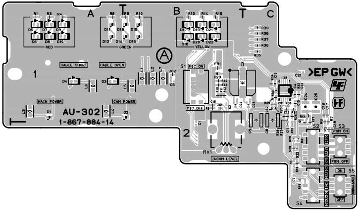
AU-302 -A SIDE- SUFFIX: -14, 31
