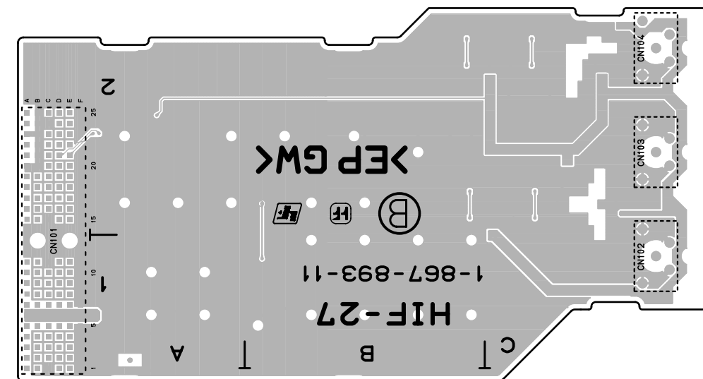
HIF-27 -B SIDE- SUFFIX: -11, 31
