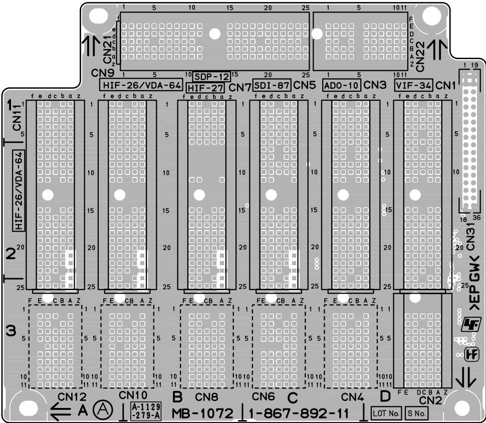
MB-1072 -A SIDE- SUFFIX: -11, 31
