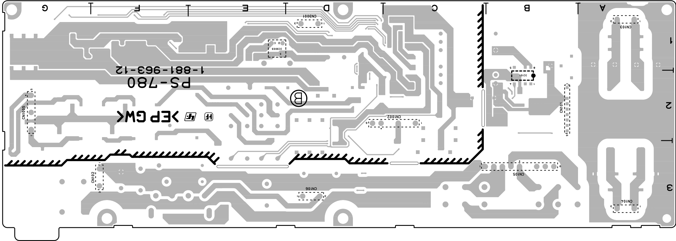
PS-780 -B SIDE- SUFFIX: -12
