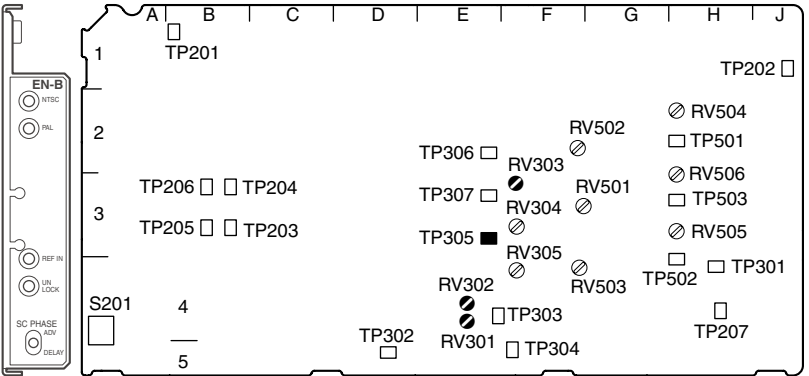
EN-159A/159B board (A side and panel side)
