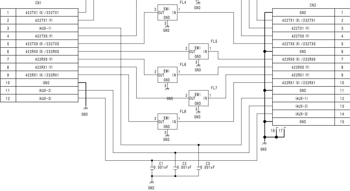
CN-2805G BOARD NO. 1-867-873-11
