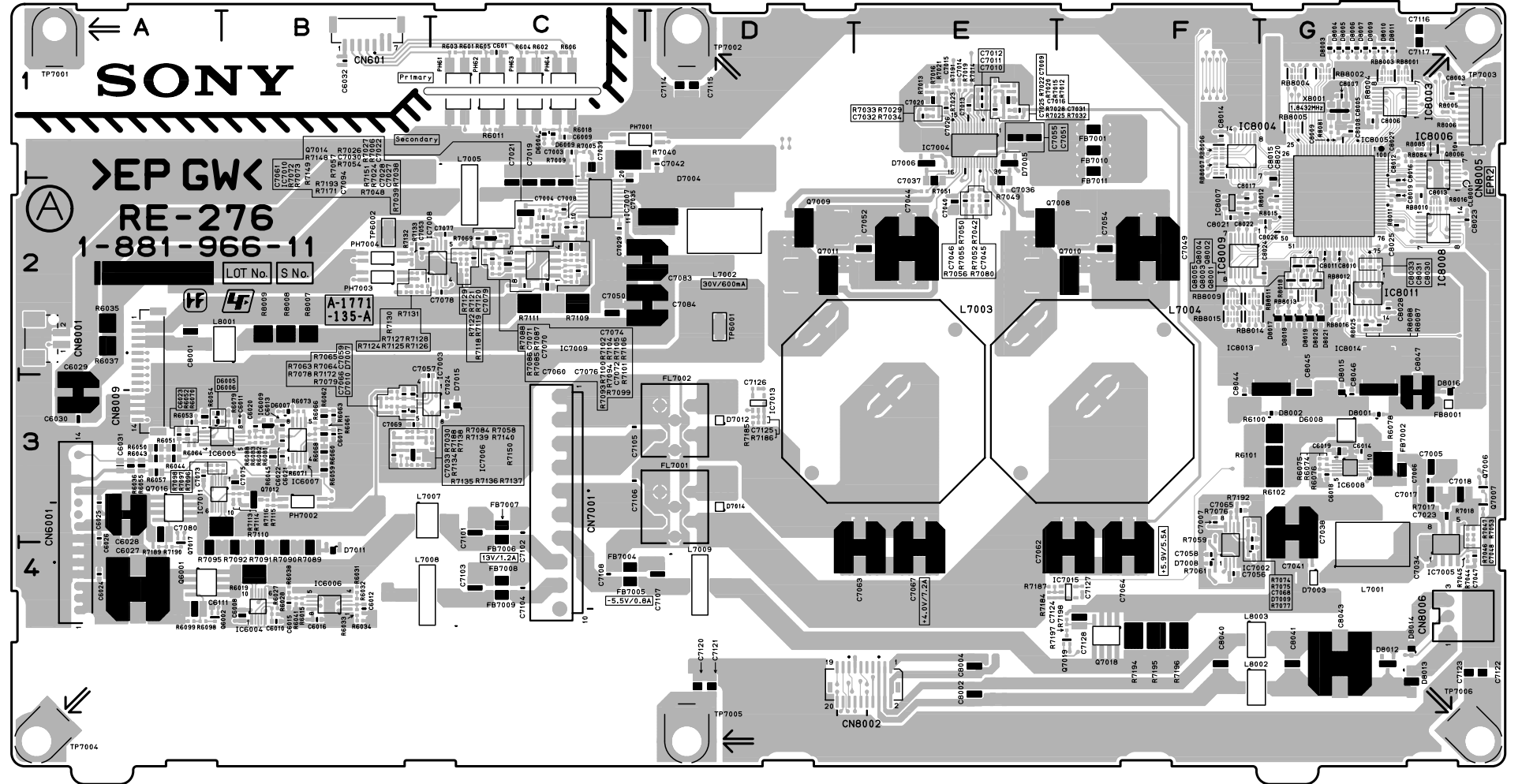
RE-276 -A SIDE-SUFFIX: -11
