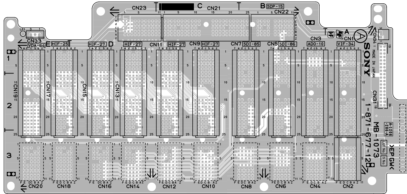
MB-1073 -A SIDE-SUFFIX: -12
