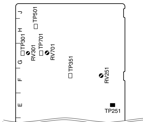
DTX-5 board (A side)
