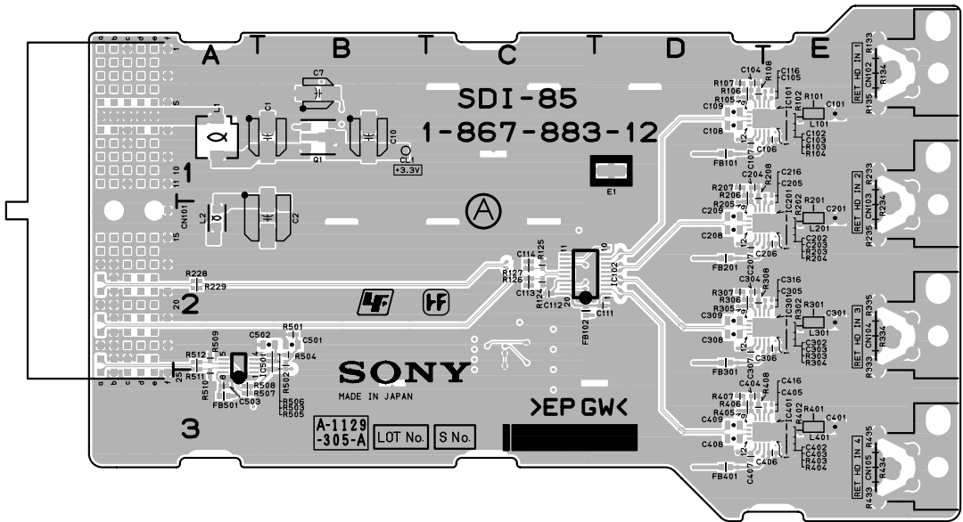
SDI-85 -A SIDE- SUFFIX: -12
