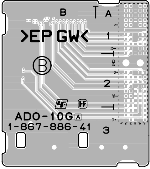
ADO-10GA -B SIDE- SUFFIX: -41
