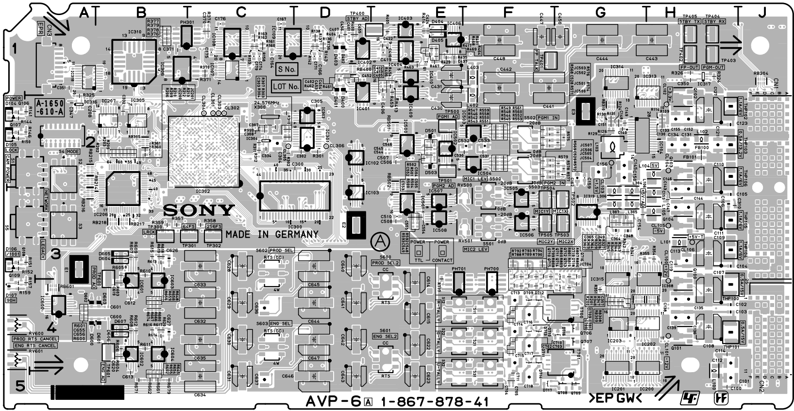
AVP-6A -A SIDE- SUFFIX: -41
