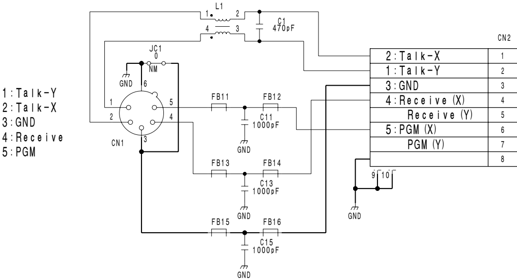
CN-2700 BOARD NO. 1-867-874-12
