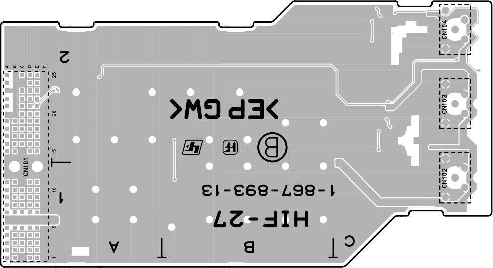
HIF-27 -B SIDE- SUFFIX: -13
