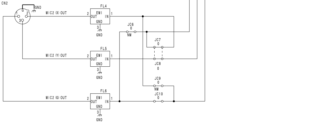
CN-2673 BOARD NO. 1-867-887-11
