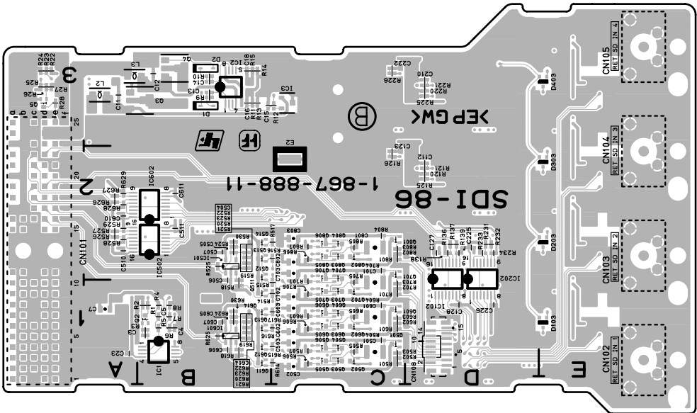
SDI-86G -B SIDE- SUFFIX: -11
