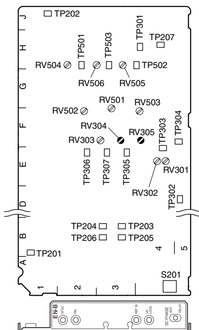
EN-159A/159B board (A side and panel side)
