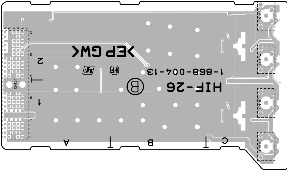
HIF-26 -B SIDE- SUFFIX: -13
