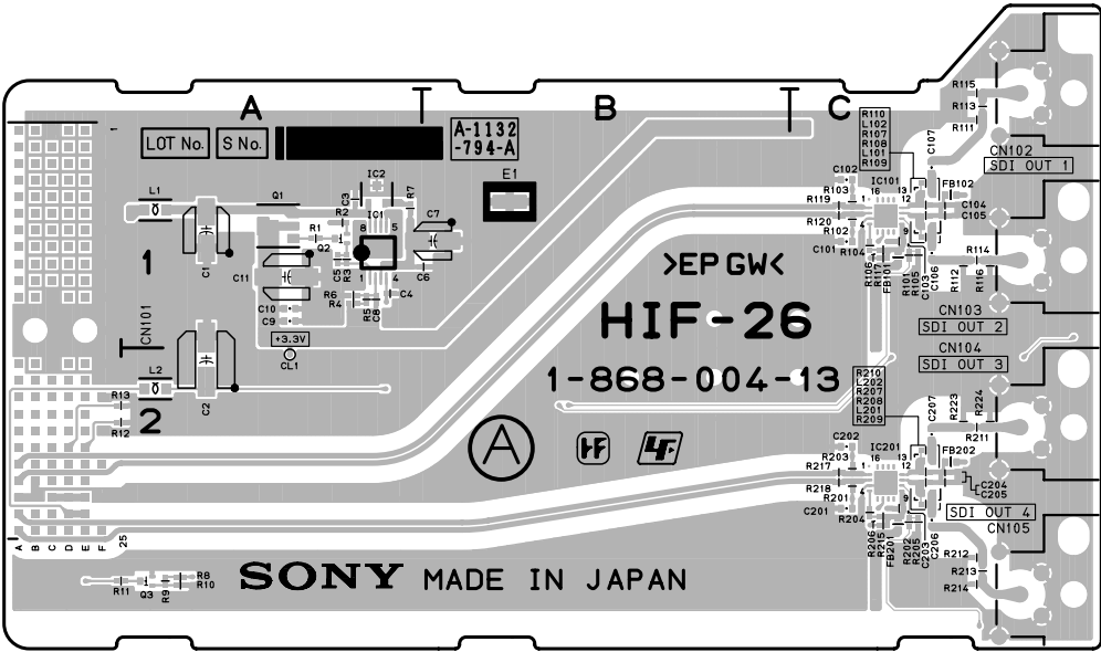
HIF-26 -A SIDE- SUFFIX: -13
