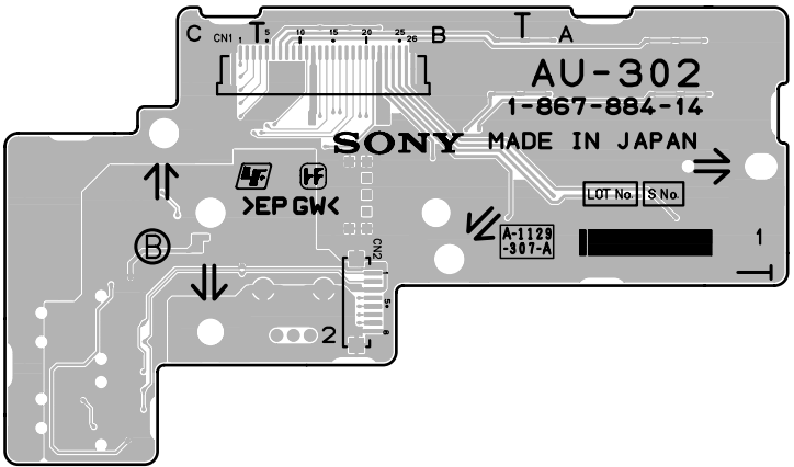
AU-302 -B SIDE- SUFFIX: -14
