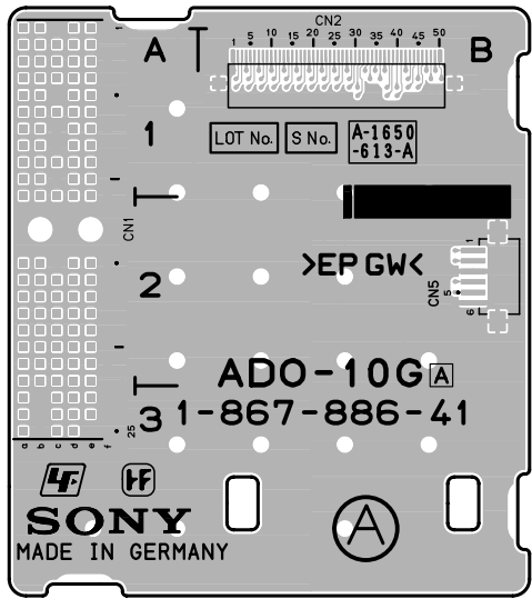
ADO-10GA -A SIDE- SUFFIX: -41
