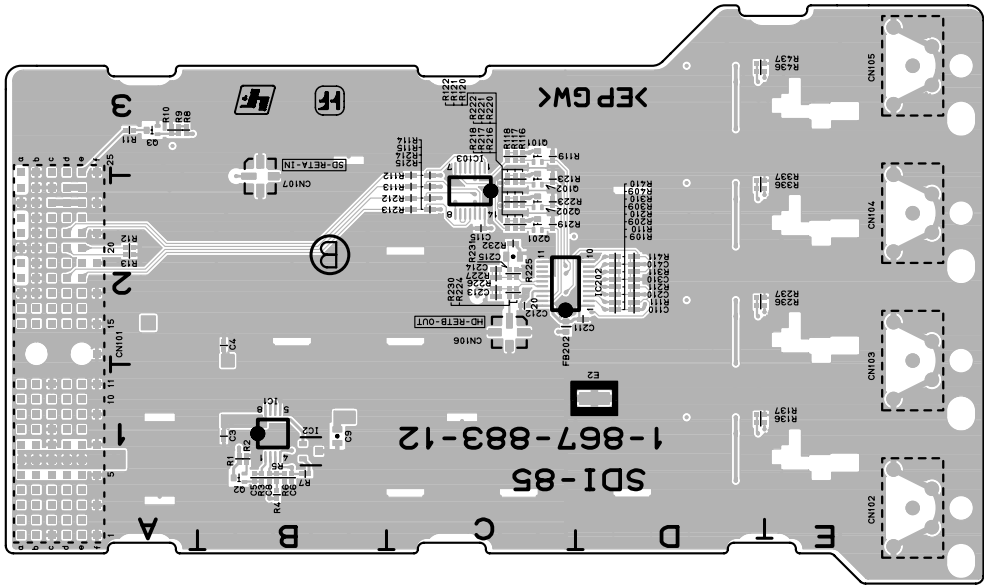
SDI-85 -B SIDE- SUFFIX: -12
