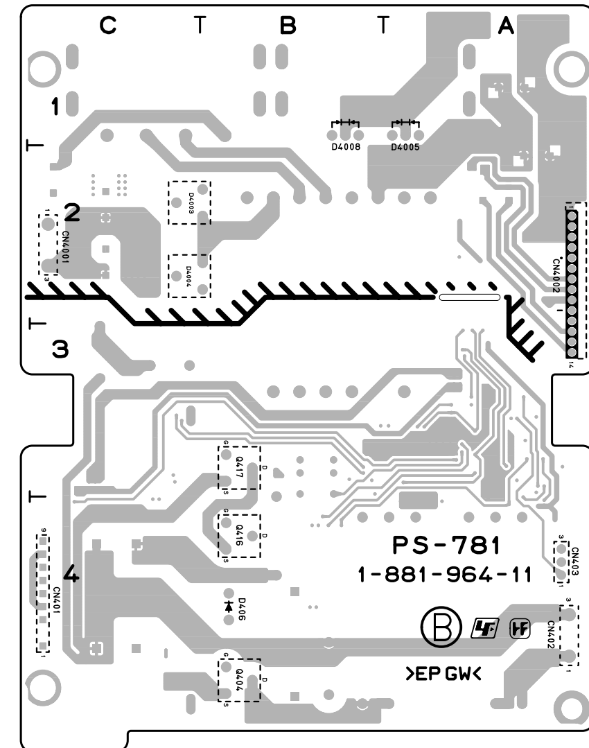
PS-781 -B SIDE- SUFFIX: -11
