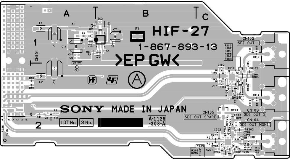
HIF-27 -A SIDE- SUFFIX: -13
