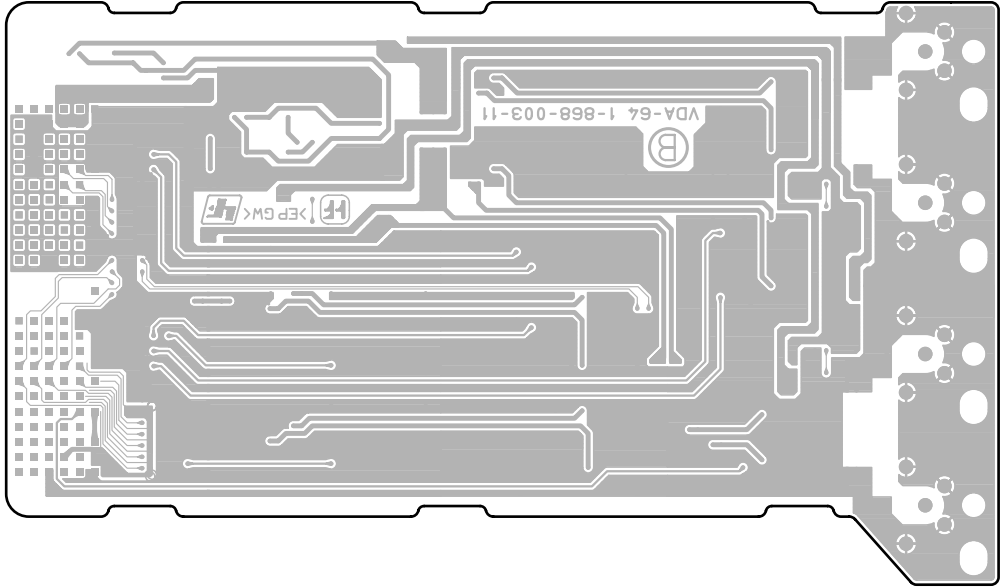
VDA-64 -B SIDE- SUFFIX: -12
