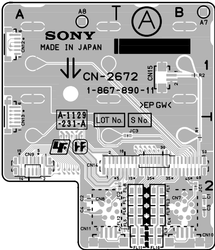
CN-2672G -A SIDE- SUFFIX: -11
