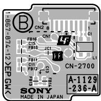
CN-2700 -B SIDE- SUFFIX: -12
