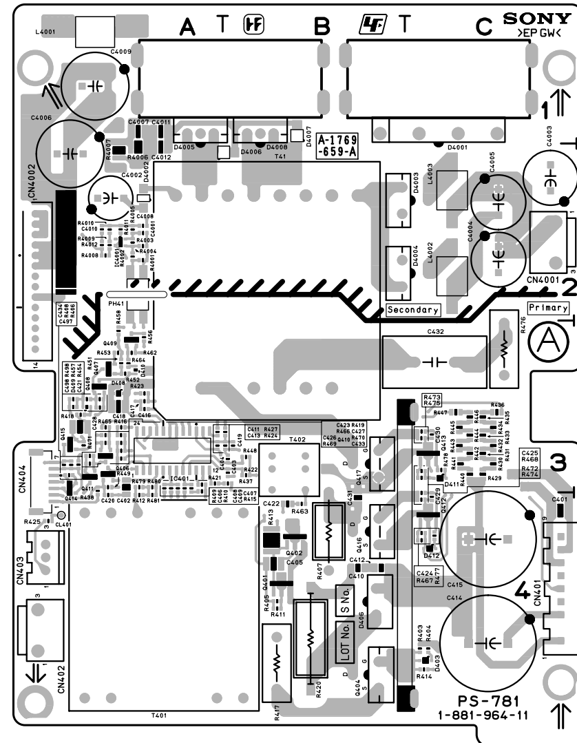
PS-781 -A SIDE-SUFFIX: -11
