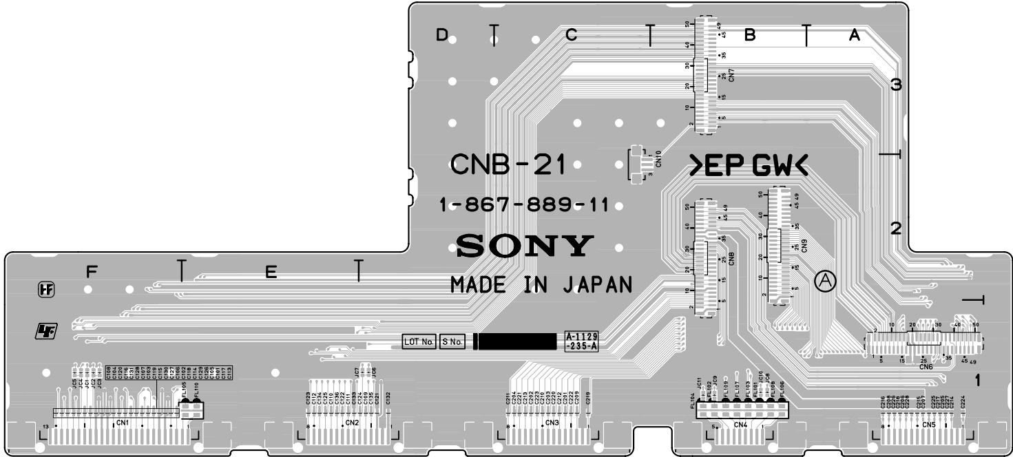
CNB-21G -A SIDE- SUFFIX: -11
