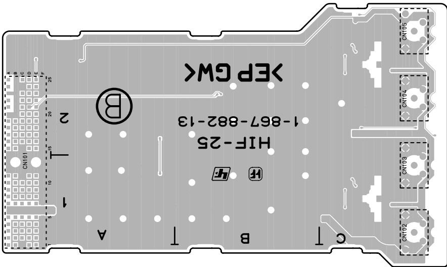
HIF-25 -B SIDE- SUFFIX: -13
