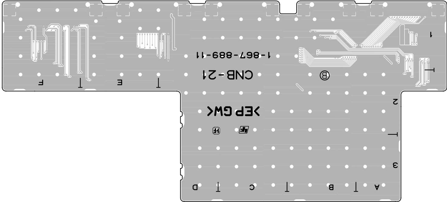
CNB-21G -B SIDE- SUFFIX: -11
