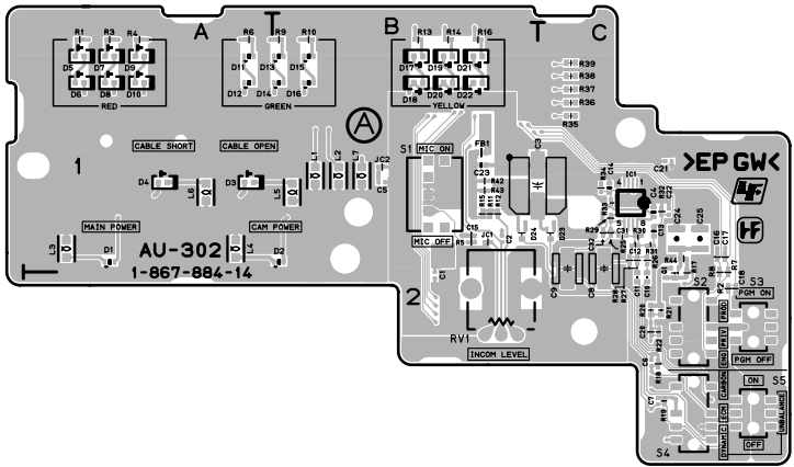
AU-302 -A SIDE- SUFFIX: -14
