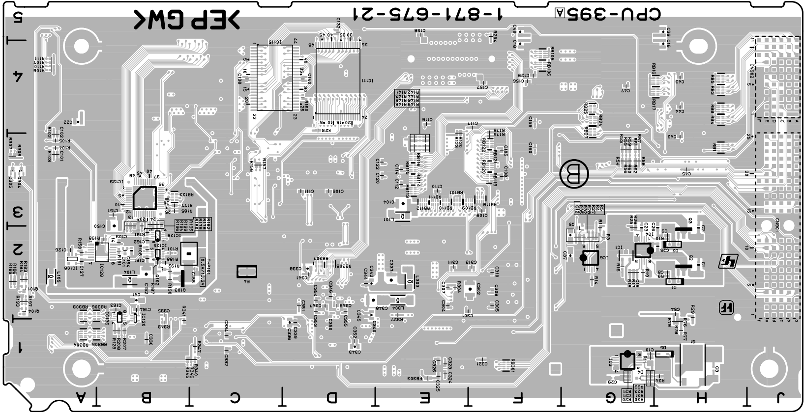
CPU-395A -B SIDE- SUFFIX: -21
