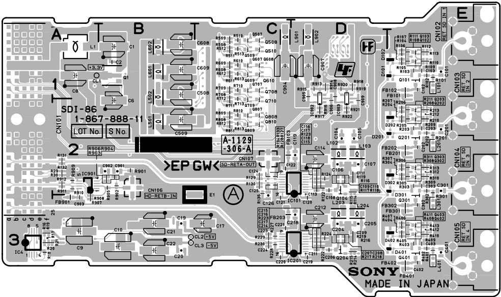
SDI-86G -A SIDE- SUFFIX: -11
