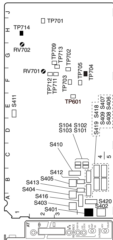
AT-167S board (A side and panel side)
