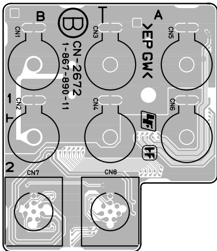
CN-2672G -B SIDE- SUFFIX: -11
