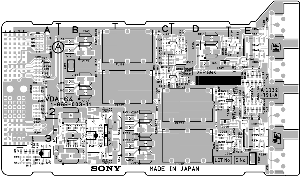
VDA-64 -A SIDE- SUFFIX: -12
