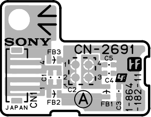
CN-2691 -A SIDE- SUFFIX: -11
