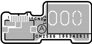
CN-2566 -A SIDE- SUFFIX: -11
