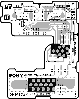
CN-2550 -B SIDE- SUFFIX: -13
