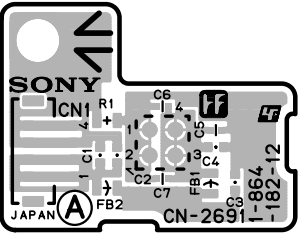
CN-2691 -A SIDE- SUFFIX: -12
