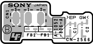
CN-2566 -B SIDE- SUFFIX: -11
