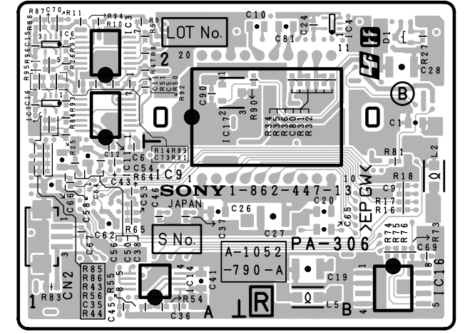
PA-306 -B SIDE- SUFFIX: -13
