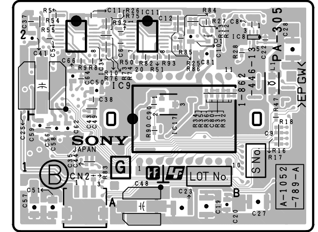
PA-305 -B SIDE- SUFFIX: -13
