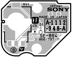
SE-804 (HKC-SV1) -B SIDE- SUFFIX: -11
