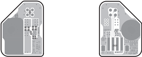
CN-3715 -A SIDE- SUFFIX: -11
