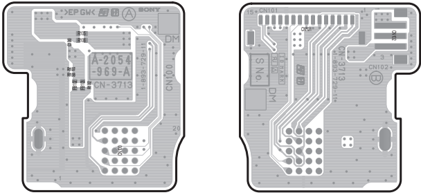
CN-3713 -A SIDE- SUFFIX: -11
