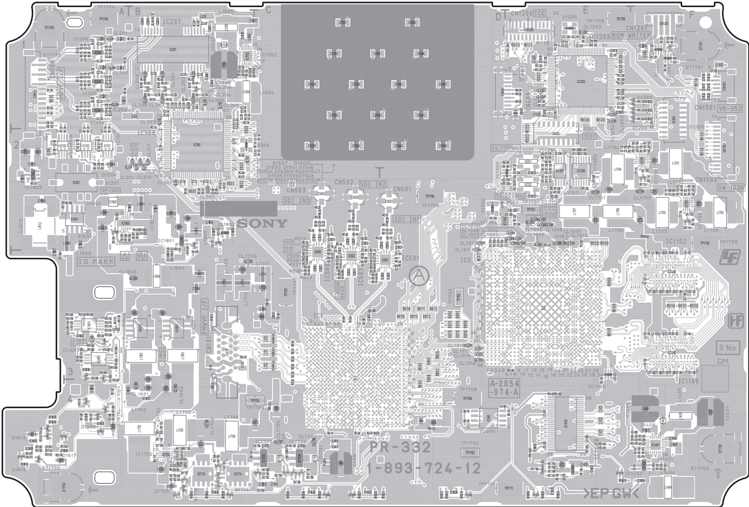
PR-332 -A SIDE- SUFFIX: -12
