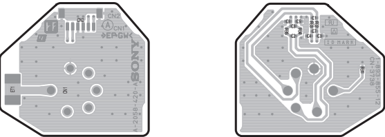
CN-3738 -A SIDE- SUFFIX: -12
