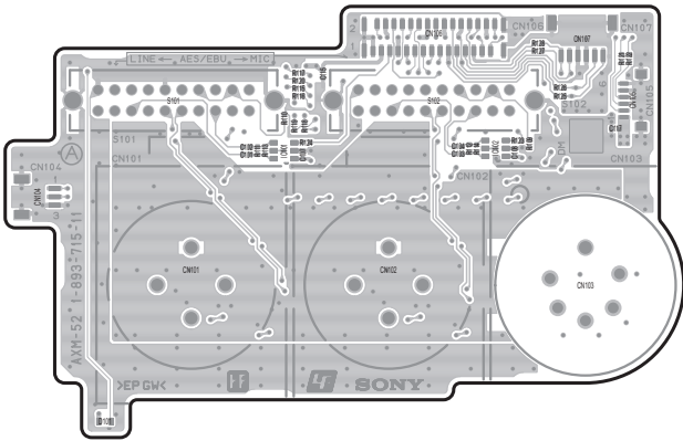
AXM-52 -A SIDE- SUFFIX: -11
