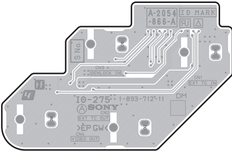
IO-275 -A SIDE- SUFFIX: -11
