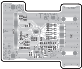
DIF-232 -A SIDE- SUFFIX: -11
