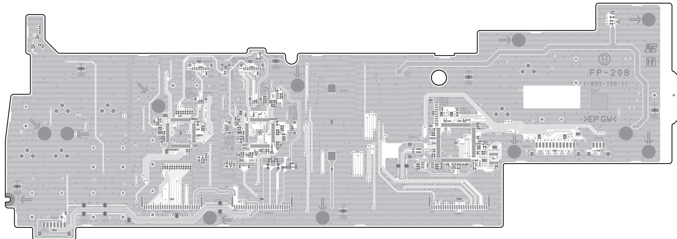
FP-208 -A SIDE- SUFFIX: -11
