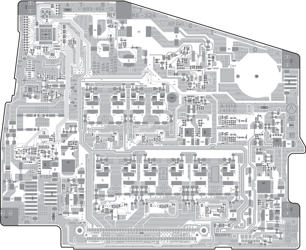
RE-326 -A SIDE- SUFFIX: -12
