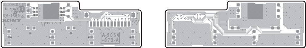
SW-1650 -A SIDE- SUFFIX: -11
