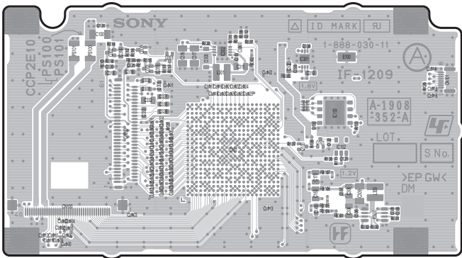
IF-1209 -A SIDE- SUFFIX: -11
