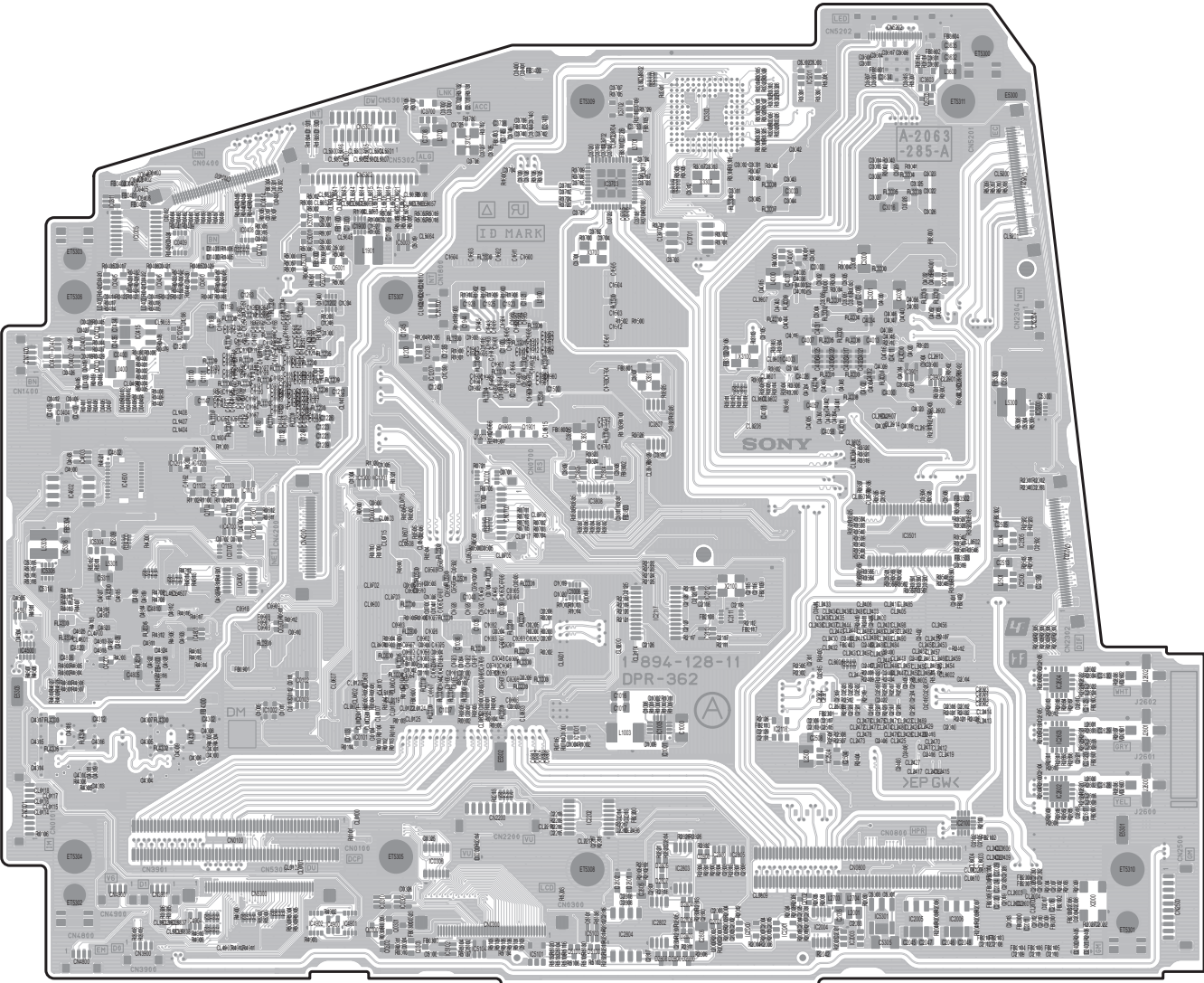
DPR-362 -A SIDE- SUFFIX: -12
