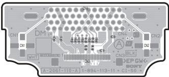
CI-50 -A SIDE- SUFFIX: -11
