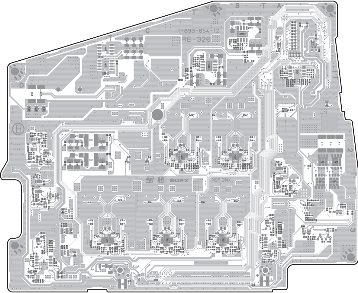
RE-326 -B SIDE- SUFFIX: -12
