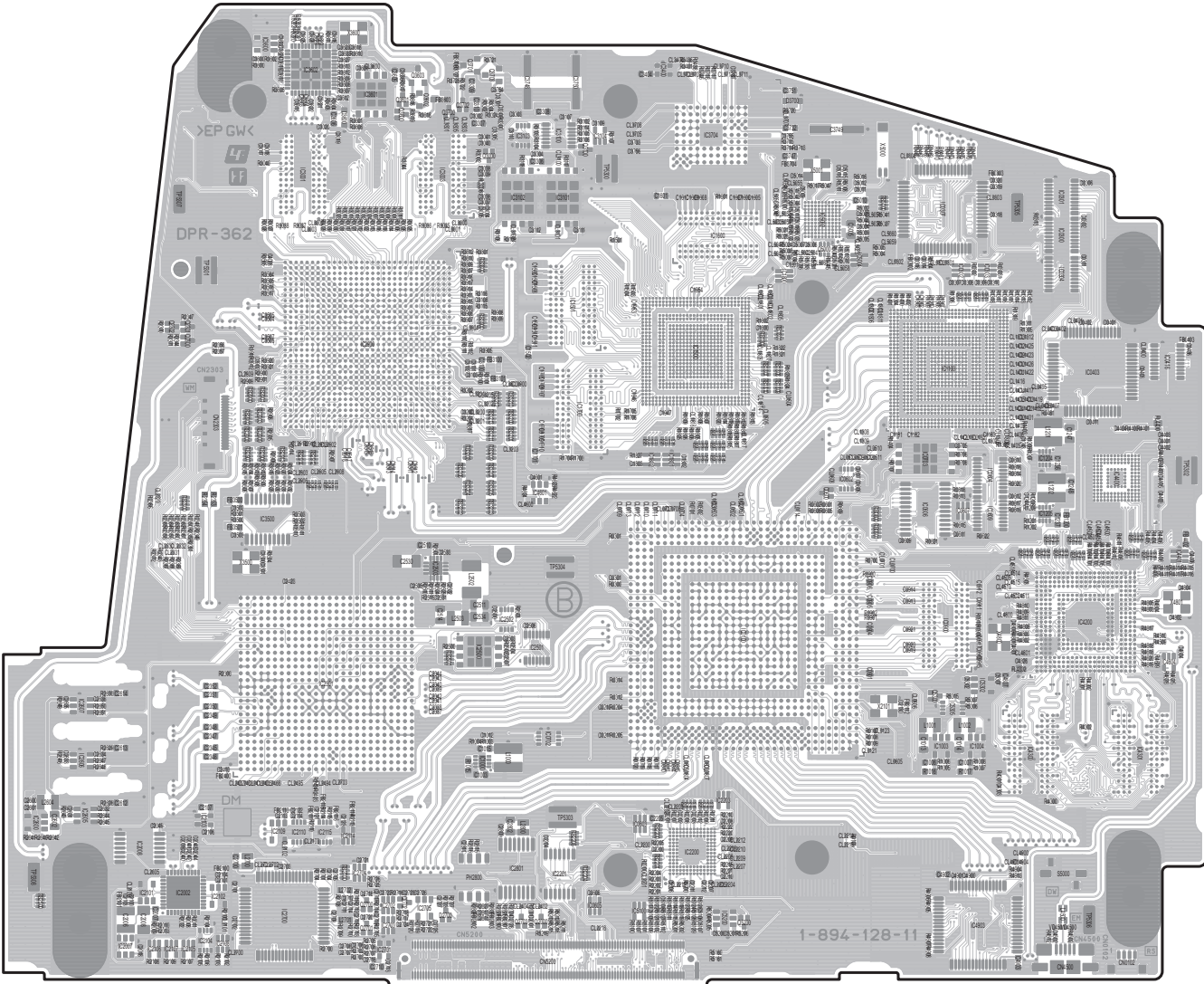
DPR-362 -B SIDE- SUFFIX: -11
