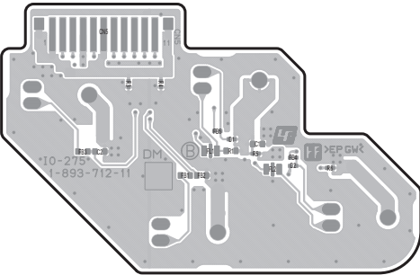
IO-275 -B SIDE- SUFFIX: -11
