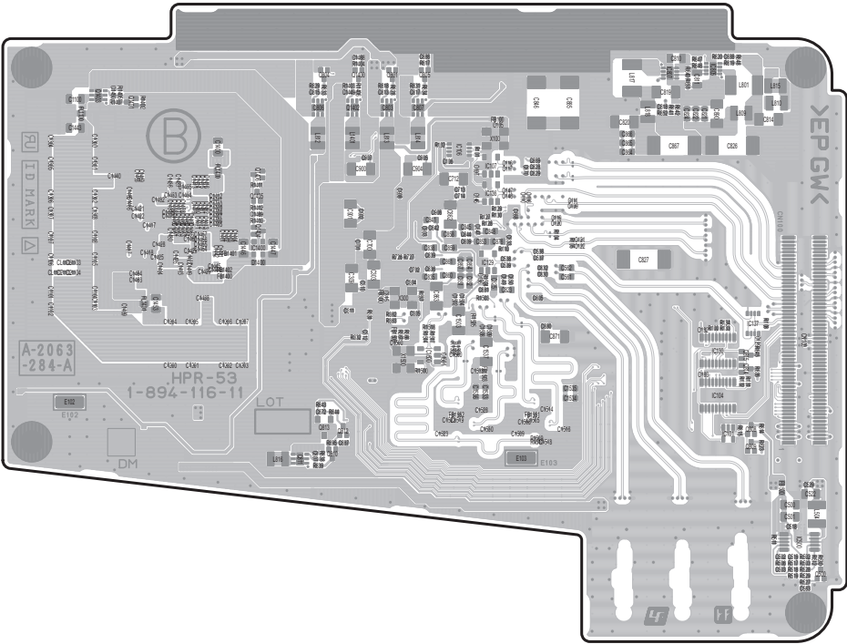
HPR-53 -B SIDE- SUFFIX: -11
