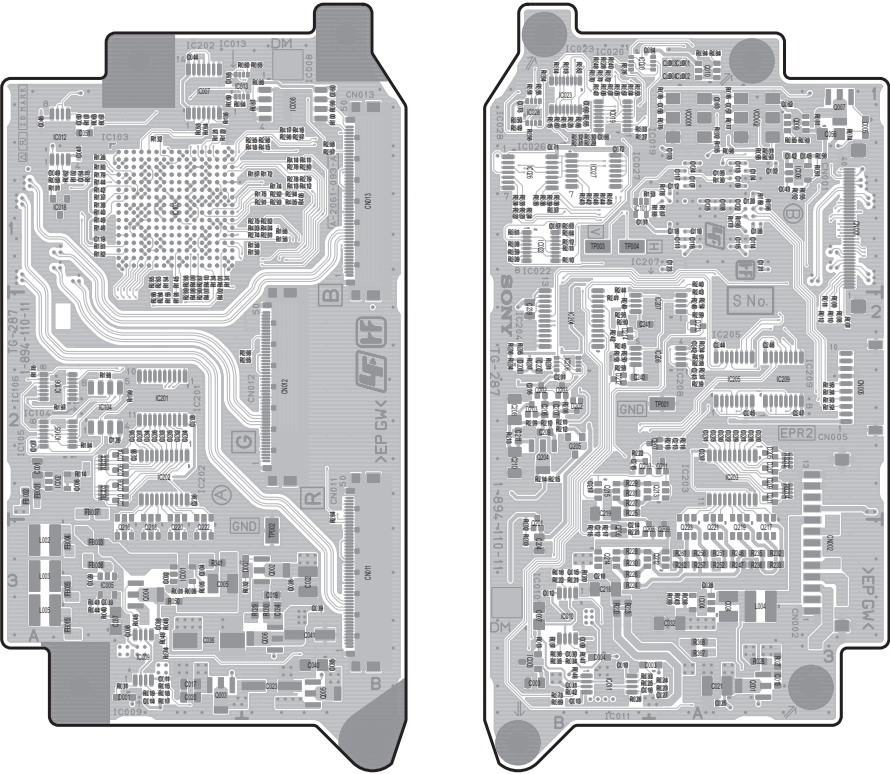
TG-287 -A SIDE- SUFFIX: -11
