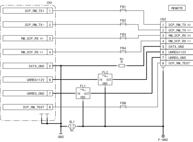
RM-246 BOARD NO. 1-893-856-11 RM-246_1
