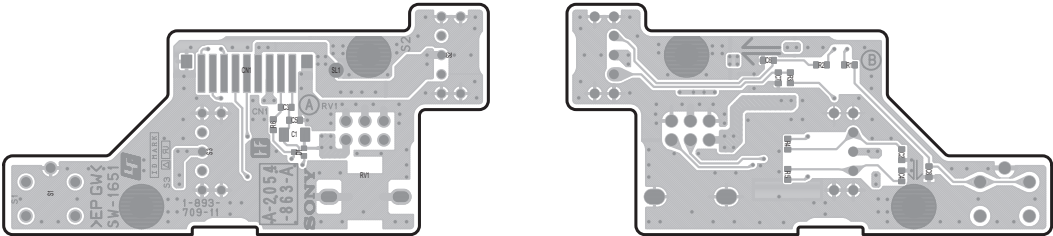
SW-1651 -A SIDE- SUFFIX: -11
