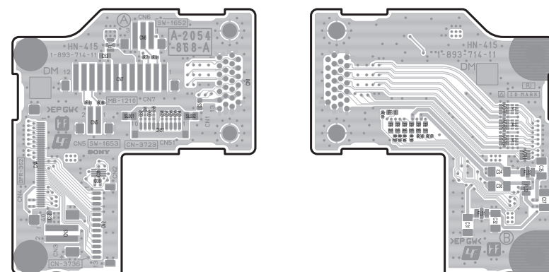
HN-415 -A SIDE- SUFFIX: -11
