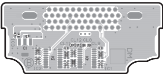
CI-50 -B SIDE- SUFFIX: -11
