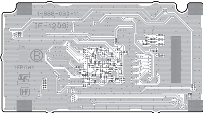
IF-1209 -B SIDE- SUFFIX: -11
