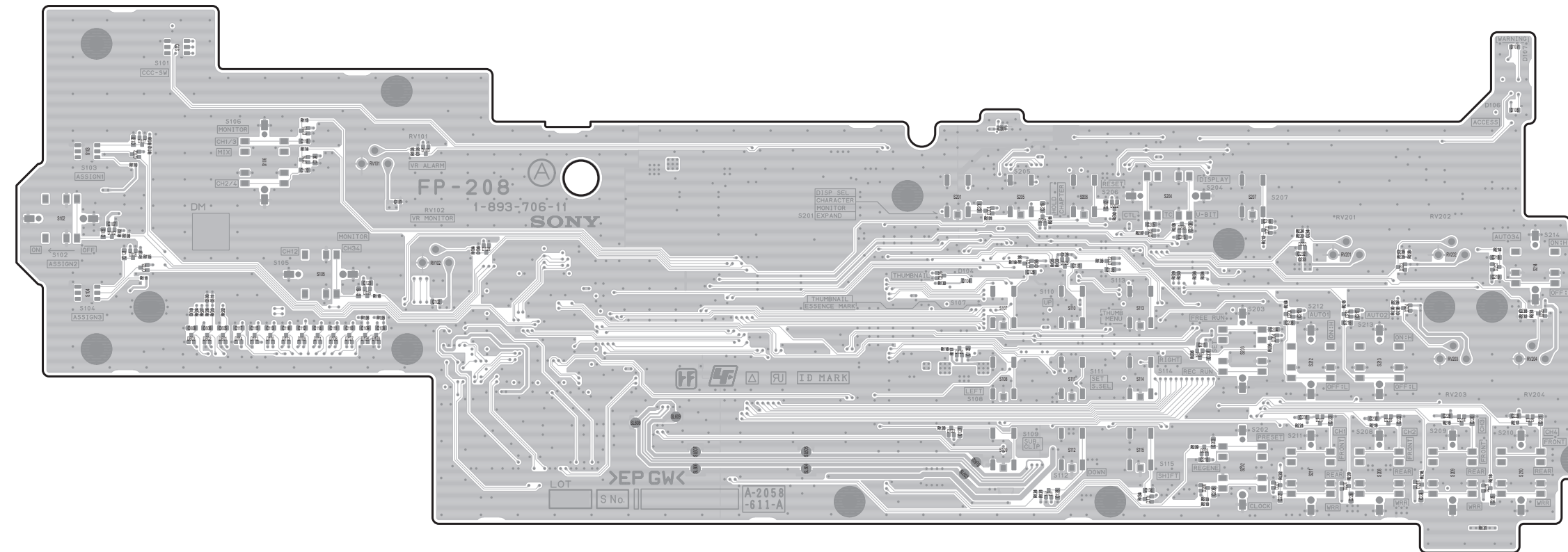
FP-208 -B SIDE-SUFFIX: -11
