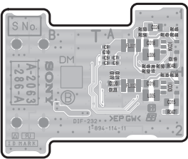
DIF-232 -B SIDE- SUFFIX: -11
