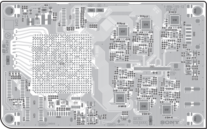
DCP-67 -A SIDE- SUFFIX: -12
