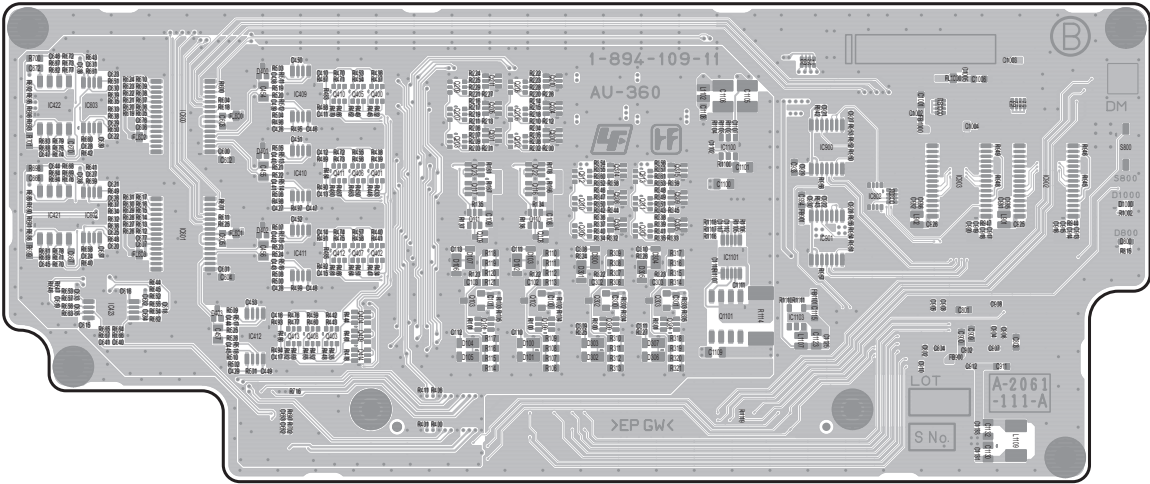
AU-360 -B SIDE- SUFFIX: -11
