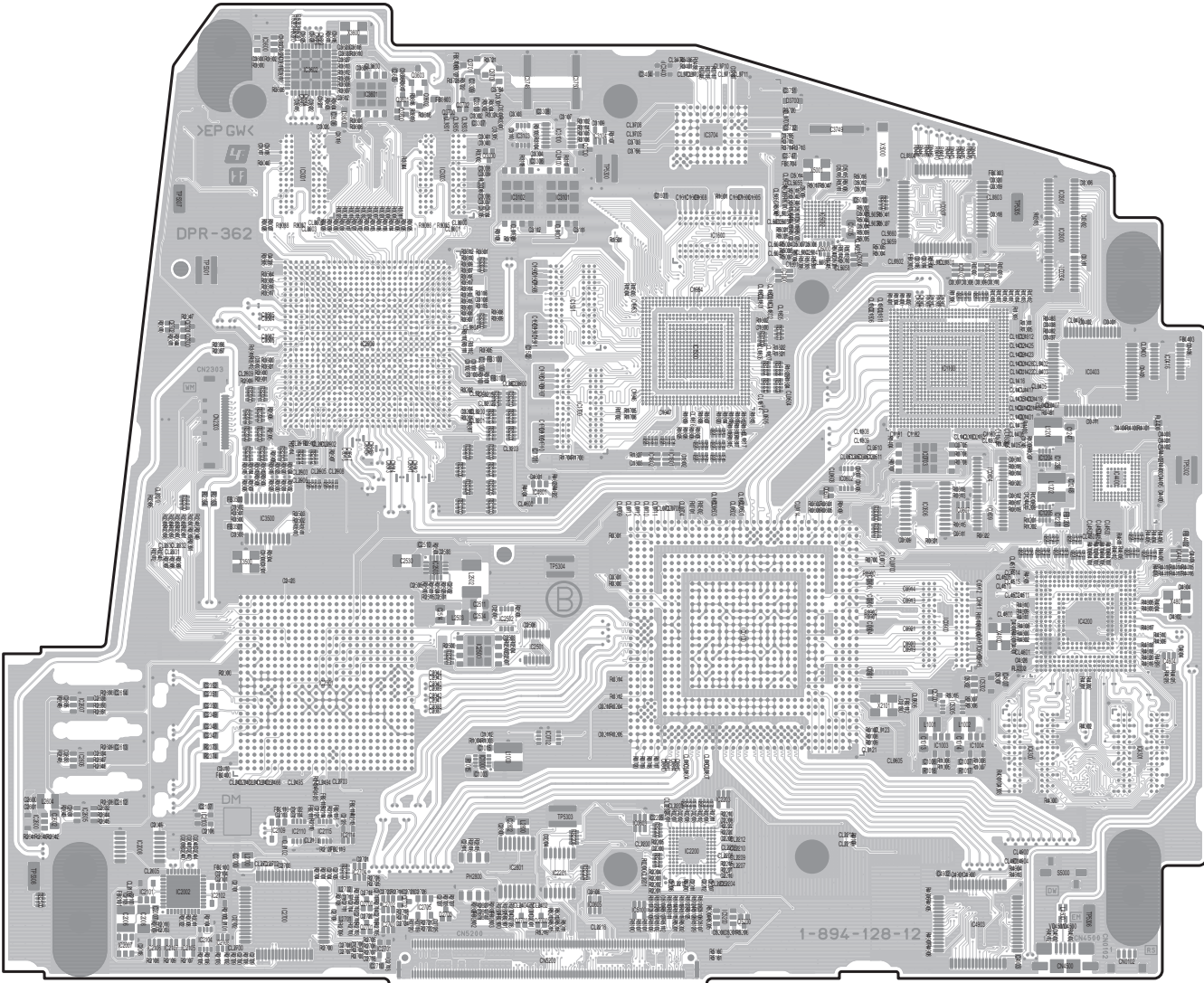
DPR-362 -B SIDE- SUFFIX: -12
