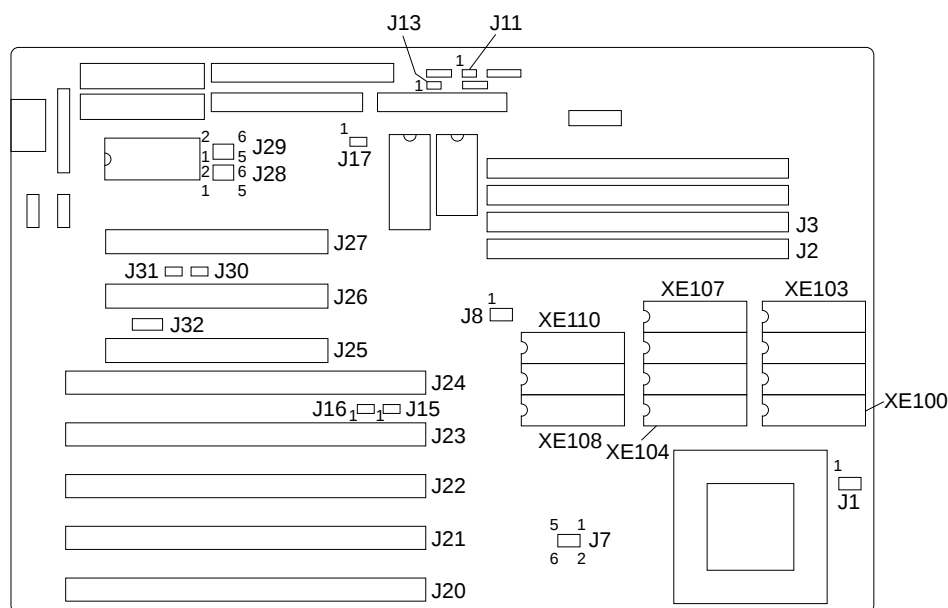
PCI Mother Board (AXPpci33)
