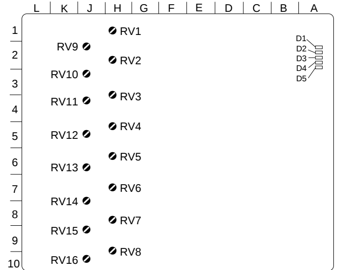
DAC-19 BOARD (A-side)
