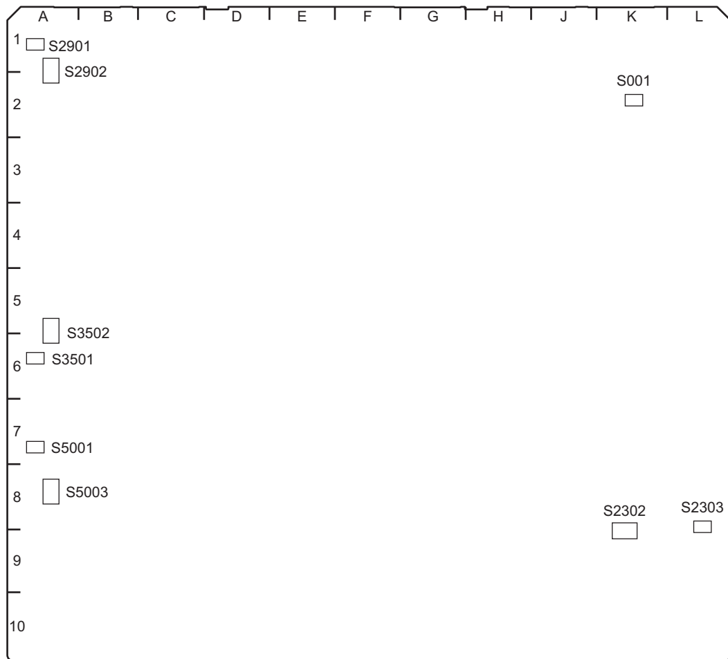
DIO-101 board (Side A)
