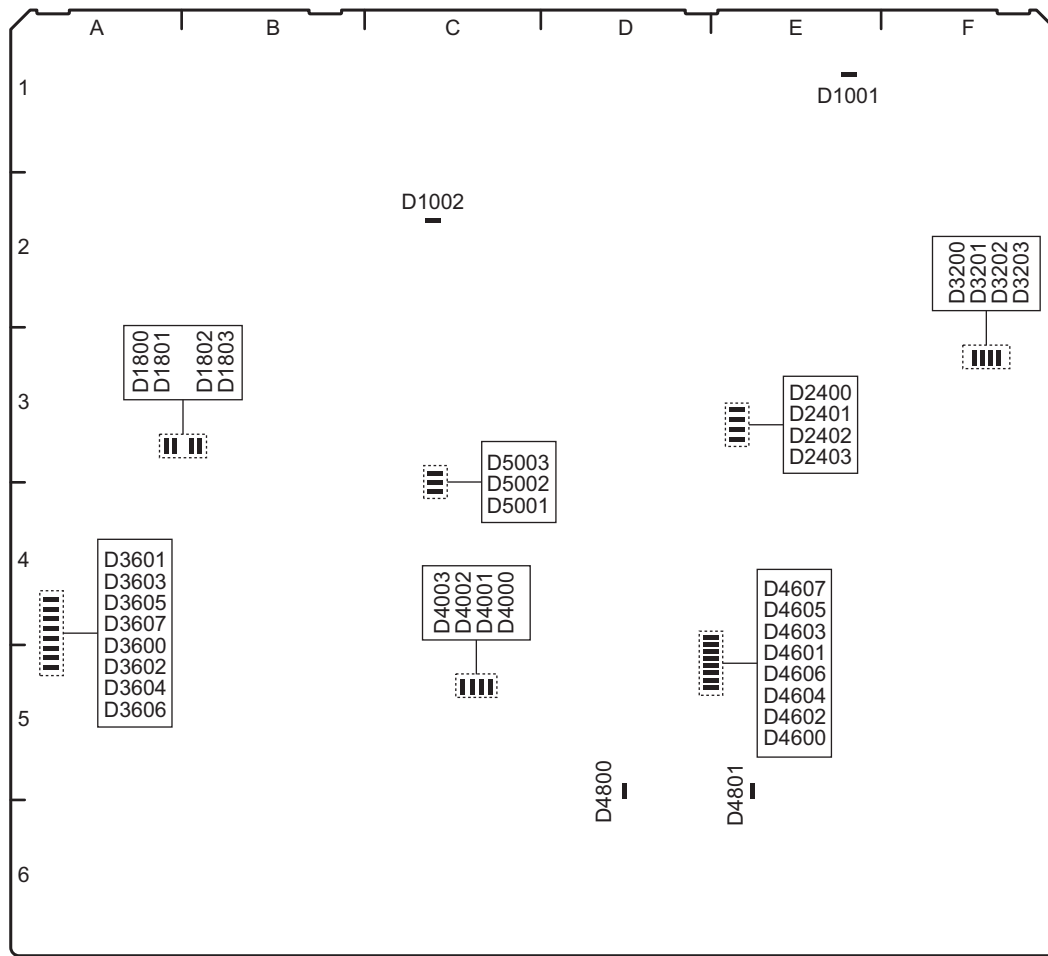
DM-155 board (Side A)
