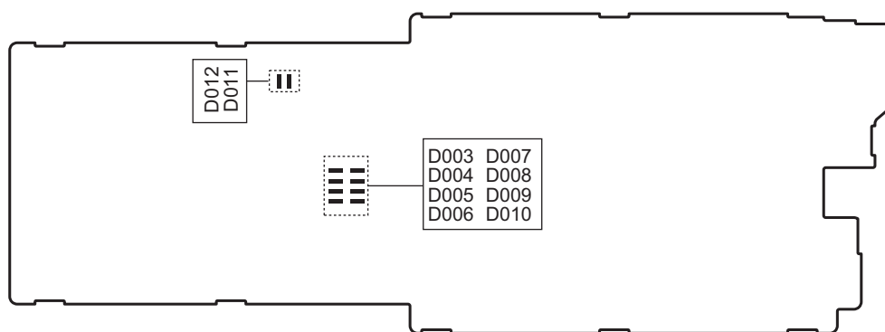
HP-175 board (Side A)
