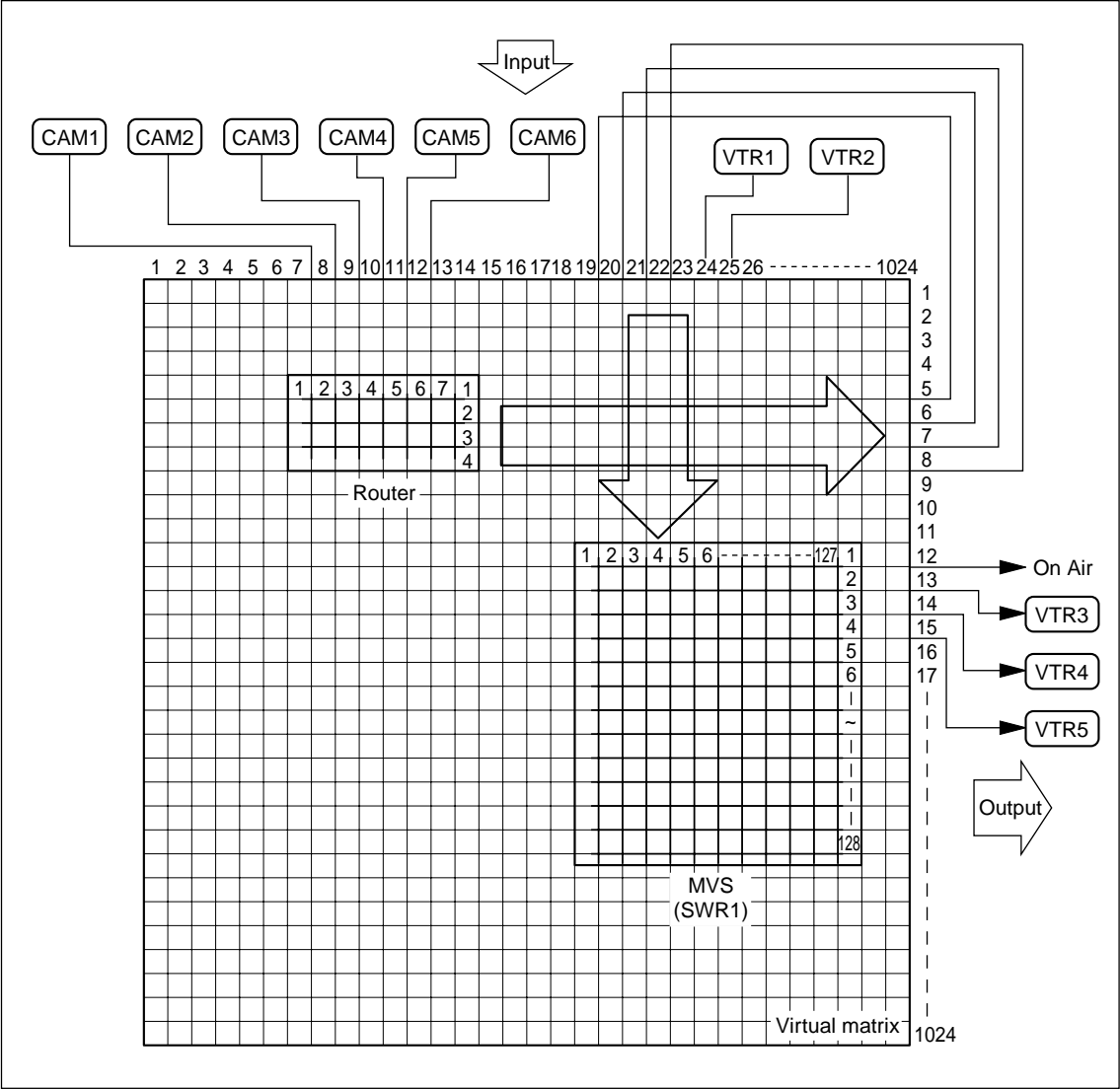
Setting the crosspoints connections (wiring)
