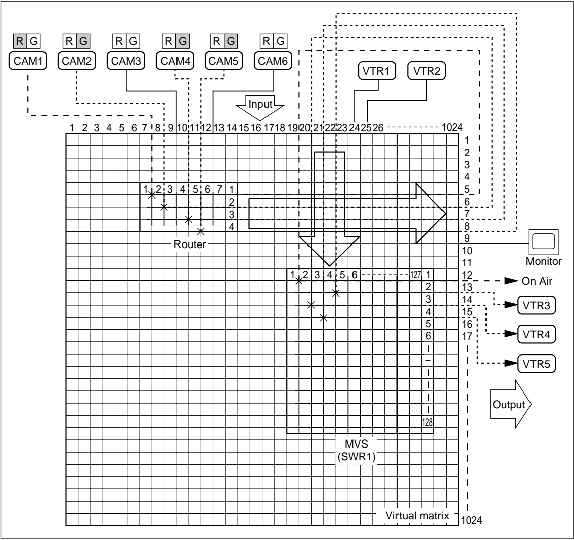
System connection diagram (example)
