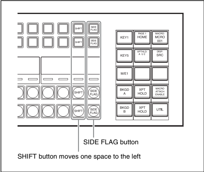
Cross-point control block
