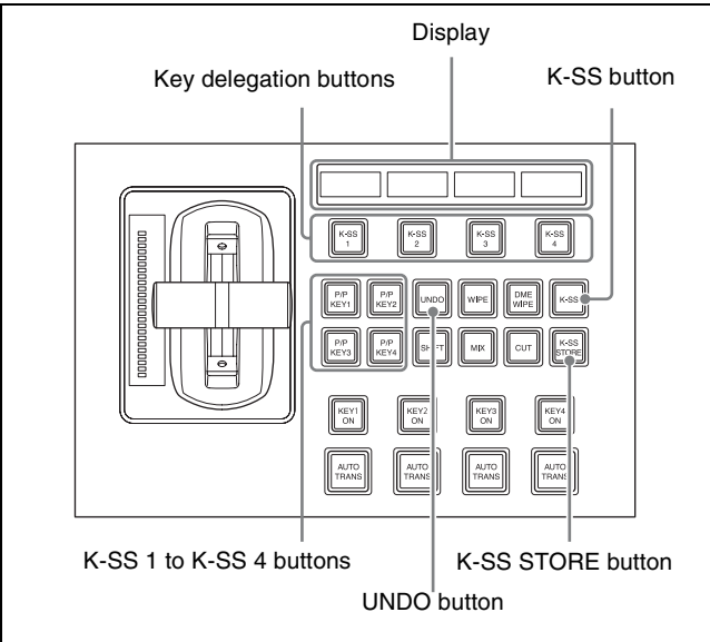
Key fader control block
