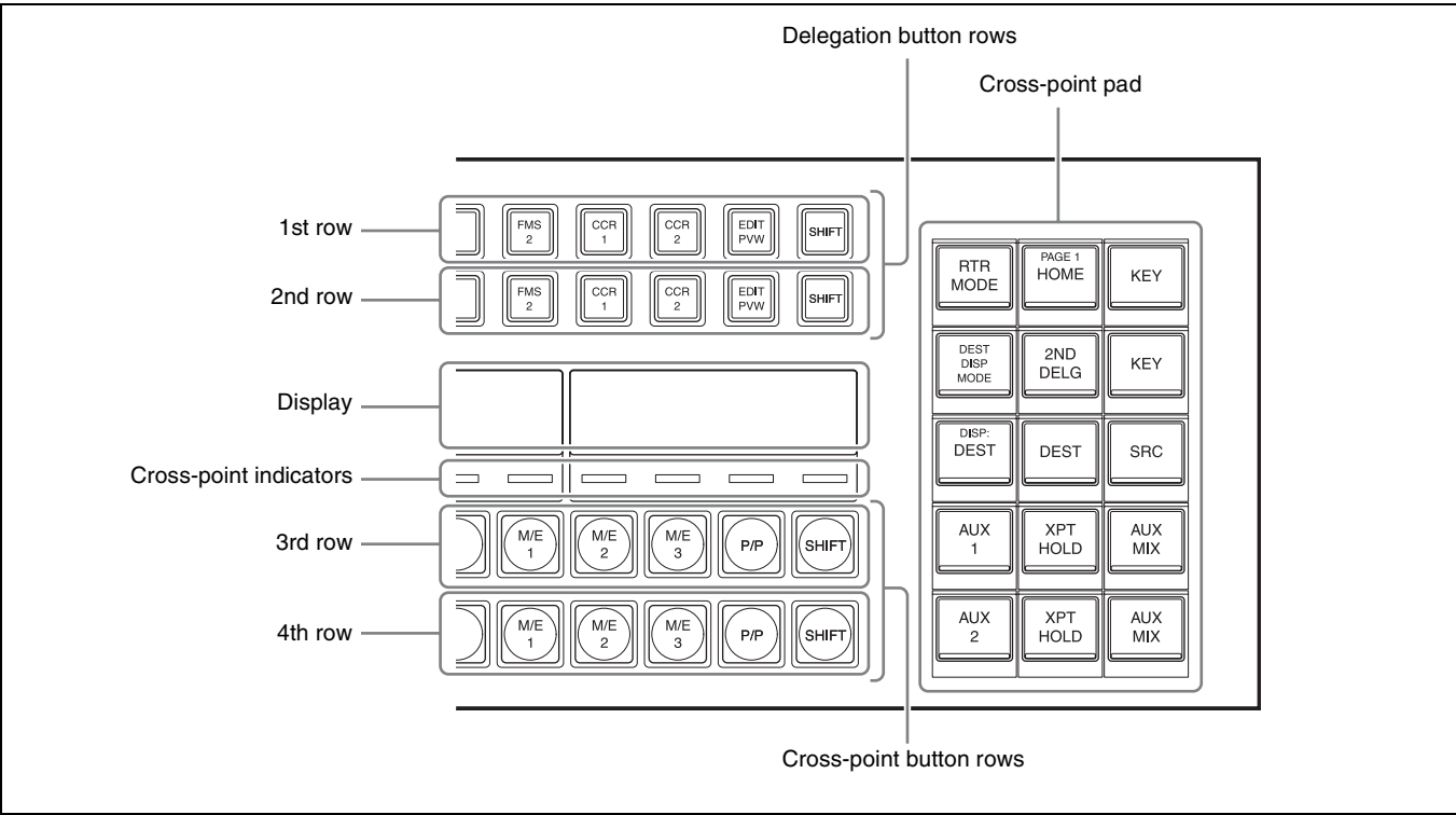
AUX bus control block (AUX bus operation mode)
