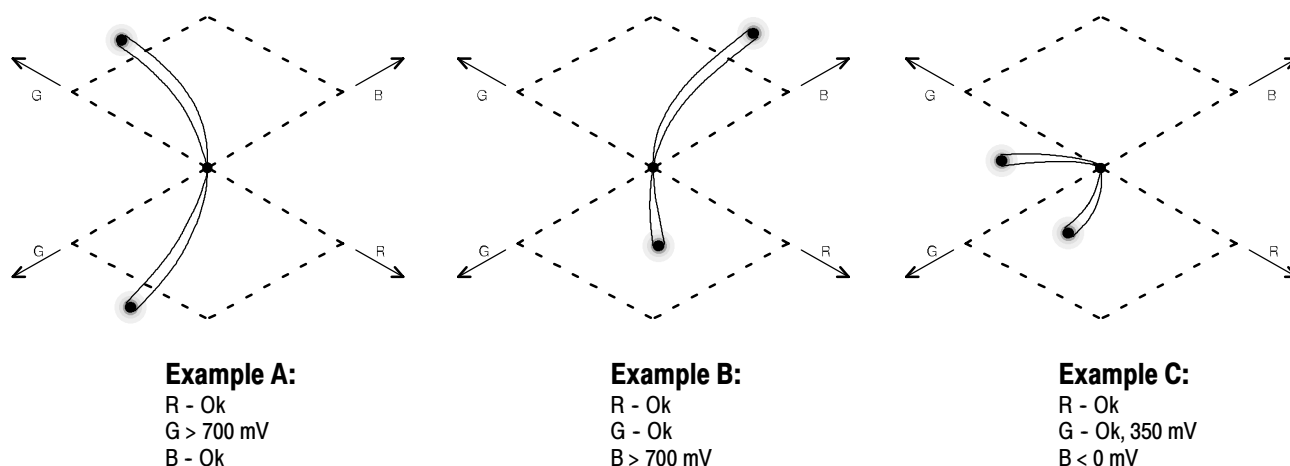
Figure 3-10: Out-of-gamut signals on a Diamond display
