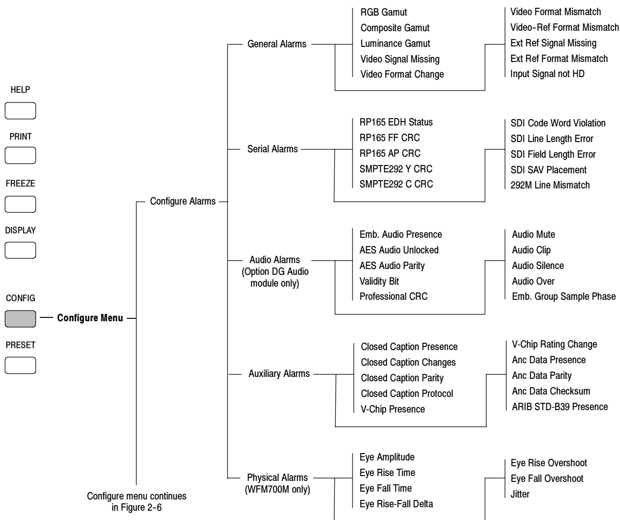
Figure 2-5: Configuration menu diagram - part 1
