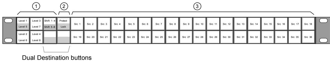
Figure 4-1 UCP 36/8 Panel
