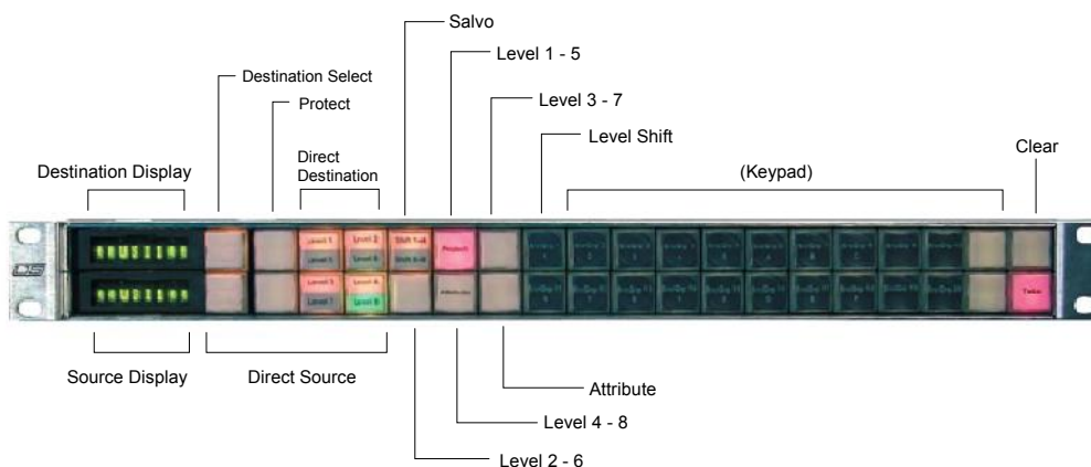
Figure 3-1. UCP 2 Panel
