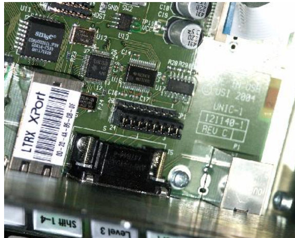
Figure 2-8. RS-422 Operation
