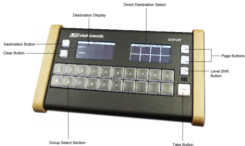
Figure 7-2. UCP-DT Panel Selections
