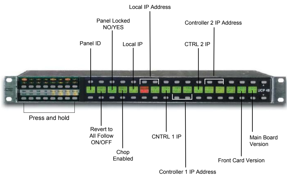
Figure 5-15. LCD Displays
