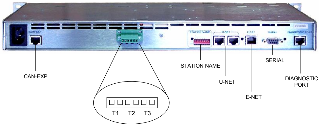
Figure 6-2. Panel Rear
