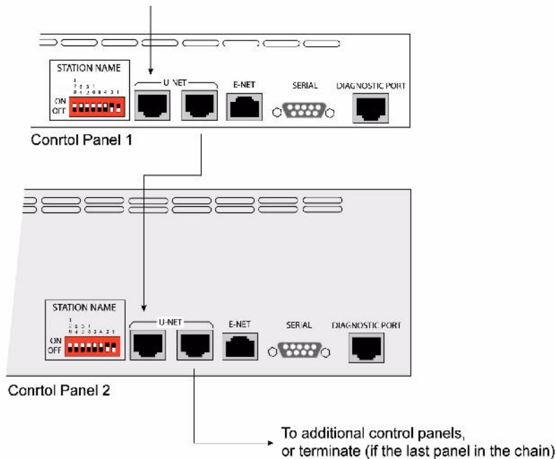
Figure 2-4. U-Net Interconnection Diagram
