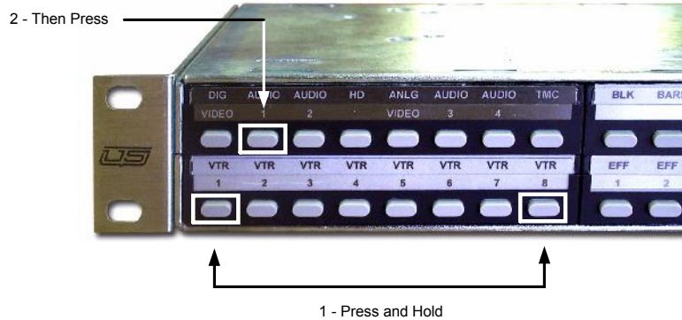
Figure 5-10. Panel Lock button combination
