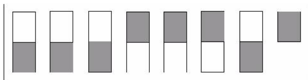
Dip Switch Setting (rear)
