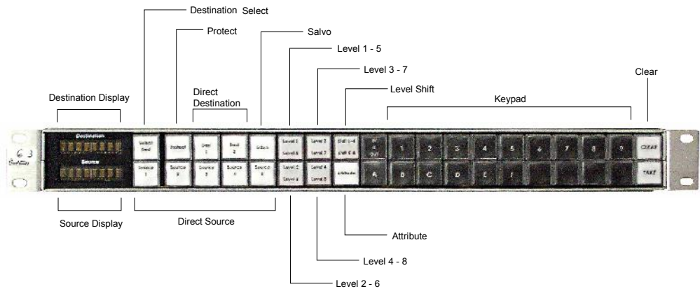
Figure 4-1. UCP 1 Panel
