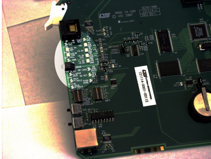
FIGURE 4-17. FIGURE 4-17. SCX-400 Control Board View
