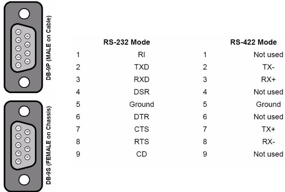
FIGURE 3-3. Pinout detail
