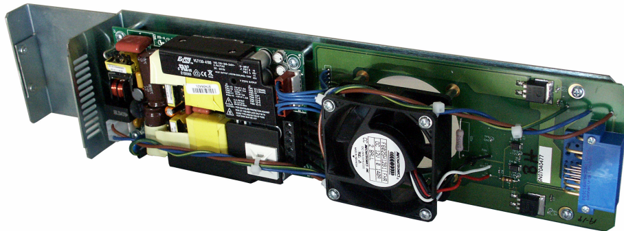
FIGURE 4-27. Fan device location
