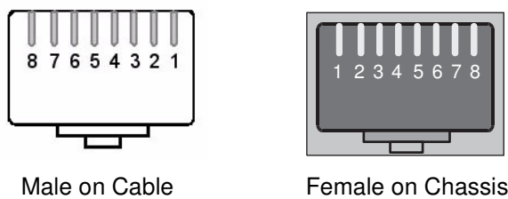
FIGURE 3-4. Pin-outs for the RJ-45 U-Net connector
