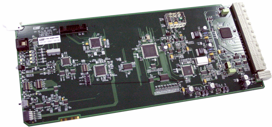
FIGURE 2-9. Audio Crosspoint
