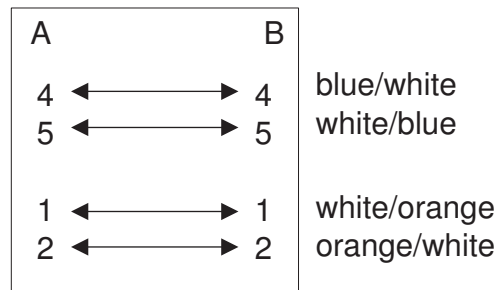
FIGURE 3-6. U-Net Cable Pairs and Pin-out
