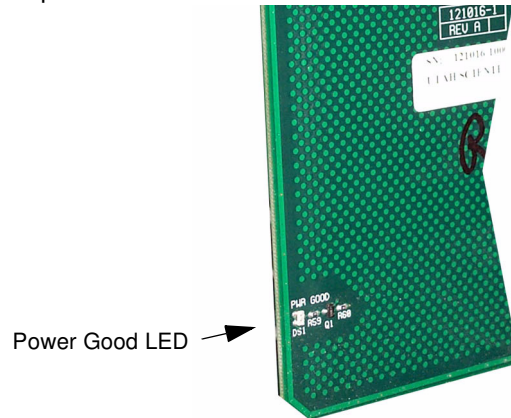
FIGURE 4-11. SD and HD Output Power Good LED
