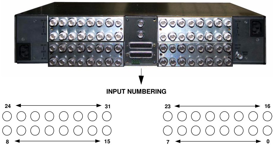
FIGURE 2-12. Video and Unbalanced Audio Input Connector Matrix
