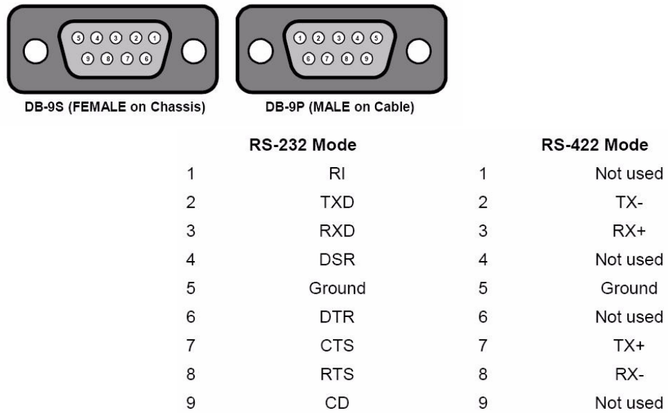
FIGURE 3-7. Pinout detail
