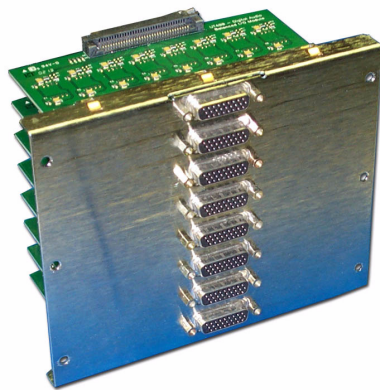
FIGURE 4-23. D-sub assembly
