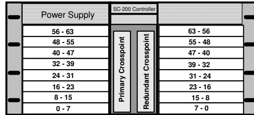
Input Output Single Power Supply, SC-200 Control, Redundant crosspoint cards
