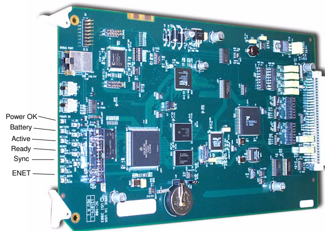
Board placement within the 64x64 router
