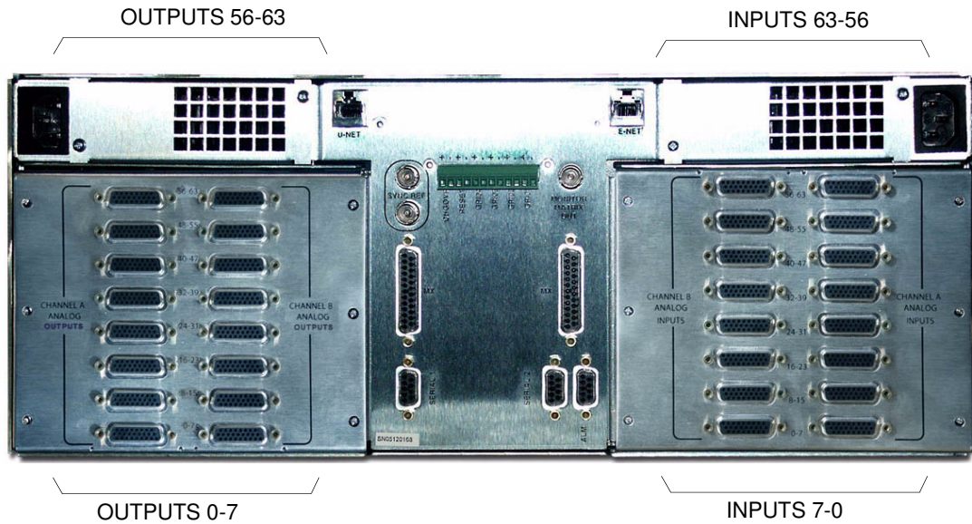
FIGURE 2-11. Utah-400 Analog Audio Backplane
