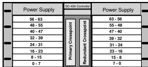
Input Output Dual Power Supply, SC-400 Control, Redundant crosspoint cards
