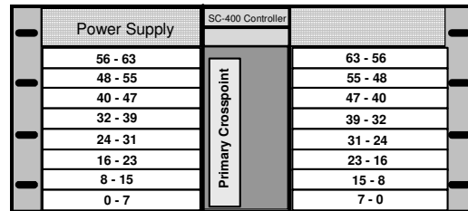
Input Output Single Power Supply, SC-400 Control, Single crosspoint card
