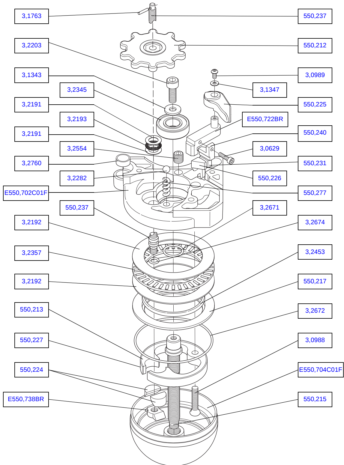
Fig 1.5 Pan Drag Assembly
