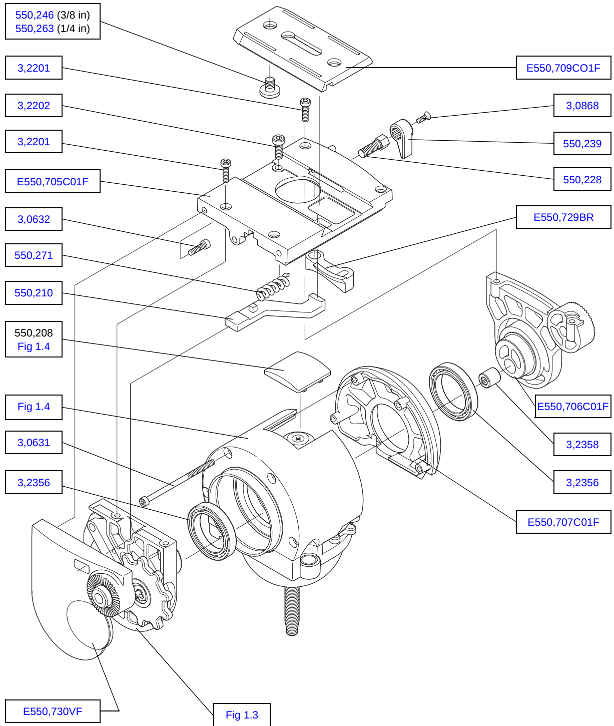
Fig 1.2 Platform and Side Plates
