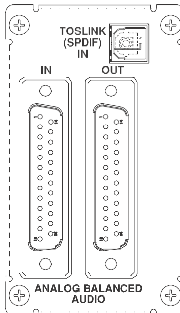
Figure 6-7 Analog I/O and SPDIF TOSLINK Panel Adaptor and Cover Plate
