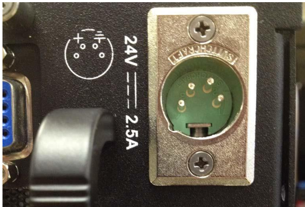
Figure 6–9 DC 4-Pin Power Connector
