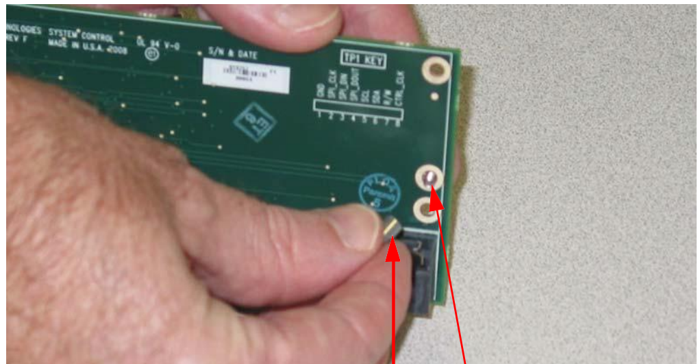
Standoff Screw from the Other Side
