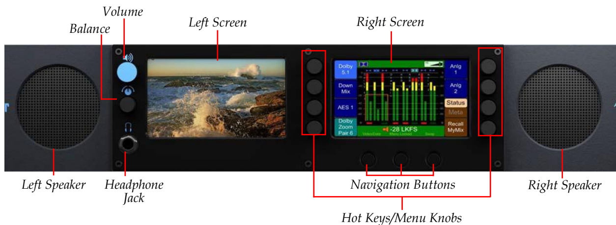
Figure 1–1 Front Panel Layout
