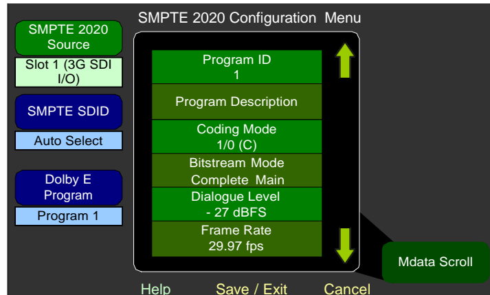
Figure 1–11 SMPTE 2020 Configuration Menu
