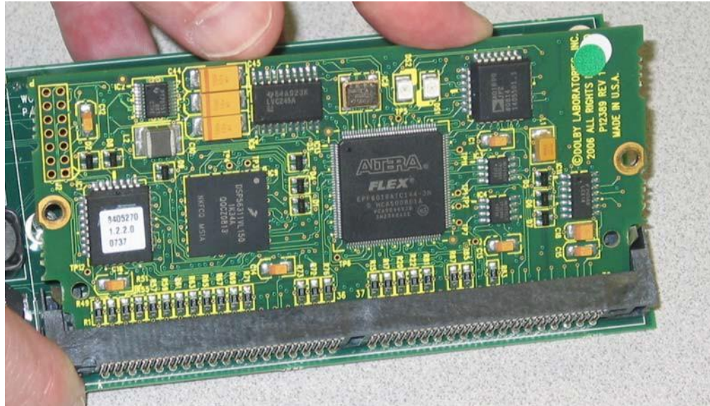
Figure 6-17 Insert Dolby D/E/DD+ Card
