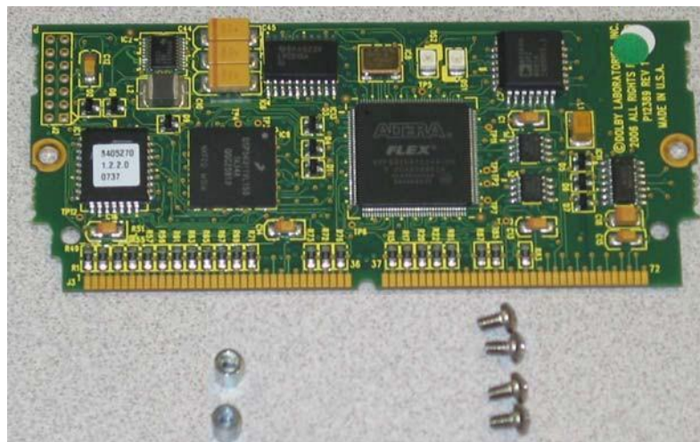
Figure 6–14 Dolby D/E/DD+ Option Kit
