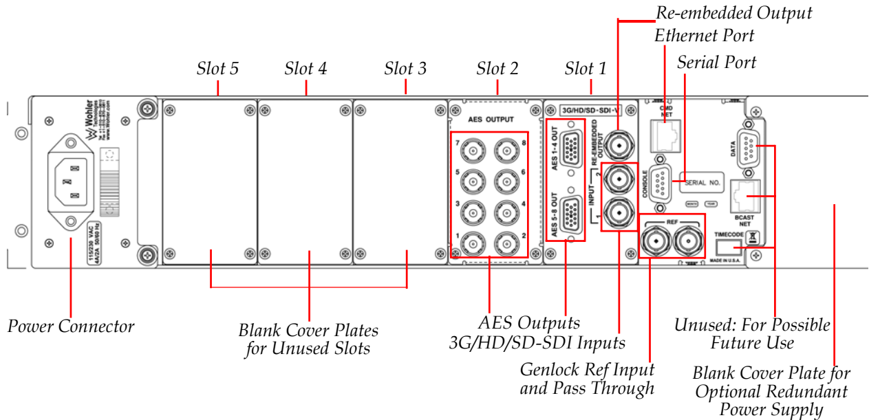
Figure 2-1 Typical Back Panel Layout
