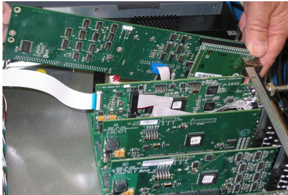
Figure 6–20 Re-Seat System Control Board
