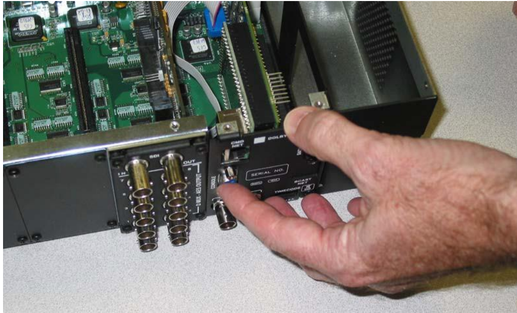
Figure 6-21 Replace Rear Panel
