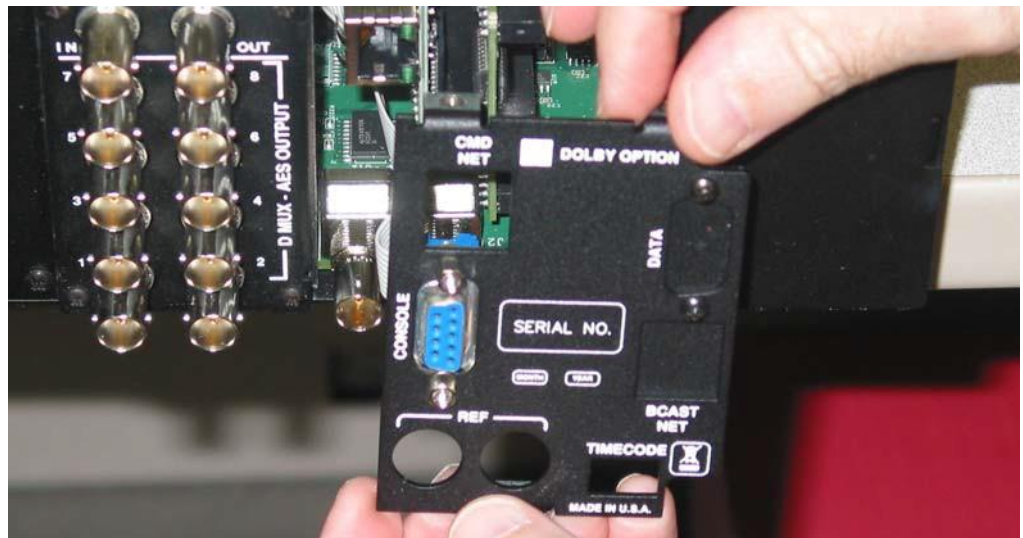
Figure 6-12 Remove System Control Board's Rear Panel Adaptor
