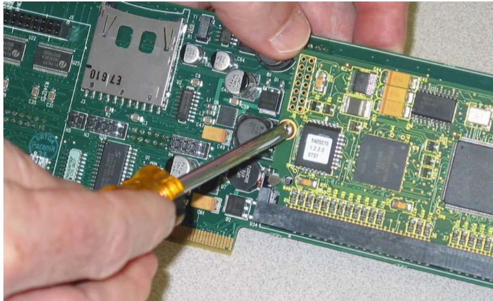
Figure 6-18 Tighten First Standoff Screw
