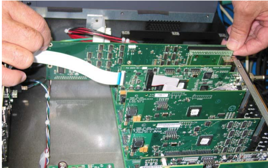
Figure 6–13 Remove System Control Board
