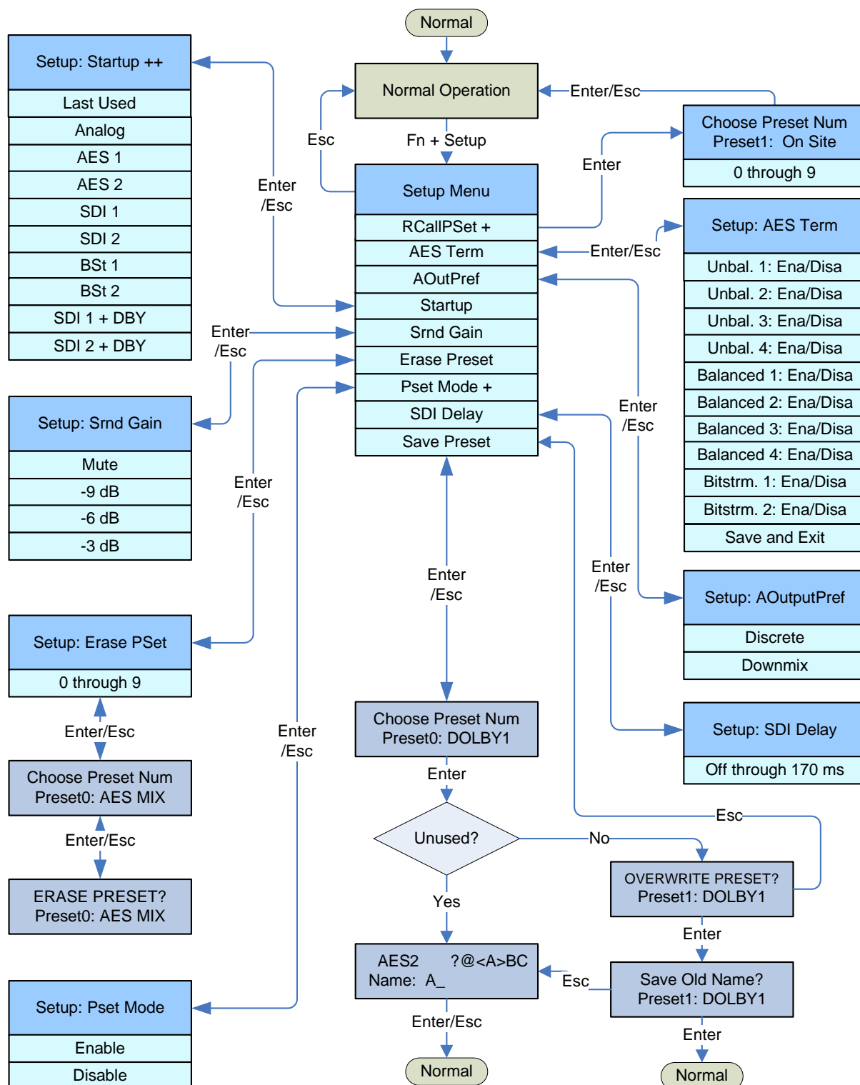
Figure 6–1 Setup Menu Tree
