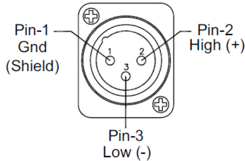
Figure 1-13 XLR-M Pin-Out
