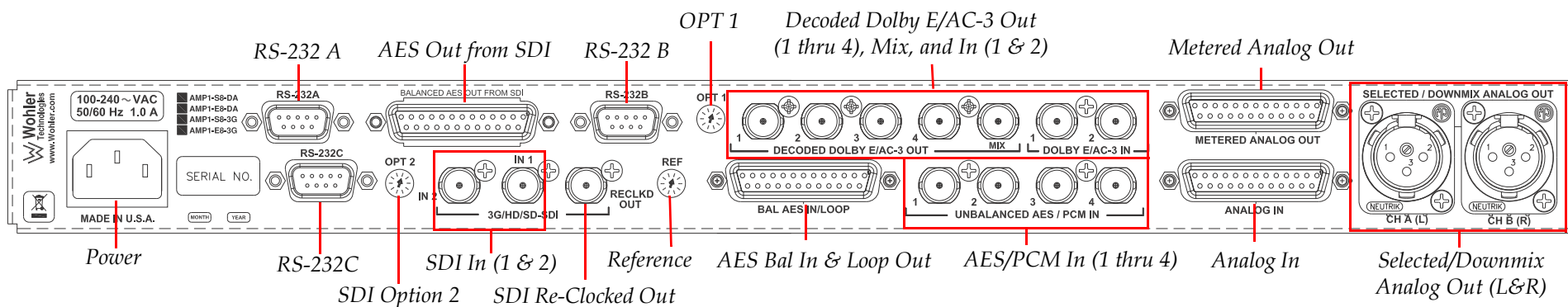
Figure 1–8 The AMP2-E8-MDA-3G Rear Panel
