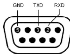
Figure 1-14 RS-232 Pin-Out
