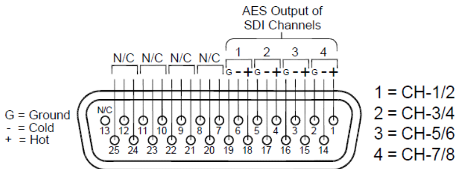
Figure 1–12 AES Balanced Out from SDI DB-25 Pin-Out
