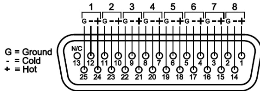
Figure 1-9 Analog Input Connector Pin-Out
