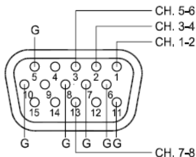
Figure 1–11 AES Unbalanced Out from SDI HD-15 Pin-Out
