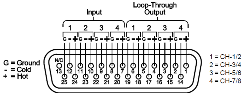
Figure 1–10 AES/PCM Input and Loop-Through DB-25 Pin-Out
