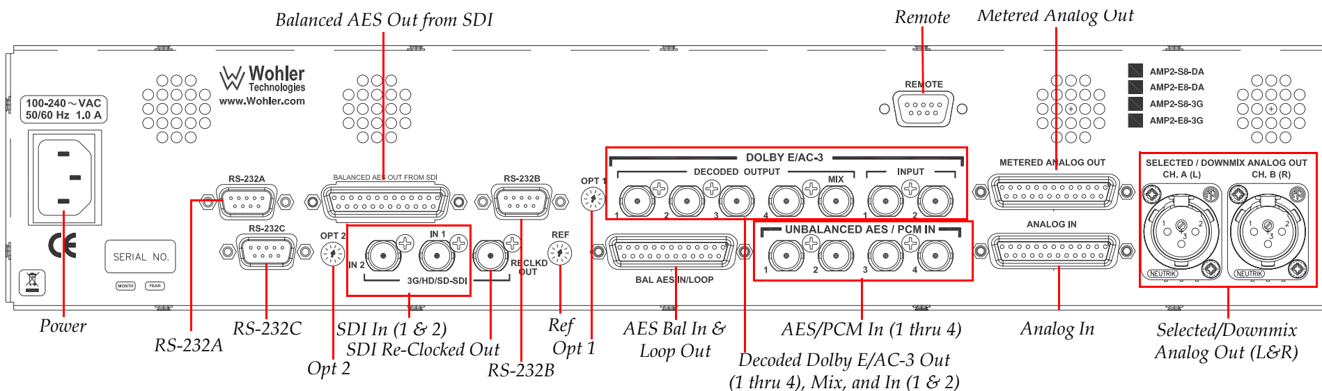
Figure 1–8 The AMP2-E8-MDA-3G Rear Panel
