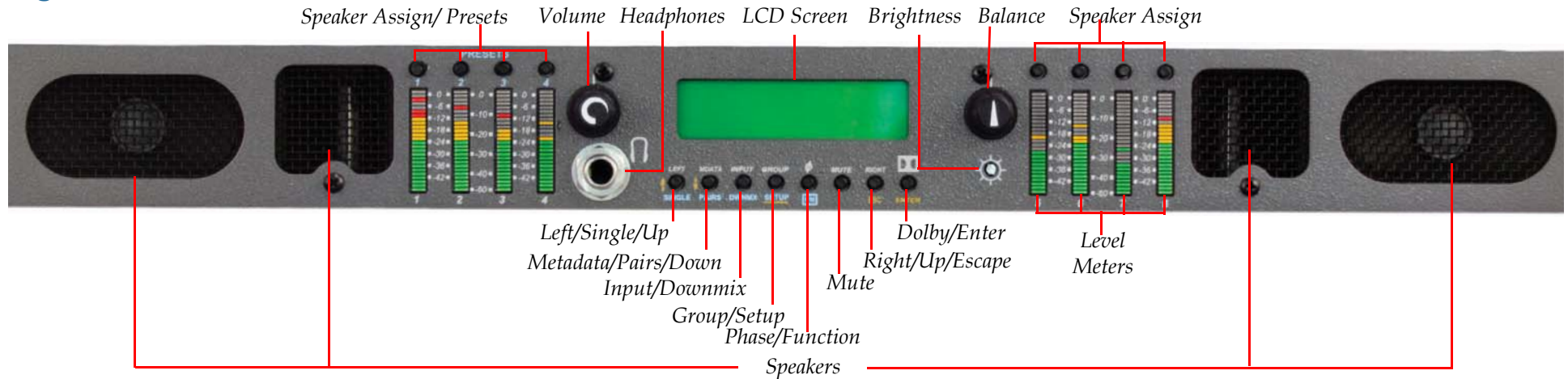
Figure 1–1 The AMP1-E8 Series Front Panel
