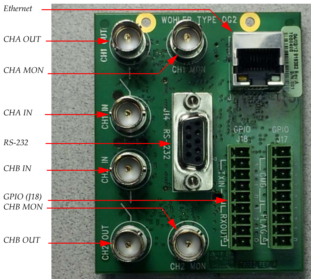
Figure 1-5 OG2 Rear Panel
