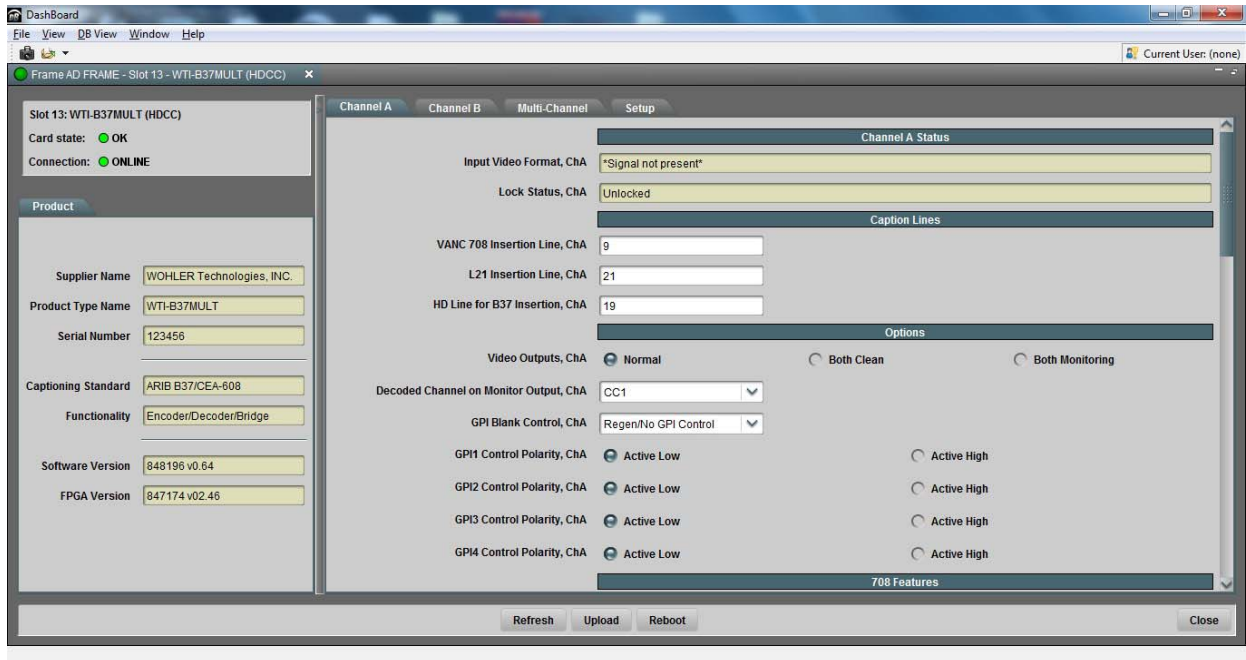
Figure 4–2 DashBoard Main Screen (Top)
