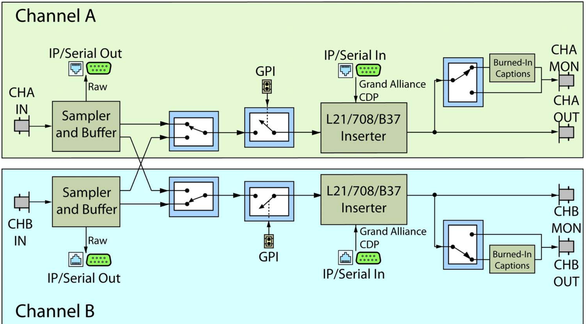
Figure B–2 HDCC Block Diagram
