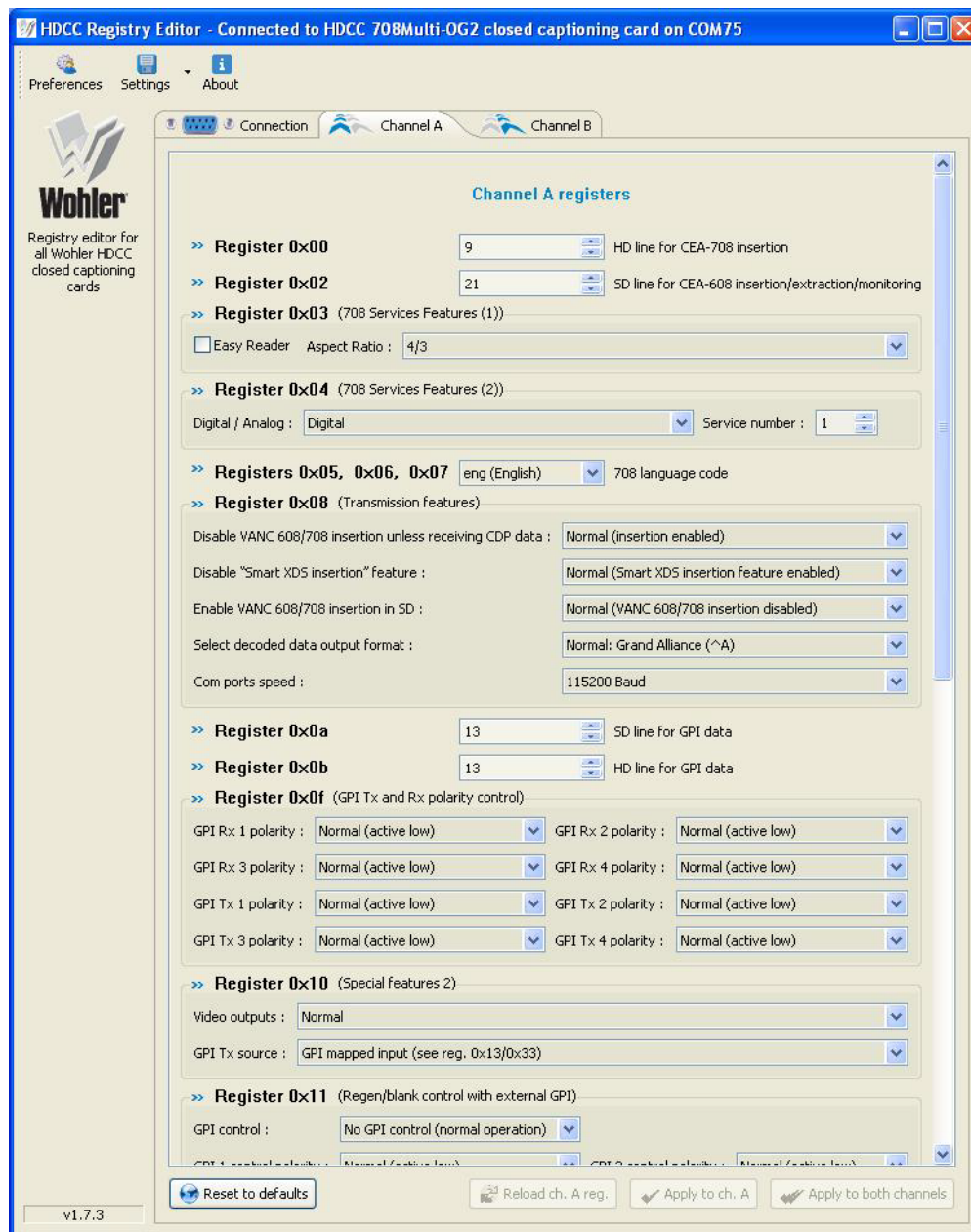
Figure 5–5 Channel A Settings (Bottom)
