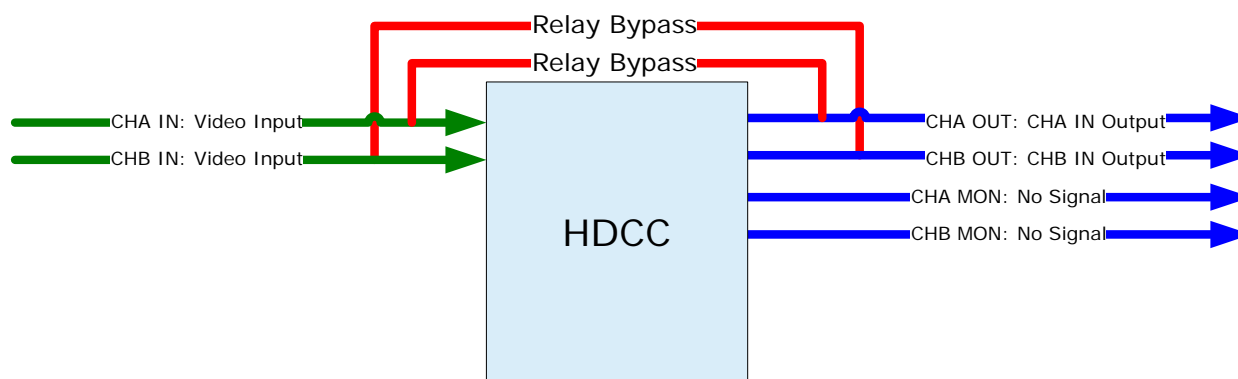
Figure 1–8 Relay Bypass - No Power Condition
