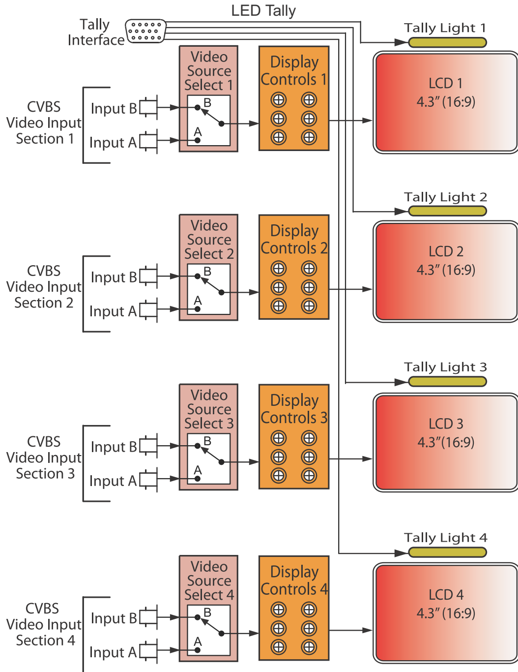
Figure 1–11 RM-2443W-2C Block Diagram
