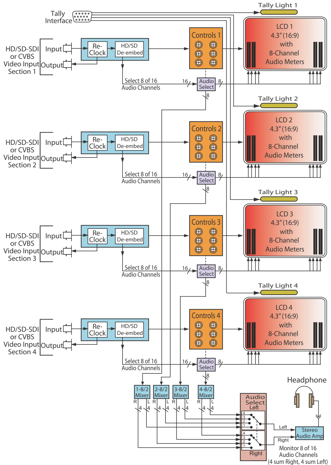
Figure 1–9 RM-2443W-HD Block Diagram
