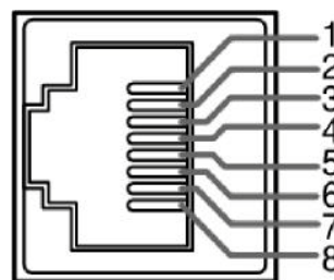
Figure 1–7 RS485 RJ45 Connector Pin Map
