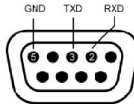
Figure 1–6 DB-9 Connector Pin-Out
