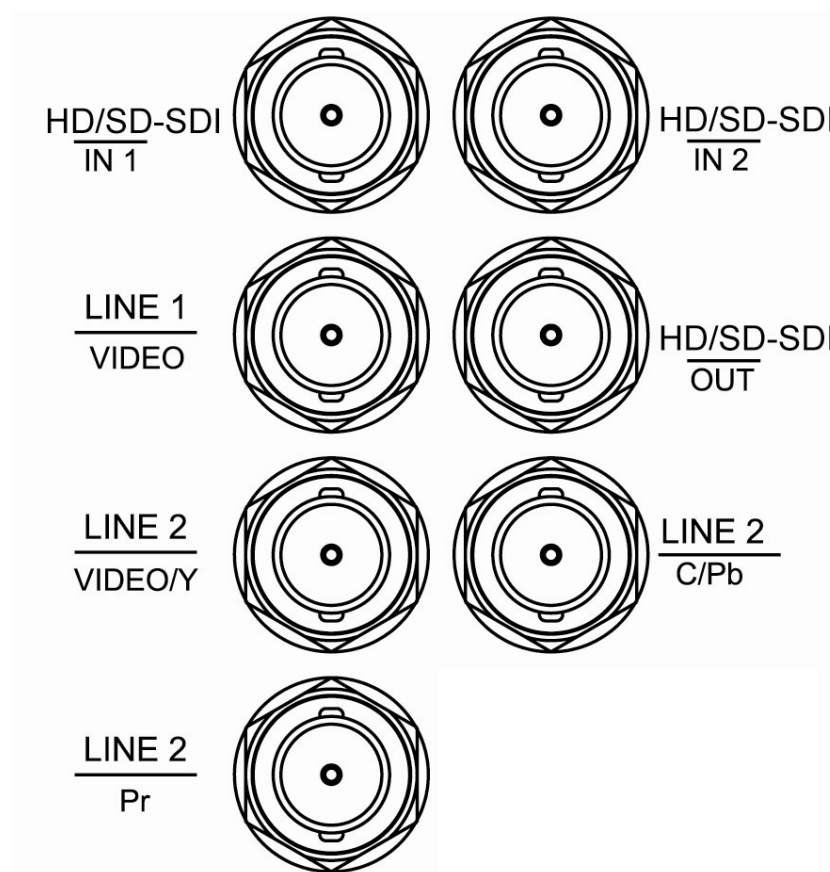
Figure 1–5 BNC Connector Close Up
