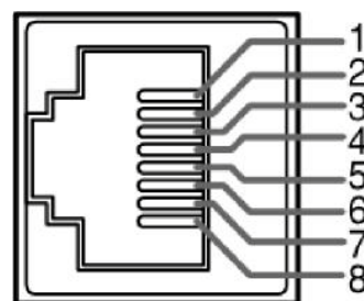
Figure 1-4 GPI/Tally Light RJ45 Connector Pin Map
