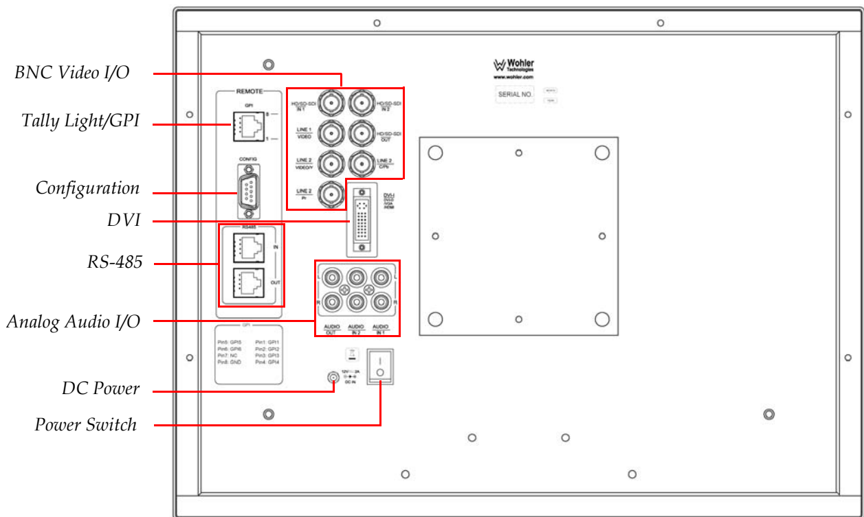
Figure 1-3 RMT-170-HD Rear Panel
