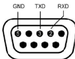
Figure 1–5 DB-9 Connector Pin-Out
