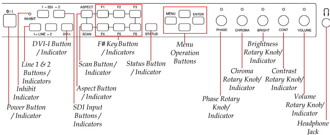
Figure 1–2 Front Panel Controls
