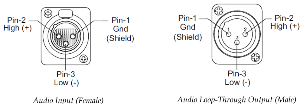
Figure 1–3 Three-Pin XLR Pin-Outs
