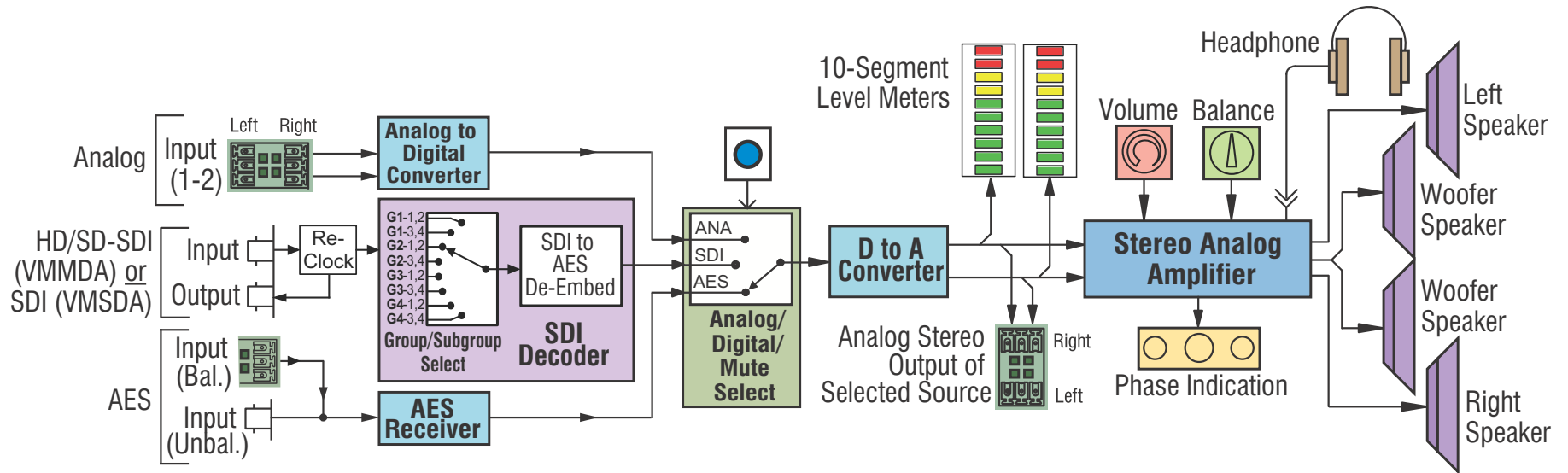
Figure 1–6 VMMDA-1 Block Diagram
