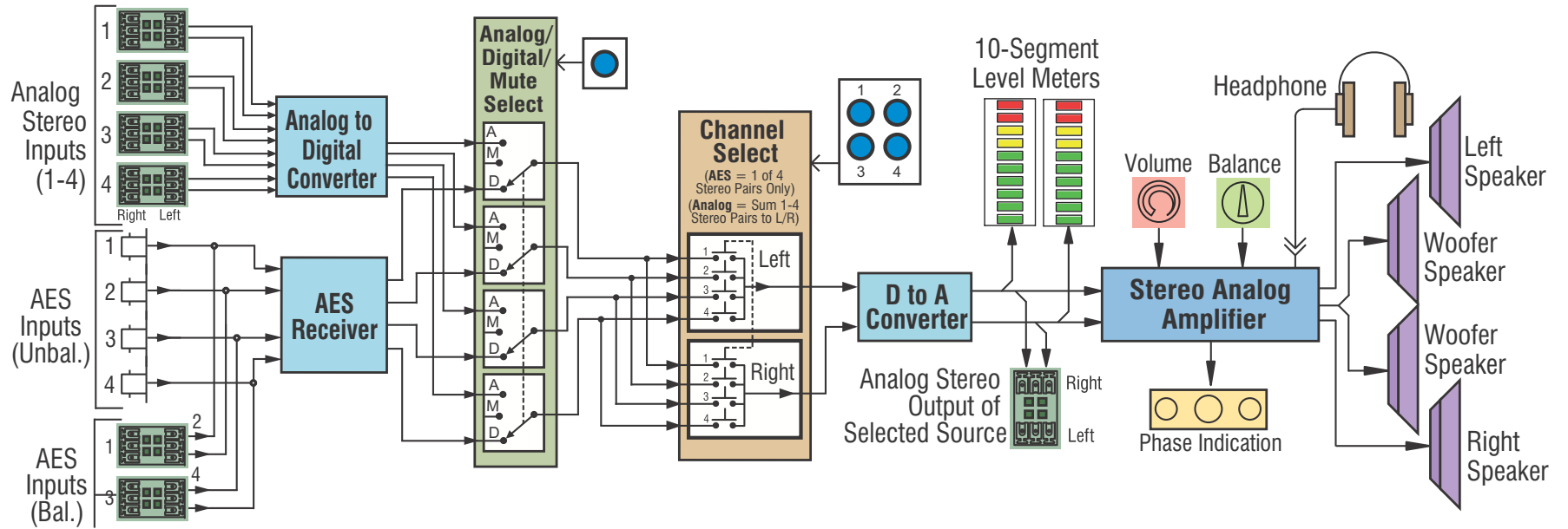
Figure 1–5 VMDA-4 Block Diagram
