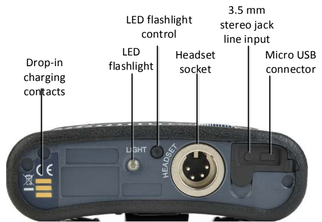
FS II Beltpack connectors
