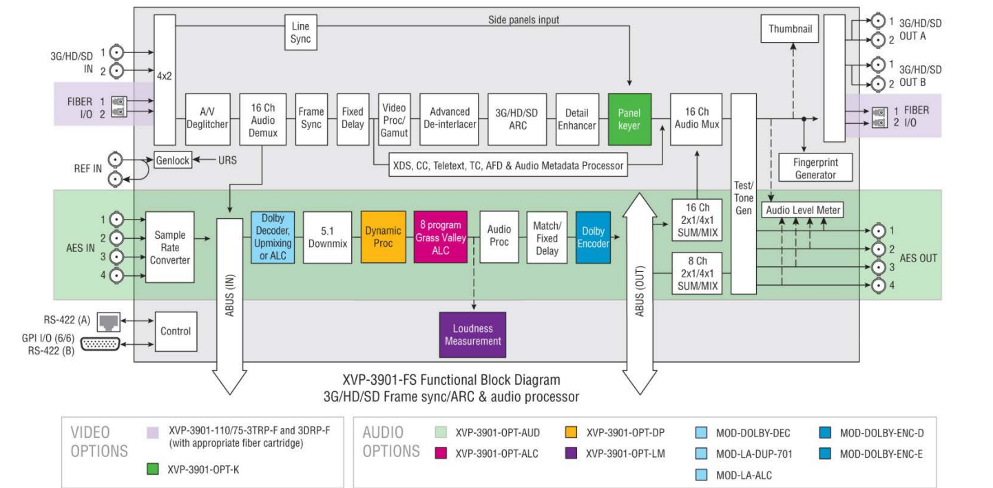
Figure 1.2 Functional block diagram XVP-3901-FS
