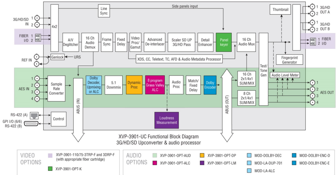
Figure 1.5 Functional block diagram XVP-3901-UC
