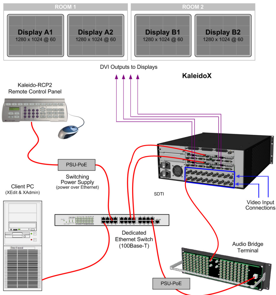
Kaleido-X (4RU) cabling diagram
