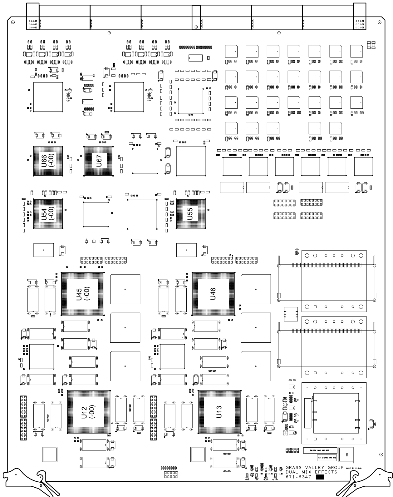
Figure 2. Dual Mix Effects Module Component Layout
