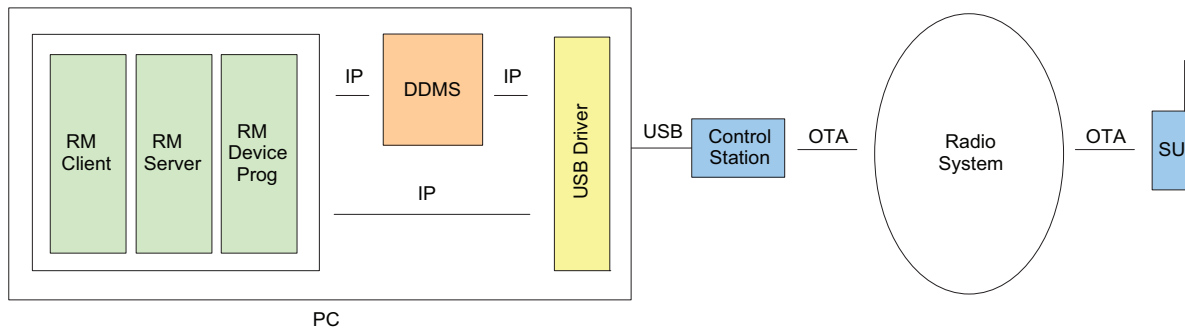
Figure 2-40 Single Channel Non-Remote RM Application with Presence (RM Client, RM Server, and RM Device Programmer Shown)
