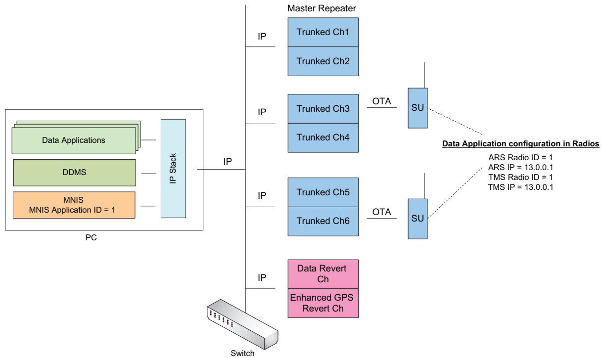
Figure 4-32 Capacity Plus System with MNIS Deployed in the Same LAN as the Repeaters
