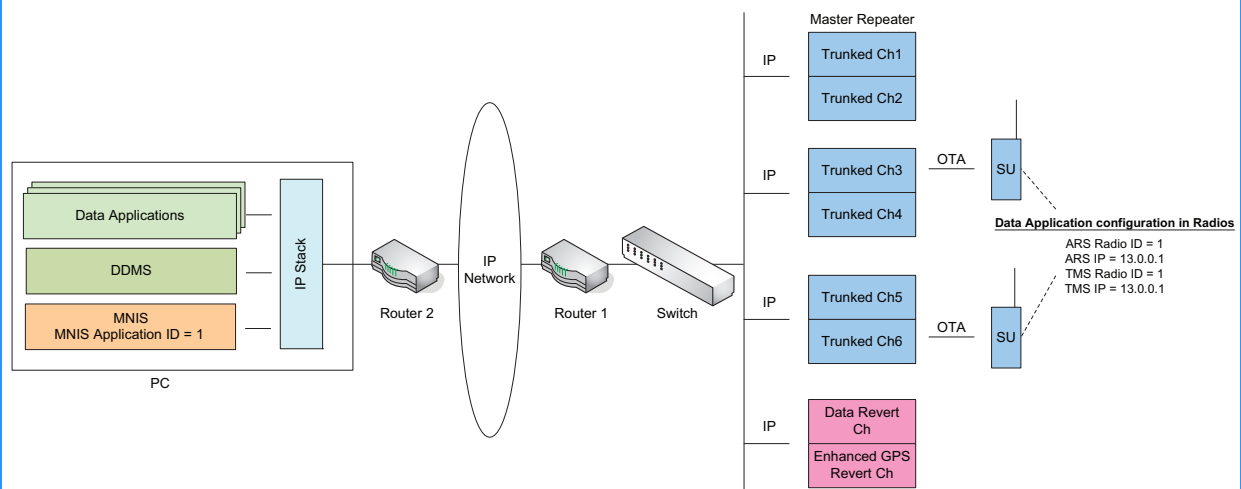
Figure 4-33 Capacity Plus System with MNIS Deployed Remotely
