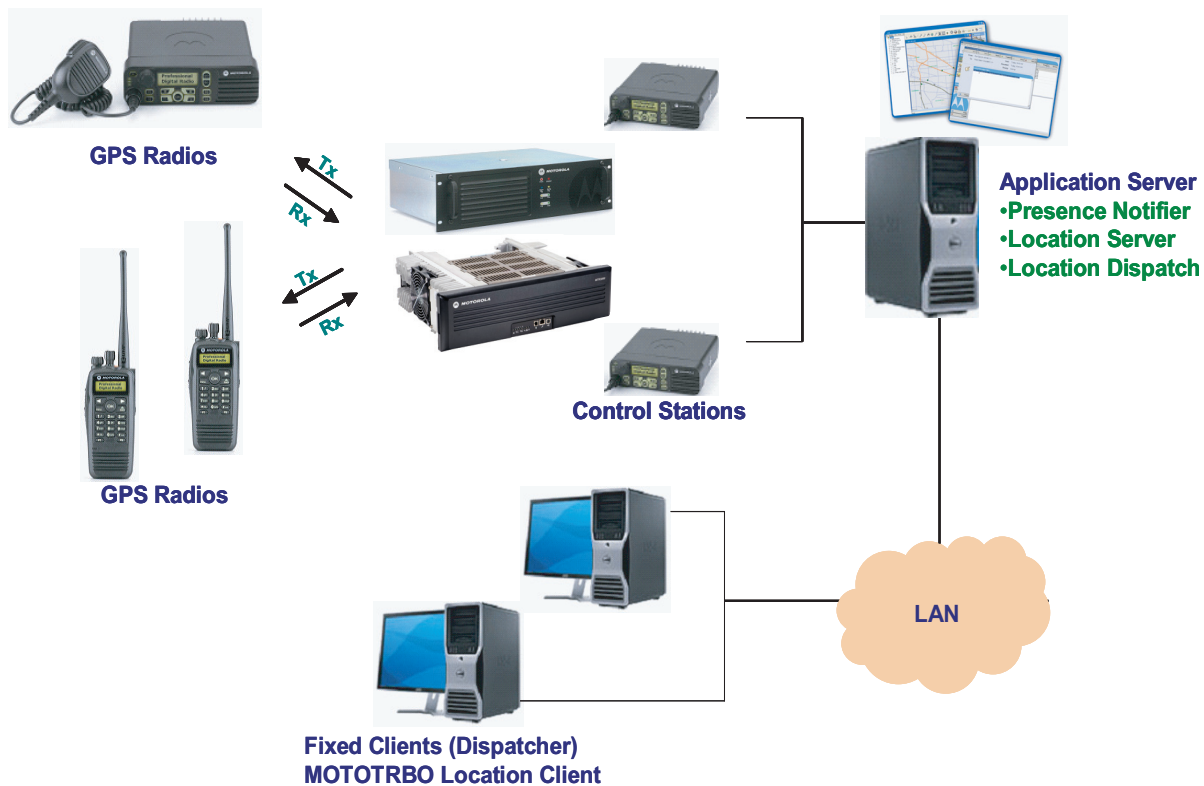
Figure 2-9 Location Services
