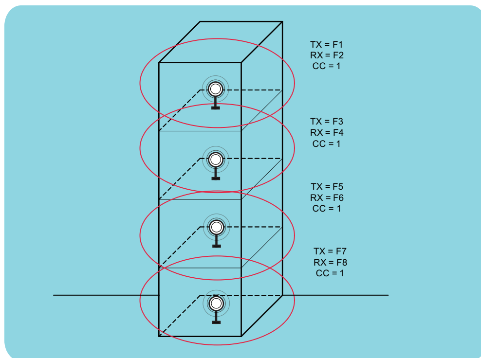
Figure 2-18 Multi-Floor Coverage
