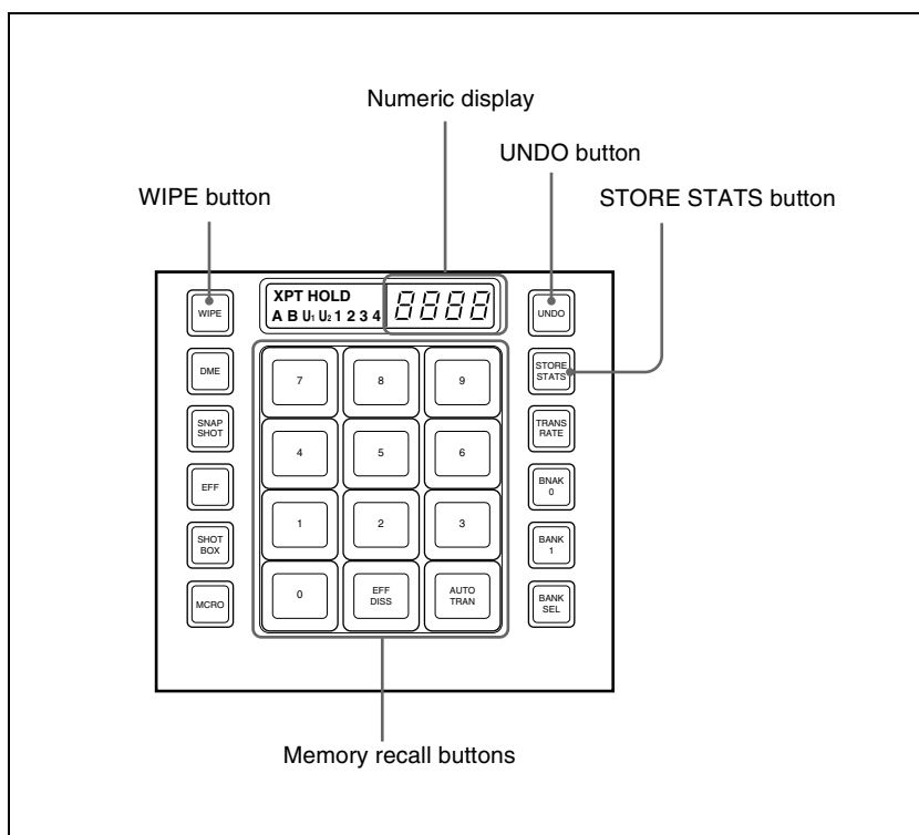
Flexi Pad control block (standard type)
