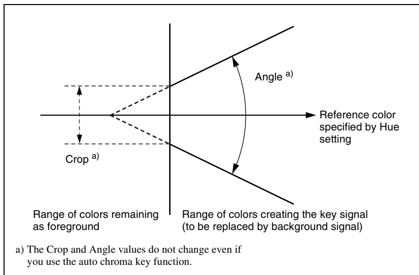
Window adjustment
