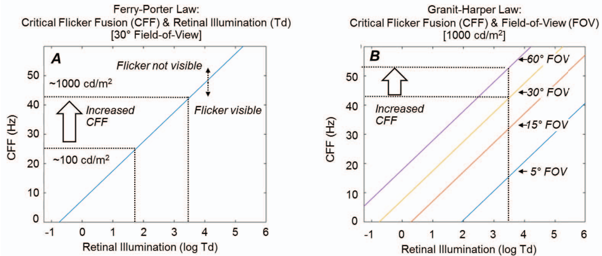
Figure 4. Illustration of the Ferry-Porter law, A , and Granit-Harper law, B . Brighter HDR displays may be expected to make non-smooth motion and flicker more noticeable. The Ferry-Porter law states that the Critical Flicker Fusion (CFF) rate increases with the log of retinal illumination. The Granit-Harper law states the CFF increases with the size of the retinal image. Thus, larger displays subtending wider field-of-view may be expected to make non-smooth motion and flicker more noticeable. (The horizontal axis is in units of log Trolands (log Td). A Troland is a measure of the illumination of the retina and is equal to luminance ( \text{cd/m}^2 ) multiplied by the area of the pupil of the eye. See Table 2.)
