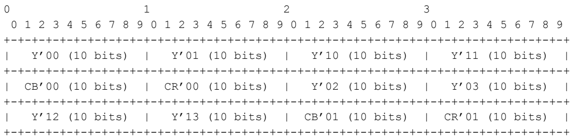
Figure 6 Example of a 4:2:0 10-bit pgroup
