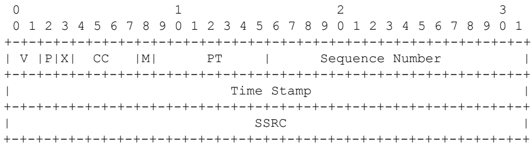
Figure 1 -- RTP Header
