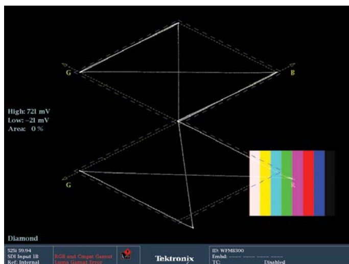
Figure 8. 100% Color Bars with red error.
