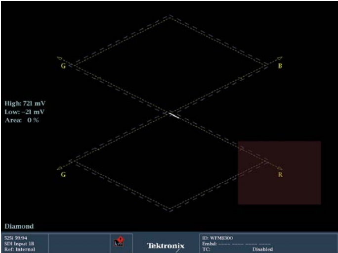
Figure 17. Red balance error on Diamond display.
