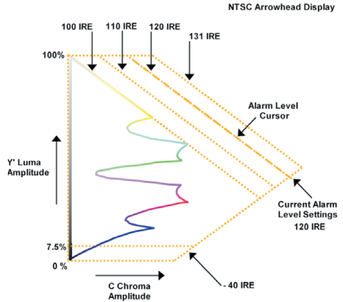
Figure 34. NTSC Arrowhead construction.
