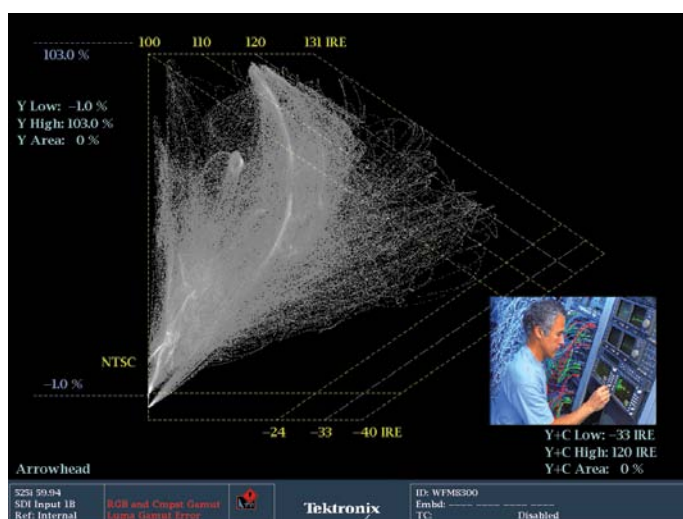
Figure 37. Live video signal monitored with the Arrowhead display showing clear indication of a composite gamut error.
