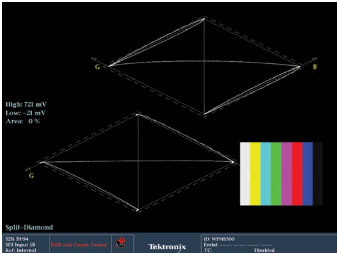
Figure 16. P'b timing error shown on Diamond display.
