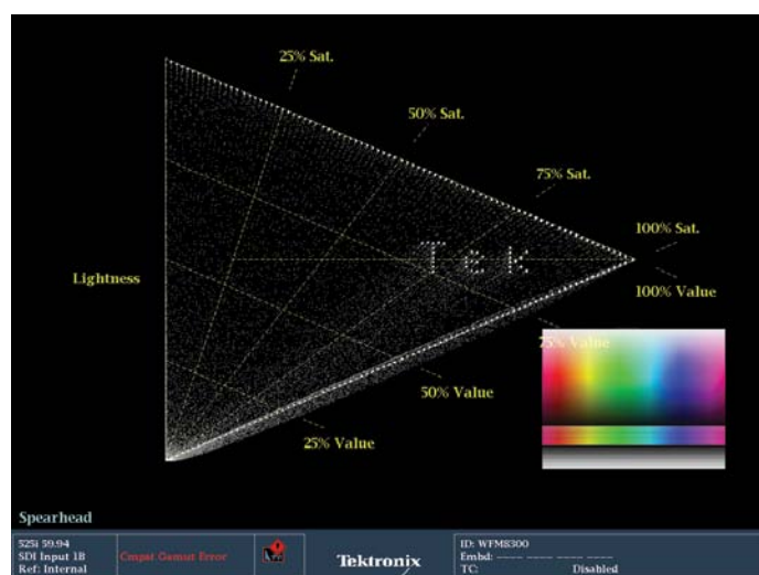
Figure 26. "Rainbow" test pattern on the Spearhead Display.
