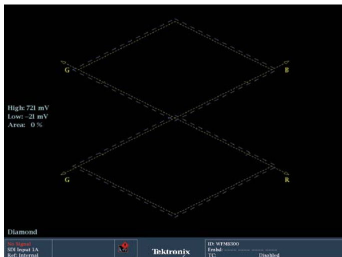
Figure 4. Diamond display graticule.
