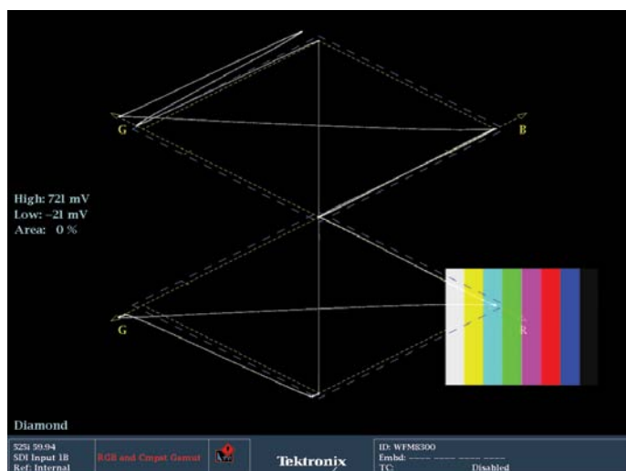
Figure 7. Diamond display using 100% color bars with green amplitude error.
