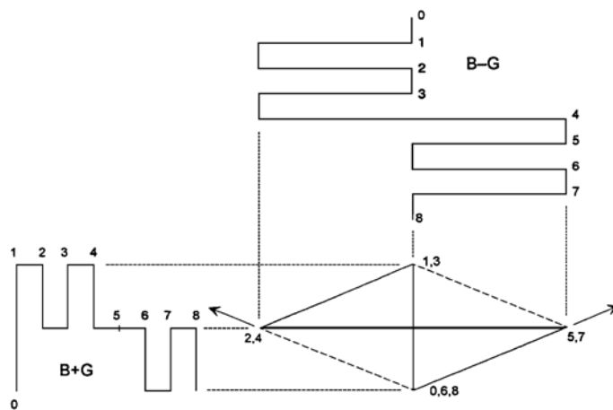
Figure 5. Formation of upper diamond with G' and B' .
