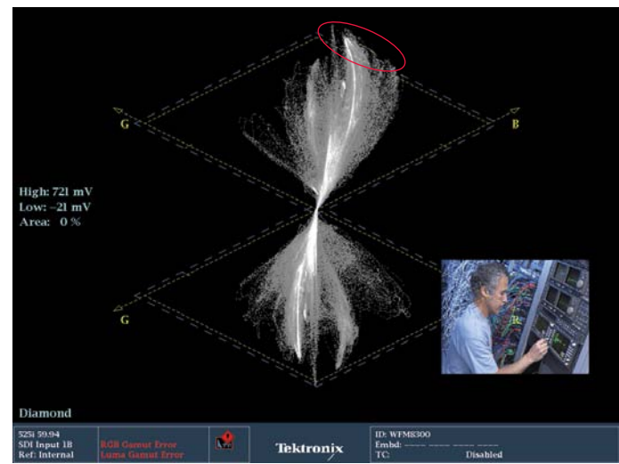
Figure 13. Diamond display with live signal and gamut errors.
