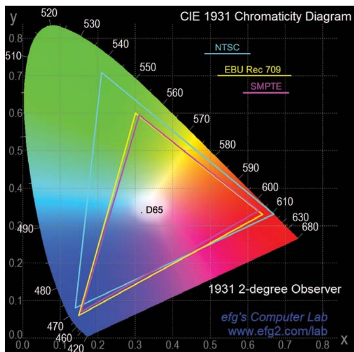
Figure 1. CIE xy Diagram with color coordinates used by NTSC, SMPTE and Rec. 709.
