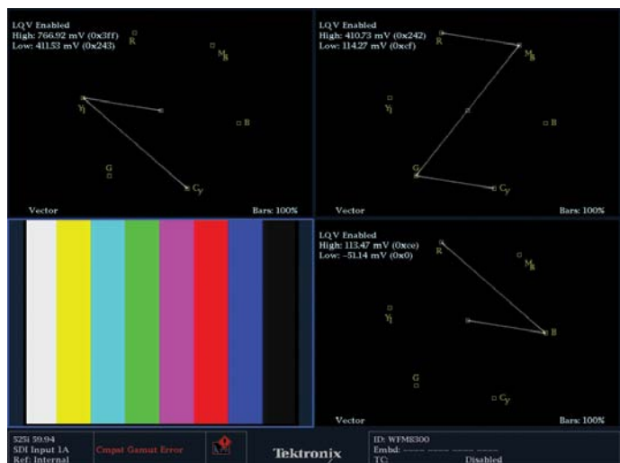
Figure 31. Luminance Qualified Vector display.
