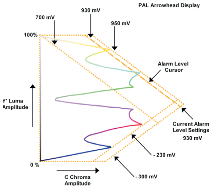
Figure 33. PAL Arrowhead construction.
