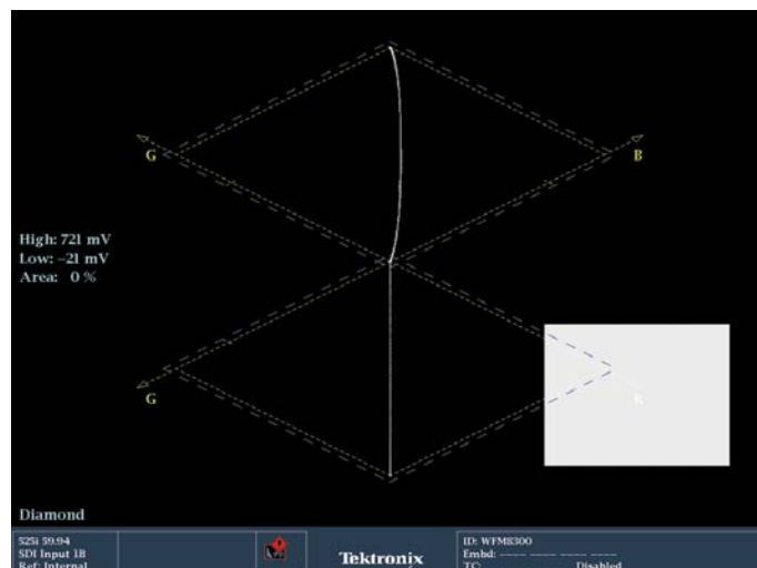
Figure 22. Blue gamma error on Diamond display.
