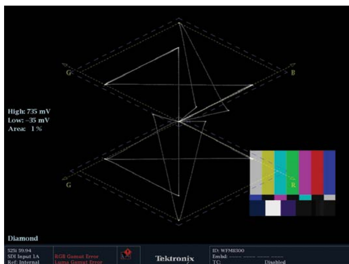
Figure 10. Diamond display using SMPTE Color Bars signal exceeds R'G'B' limits.
