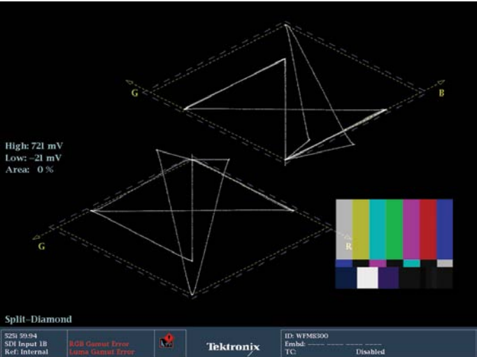
Figure 14. Split Diamond display using SMPTE Color Bars.
