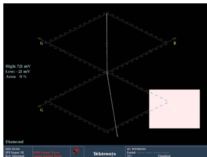
Figure 23. Red gain error on Diamond display.
