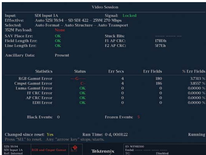
Figure 11. Video Session display, showing RGB and Composite Gamut Errors.
