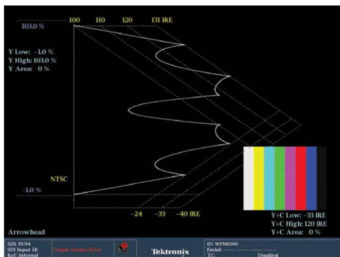
Figure 36. Arrowhead display with 100% Color Bars Signal.
