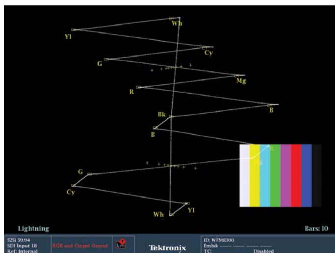
Figure 41. P'b gain error on Lightning display.
