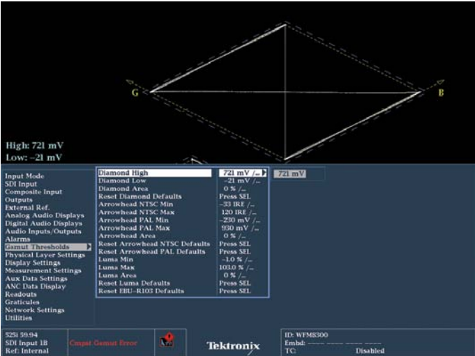
Figure 15. Configuring gamut limits on the WFM8300.
