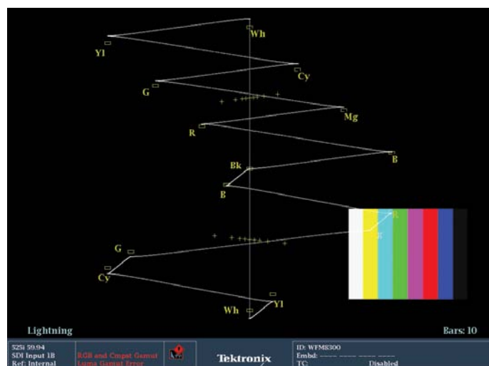
Figure 40. Luma gain error on Lightning display.
