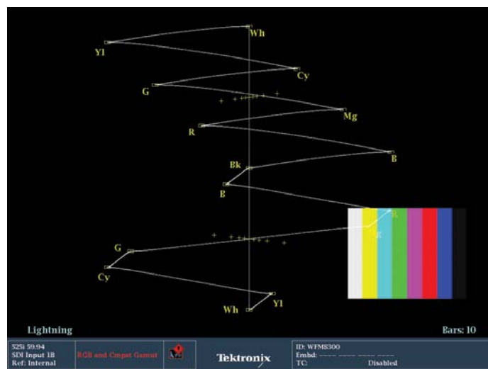
Figure 42. P'b advanced timing error on Lightning display.
