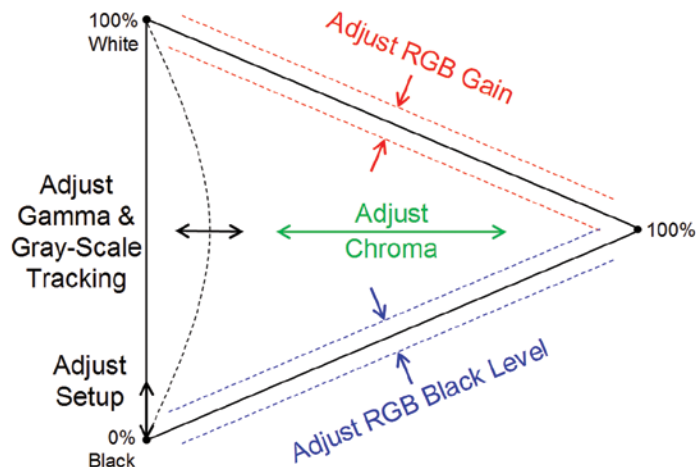
Figure 25. Using the Spearhead display for color correction.
