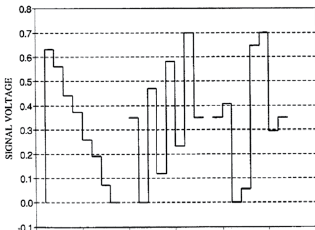
Figure 2B. Distorted but legal color-difference signal translates to an invalid R'G'B' signal.
