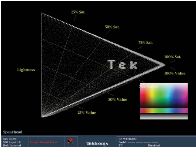
Figure 27. Hue error on the rainbow test pattern.
