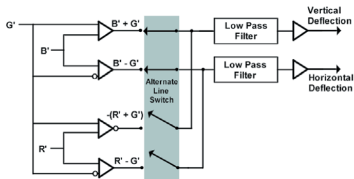
Figure 6. Low pass filter reduces high frequency transients that exceed gamut limits.
