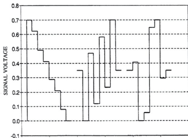
Figure 2A. Legal and valid color-difference signal translates to a legal R'G'B' signal.
