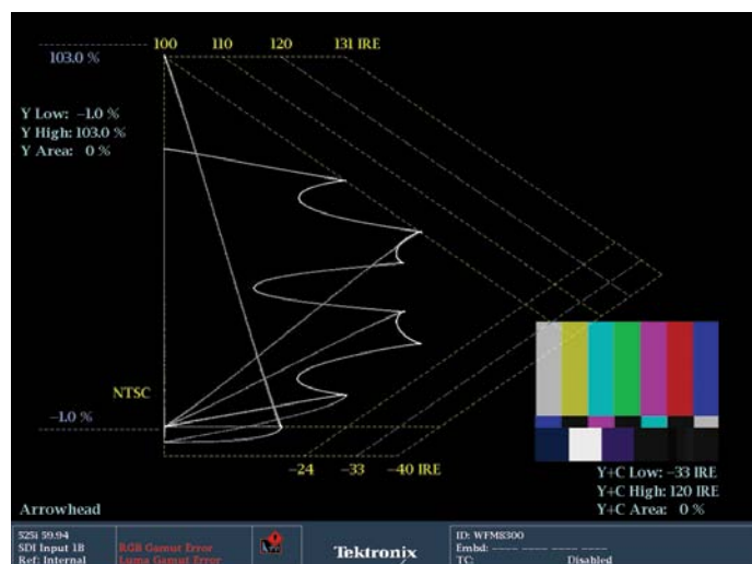
Figure 35. Arrowhead display showing SMPTE Color Bars.
