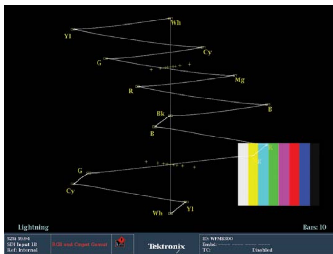
Figure 43. P'b delayed timing error on Lightning display.
