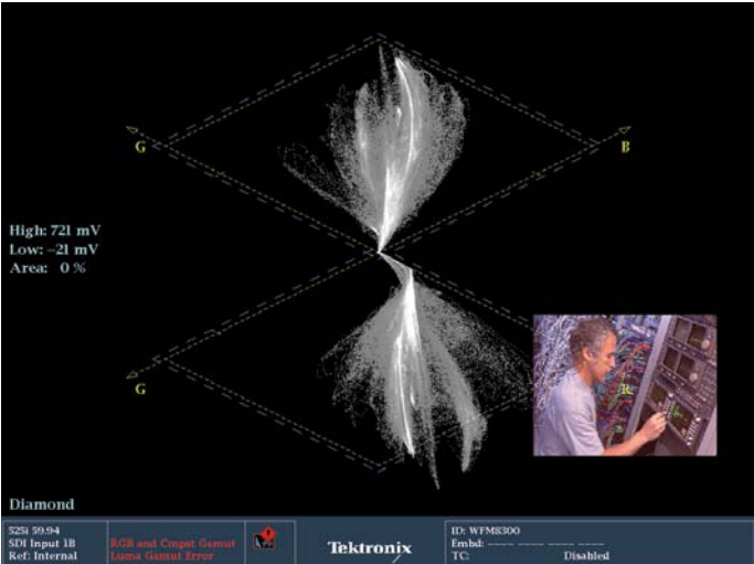
Figure 18. Live signal with red balance error.
