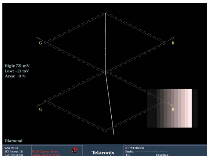
Figure 9. 10 step staircase with red imbalance.
