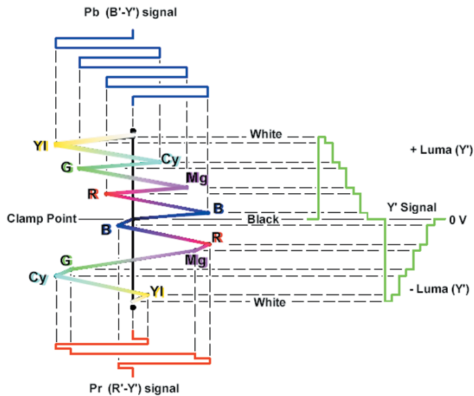
Figure 38. Construction of Lightning display.
