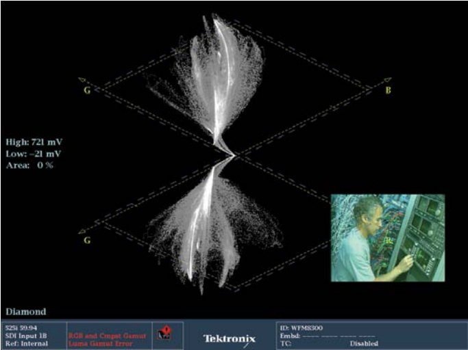
Figure 20. Live signal with green balance error.
