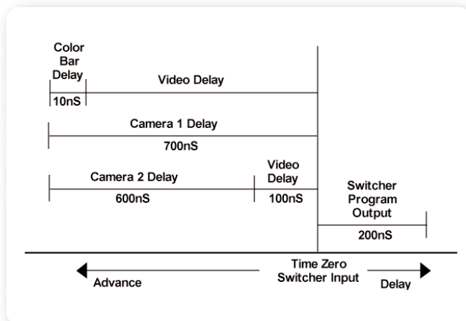
► Figure 11. System timing through the studio.
