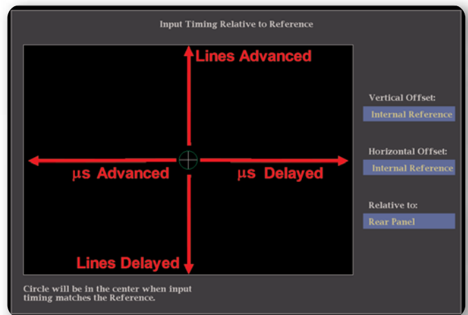
► Figure 18. Interpretation of Timing Display.
