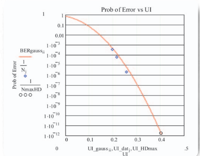
► Figure 33. BER vs. peak-to-peak jitter amplitude for a typical video signal.
