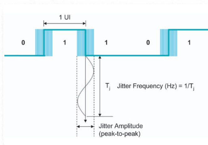
► Figure 2. SDI signal with sinusoidal edge variation (ideal positions shown in darker lines).
