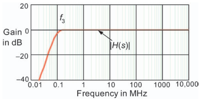
► Figure 28. Frequency response of total transfer function H(s) for Equivalent-Eye Method.
