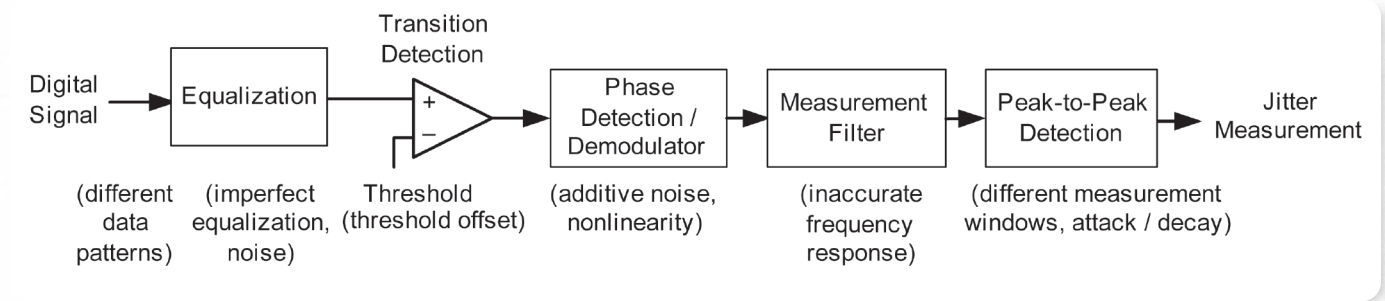
► Figure 16. The functions involved in jitter measurement (Causes of measurement discrepancies are indicated in parentheses).
