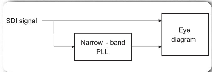
► Figure 20. Equivalent-time Eye method.
