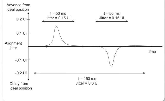
► Figure 15. Peak-to-peak measurement value depends on measurement time.
