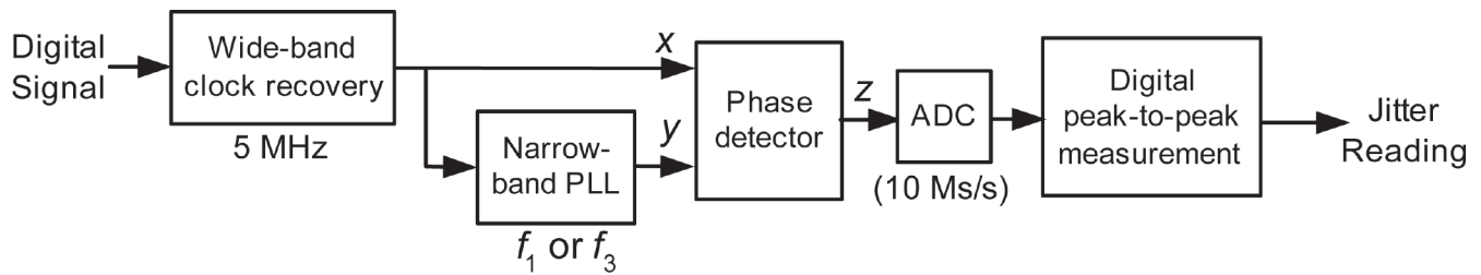
► Figure 34. Phase Demodulation method in WFM700M.
