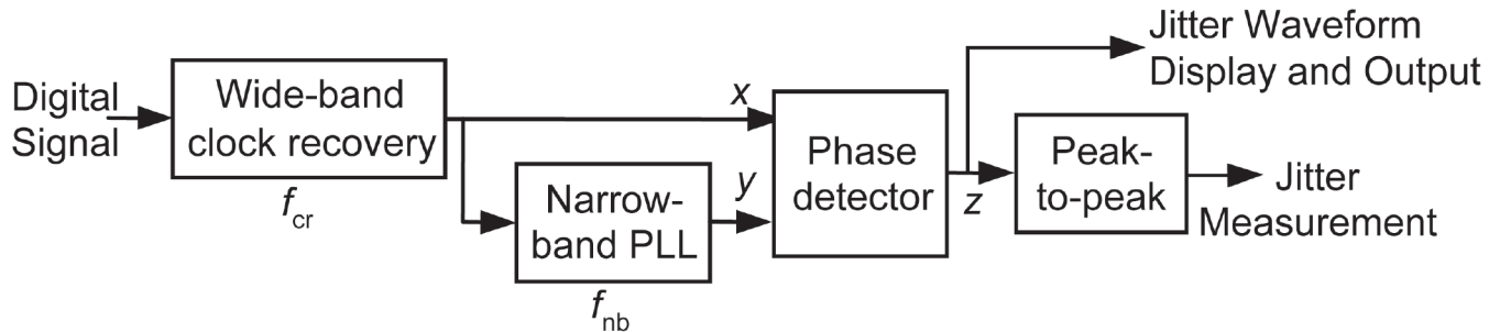
► Figure 22. Phase Demodulation method.
