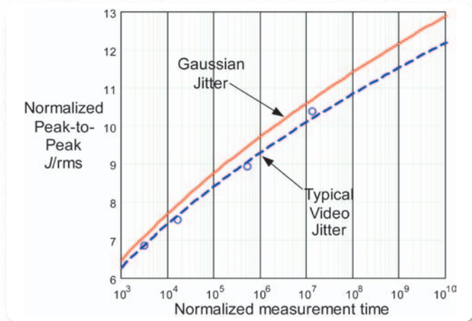
► Figure 29. Effect of normalized measurement time on measured peak-to-peak jitter amplitude ( J/rms ).
