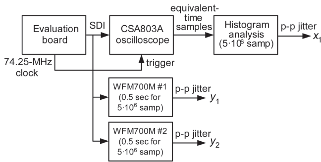
► Figure A-1. Test setup for comparing jitter measurement methods.
