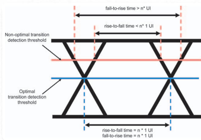
► Figure 18. Non-optimal decision threshold introduces duty cycle dependent jitter.
