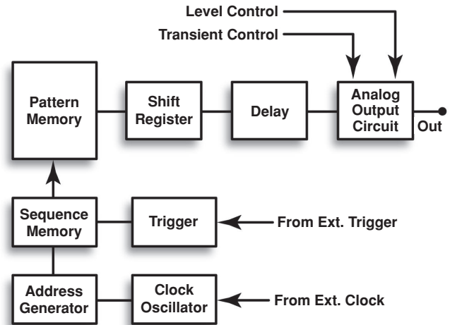
Figure 41. The architecture of a PPG or DTG (simplified).
