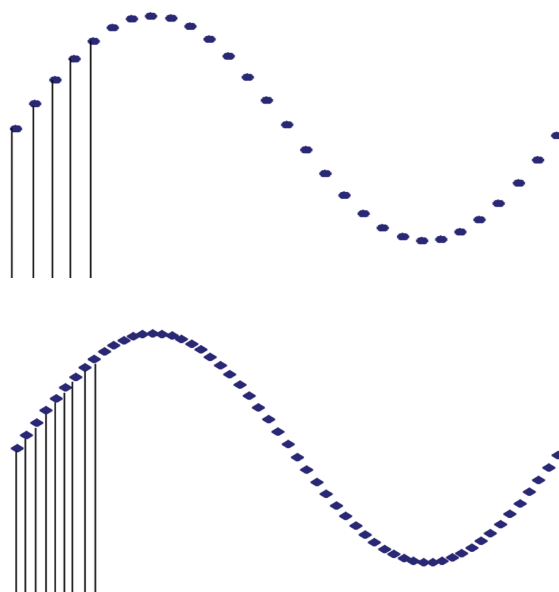
Figure 26. (Top) Low horizontal resolution; (Bottom) High horizontal resolution. Horizontal, or timing, resolution refers to the minimum increment of time by which an edge, cycle time, or pulse width can be changed.
