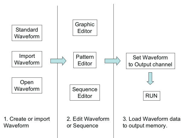
Figure 35. Basic steps used to create waveforms using an AWG.
