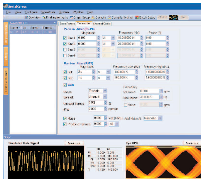
Figure 38. Impairment creation made easy with SerialXpress.
