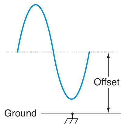
Figure 6. The offset voltage describes the DC component of a signal containing both AC and DC values.
