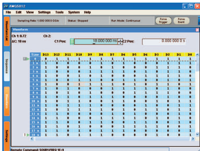
Figure 30. Parallel digital outputs.
