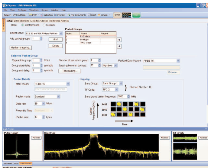
Figure 40. Complex UWB waveforms are easily created using RFXpress.
