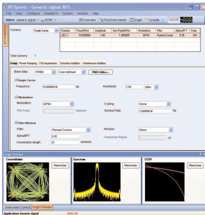
Figure 39. Single carrier RF waveform created by RFXpress.
