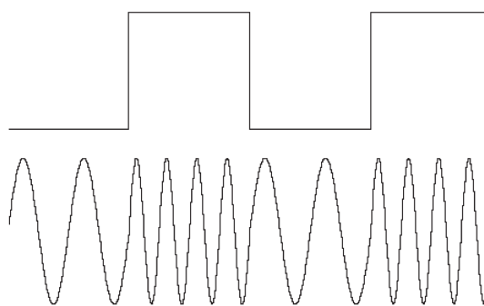
Figure 13. Frequency-shift keying (FSK) Modulation.
