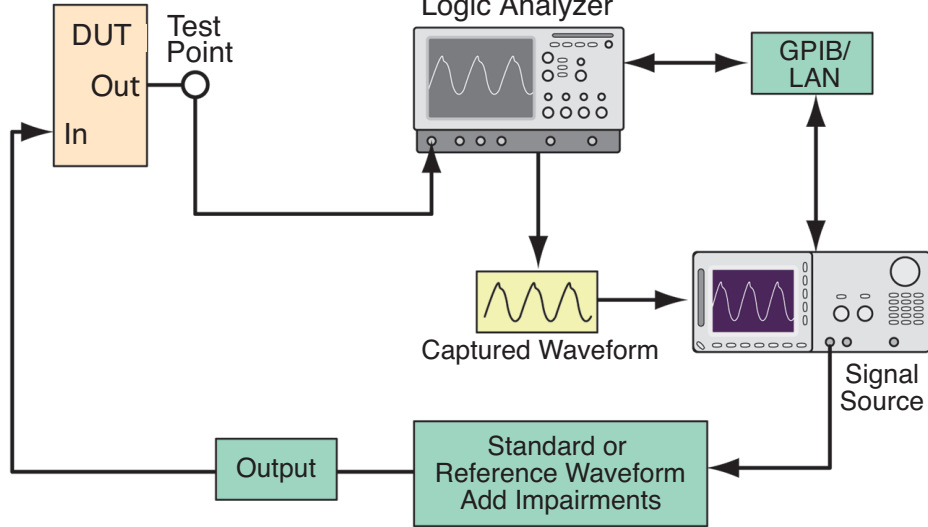
Figure 3. Signal generators can use standard, user-created or captured waveforms, adding impairments where necessary for special test applications.
