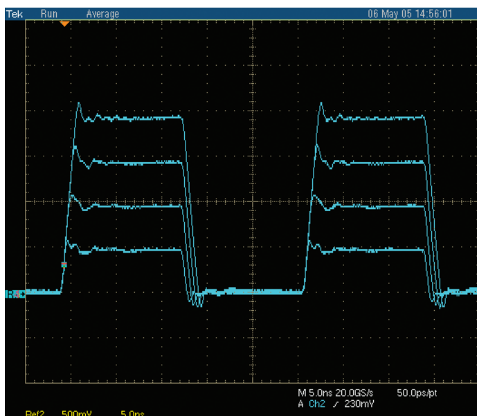
Figure 43. Programmed voltage variations on a pattern generator's output signal applies a single voltage level throughout the pattern.
