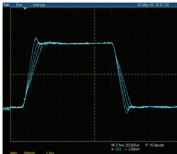
Figure 44. Programmed rise time variations on a pattern generator's output signal.
