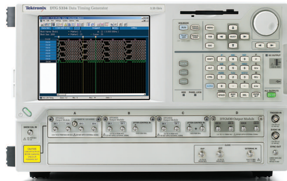
Figure 48. A high-performance logic source: the Tektronix DTG5334 Data Timing Generator.
