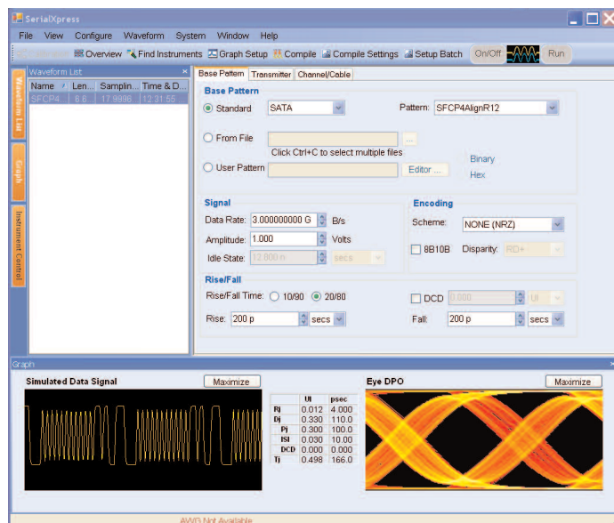
Figure 37. Standard SATA waveform with pre-emphasis.
