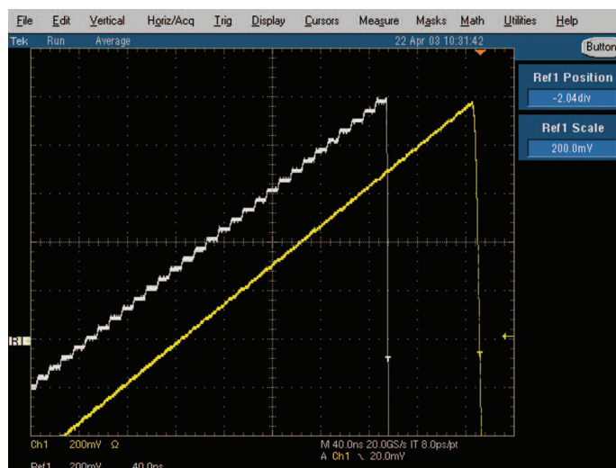
Figure 31. Filtering, before and after. Reference 1 (Top) waveform is an unfiltered ramp waveform, while Channel 1 (Bottom) waveform is a filtered ramp waveform.
