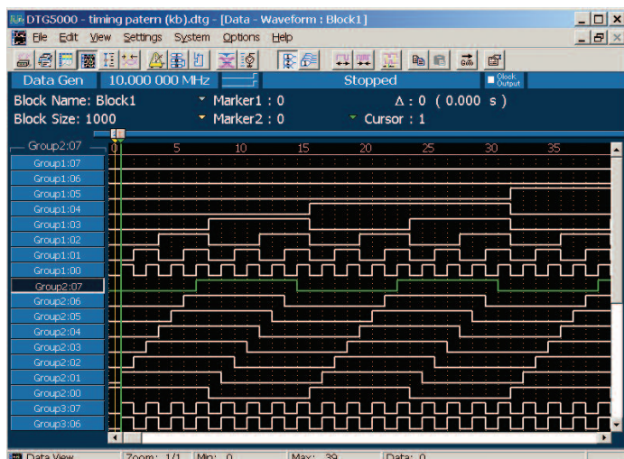
Figure 46. Multi-channel DTG's bus timing display.
