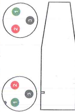
XLR MALE CONNECTOR (outside view) (solder-side view)
