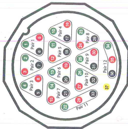
DT-12 FEMALE CONNECTOR
