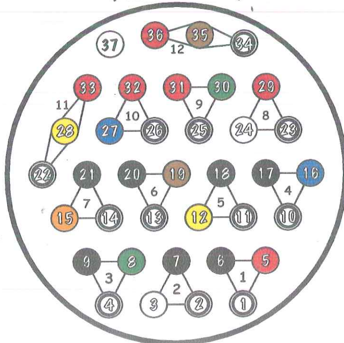
MALE (SOLDER-SIDE VIEW)
