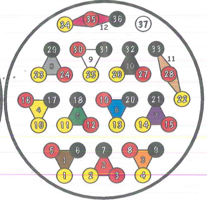
FEMALE (SOLDER-SIDE VIEW)
