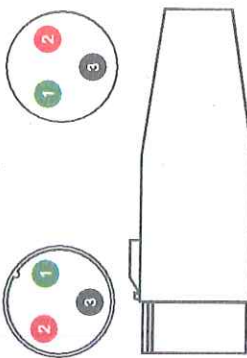
XLR FEMALE CONNECTOR (outside view) (solder-side view)
