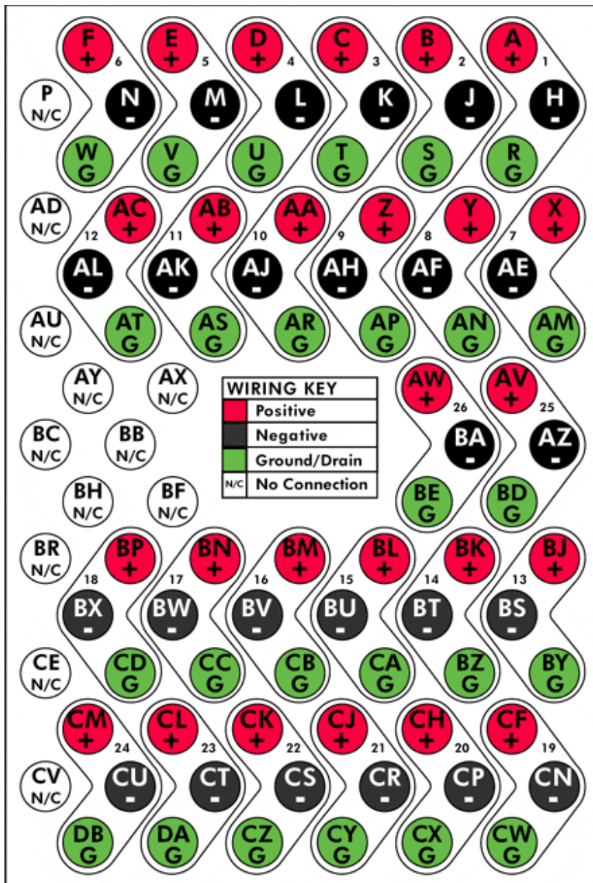
REAR VIEW OF FEMALE ELCO 90 PIN CONNECTOR FOR ADC PRO-PATCH
